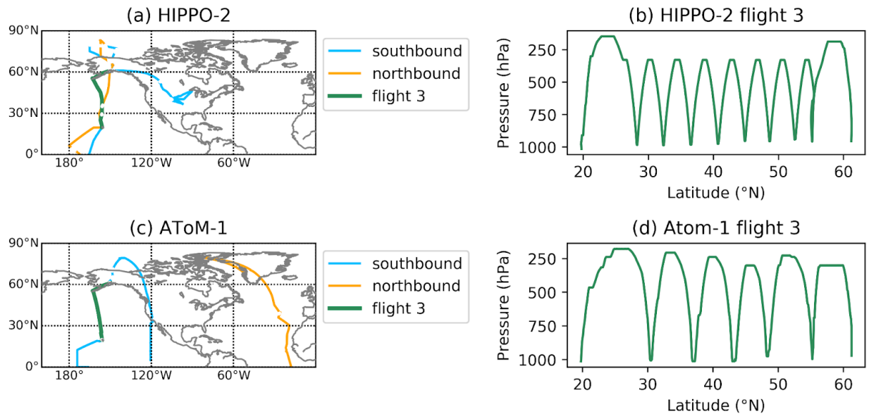
Figure 1 Flight paths for (a) HIPPO-2, which flew over the remote Pacific in November 2009, and (c) ATom-1, which flew over the Pacific and Atlantic in August 2016. All other campaigns followed similar flight paths. Flight path with continuous vertical profiling for flight 3, which flew from Anchorage, AK to Kona, HI for (b) HIPPO-2 and (d) ATom-1. All other flights flew a similar path.
