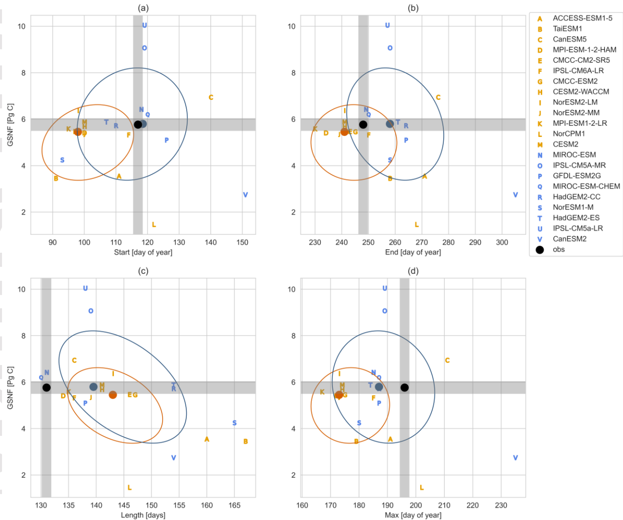
Figure 5 GSNF plotted against the (a) start of the season, defined to be the first day when the seasonal component of atmospheric CO 2 is decreasing (seasonal component of flux changes from positive to negative), (b) end of the season, defined to be the last day when the seasonal component of atmospheric CO 2 is decreasing (seasonal component of flux changes from negative to positive), (c) length of the season, and (d) max of season, defined to be the day when flux is most negative. The black point is the number inferred from the observations with the gray lines showing uncertainty. CMIP5 models are shown in blue and CMIP6 models are shown in orange. The blue and orange points are the multi-model mean for the CMIP5 and CMIP6 ensembles respectively. The surrounding ellipses show the covariance to one standard deviation. Only models where GPP, RH, and NPP output was available are included.
