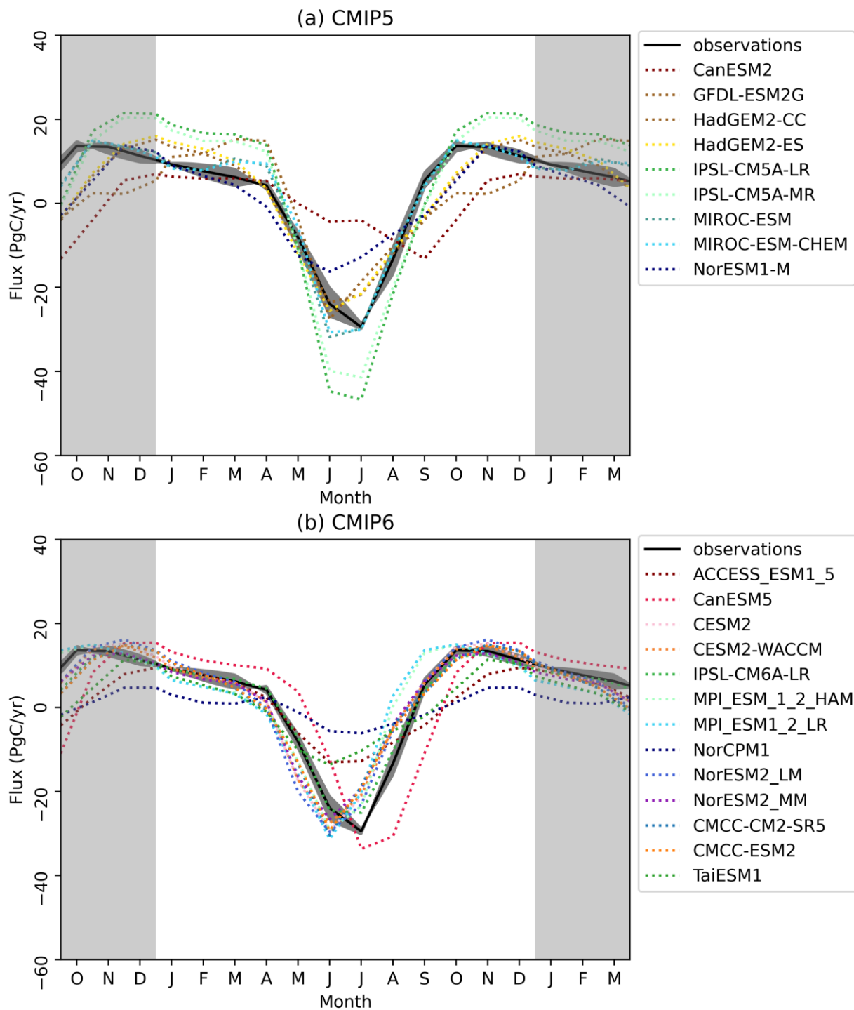
Figure 4 Corrected flux estimated from the HIPPO and ATom campaigns in comparison to area-weighted average NBP in the same domain from the (a) CMIP5 and (b) CMIP6 models. The bias corrected observation error is the standard deviation between correction using the three different inverse models. While the spread in magnitude and timing of the
