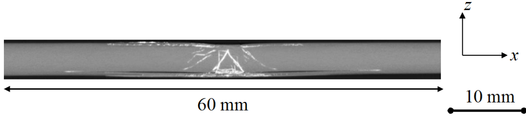
Figure 1 Edge-on \mu CT slice of an impacted [0/90/0/90_9]_s laminate .
