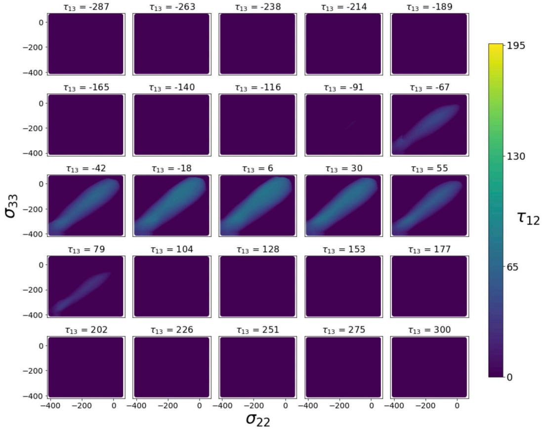
Figure 17 Failure envelope generated by the NN Classification model for E-Glass/LY556 over \tau_{13} values.
