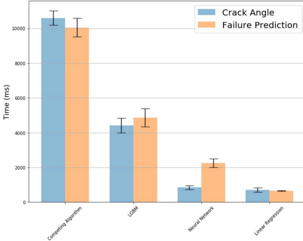
Figure 26 Performance comparison between different model types for 3D stress state.
