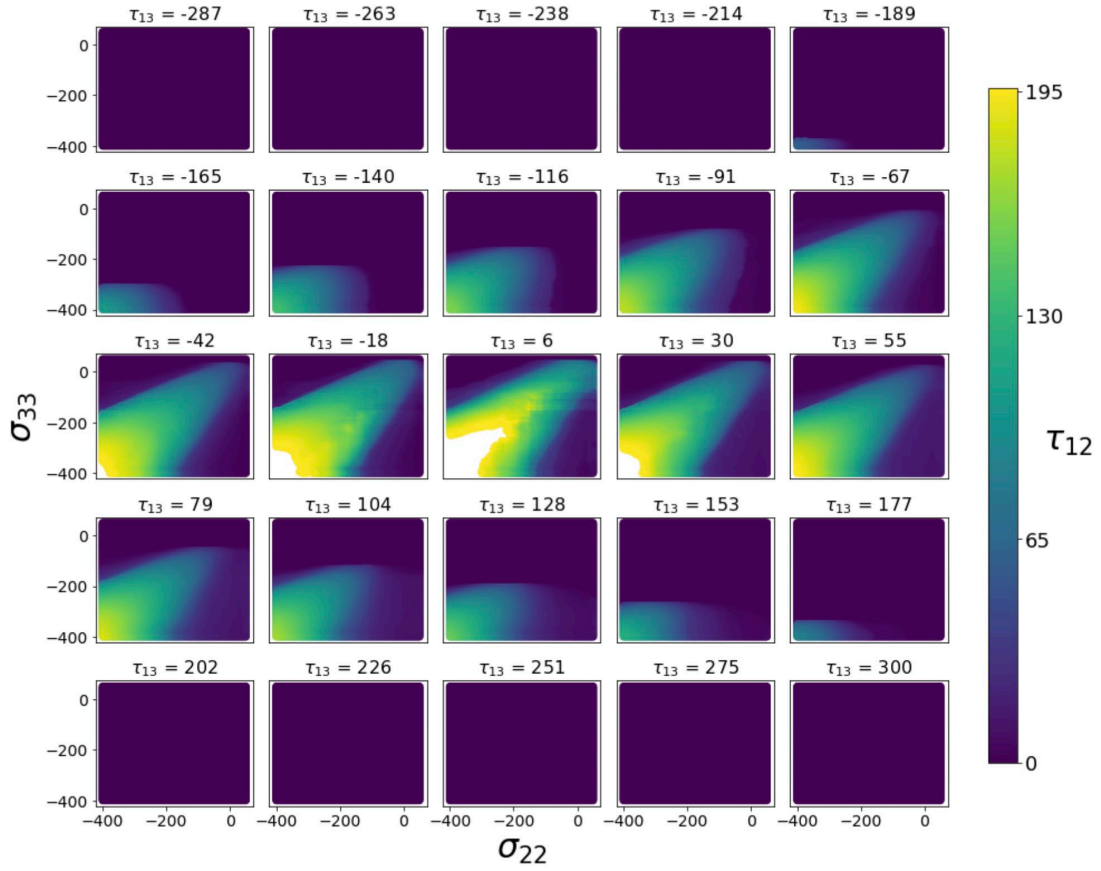
Figure 15 Failure envelope generated by the LGBM Classification model for E-Glass/LY556 over \tau_{13} values.
