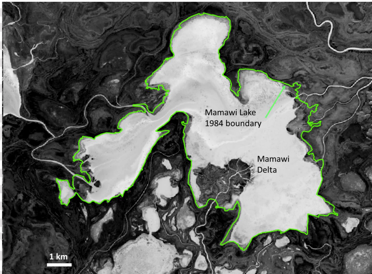
Figure S9. Mamawi Lake extent in 2019. Green lines show its boundary in 1984. The infilling is mainly from the growth of the Mamawi Delta. However, sediment is also delivered into the lake from the east and west sides. Using the same method described in section 3.3, we estimate that the sediment accretion rate for the Mamawi Lake is 0.71 \text{ km}^2 \text{ yr}^{-1} during 2003-2019. With a 91 \text{ km}^2 lake area in 2019, and known shallow bathymetry, Mamawi Lake, excluding central channels, could be completely infilled in \sim 130 years.
