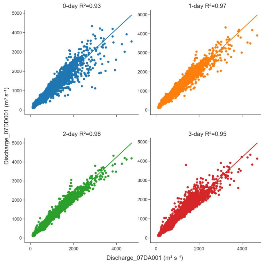
Figure S2. Discharge relationship between upstream 07DA001 and downstream 07DD001. A 2-day travel time from 07DA001 to 07DD001 was chosen as optimal based on the best R-squared value.
