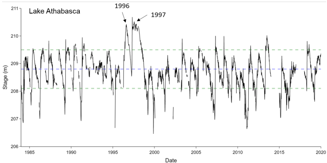
Figure S7. River stage data for the Athabasca Lake (07MD001) between 1984 and 2020. The blue and green dashed lines are mean stage and standard deviation, respectively. The highest stage occurred in 1996 and 1997.
