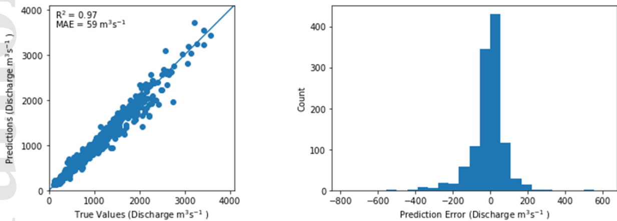
Figure S3. R-square value and mean absolute error ( \text{MAE} = 59 \text{ m}^3 \text{s}^{-1} ) between observed values and predicted values at 07DD001 (Left). Error distribution for predicted discharge at 07DD001 (Right).
