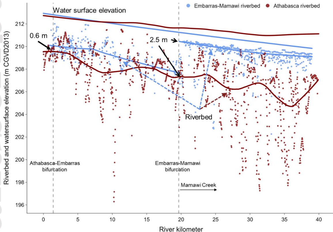
Figure 10. Longitudinal water surface elevation (WSE) and riverbed elevation along the Athabasca River and the Embarras-Mamawi channel downstream of the two rivers' bifurcations. Regression lines are locally weighted scatterplot smoothing lines (LOWESS). At the Athabasca-Embarras bifurcation, the Embarras riverbed is ~0.6 m higher than the Athabasca riverbed. At the Embarras-Mamawi bifurcation, the Mamawi Creek bed is ~2.5 m higher than the Embarras riverbed.
