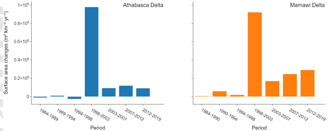
Figure 4. Discharge-normalized surface area change rate ( \text{m}^2 \text{ km}^{-3} \text{ yr}^{-1} ) of the Athabasca River delta (left) and Mamawi Creek delta (right) during seven time periods between 1984 and 2019. Areal changes are mapped from Landsat imagery; discharges are from ECCC gauging stations (07KF003 and 07MD001).
