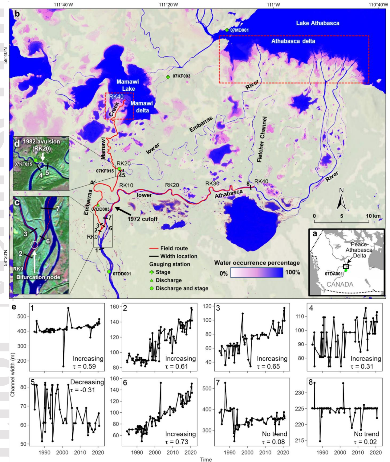
Figure 1. a) The Peace-Athabasca River Delta is located in northeastern Alberta, Canada. b) The Embarras River is a distributary of the Athabasca River that flows east into Lake Athabasca, but has diverted a growing share of Athabasca mainstem discharge northward into Mamawi Lake following its partial avulsion into Mamawi Creek in 1982. This developing Embarras-Mamawi (EM) channel thus represents a potential slow avulsion course for the Athabasca River and is the
