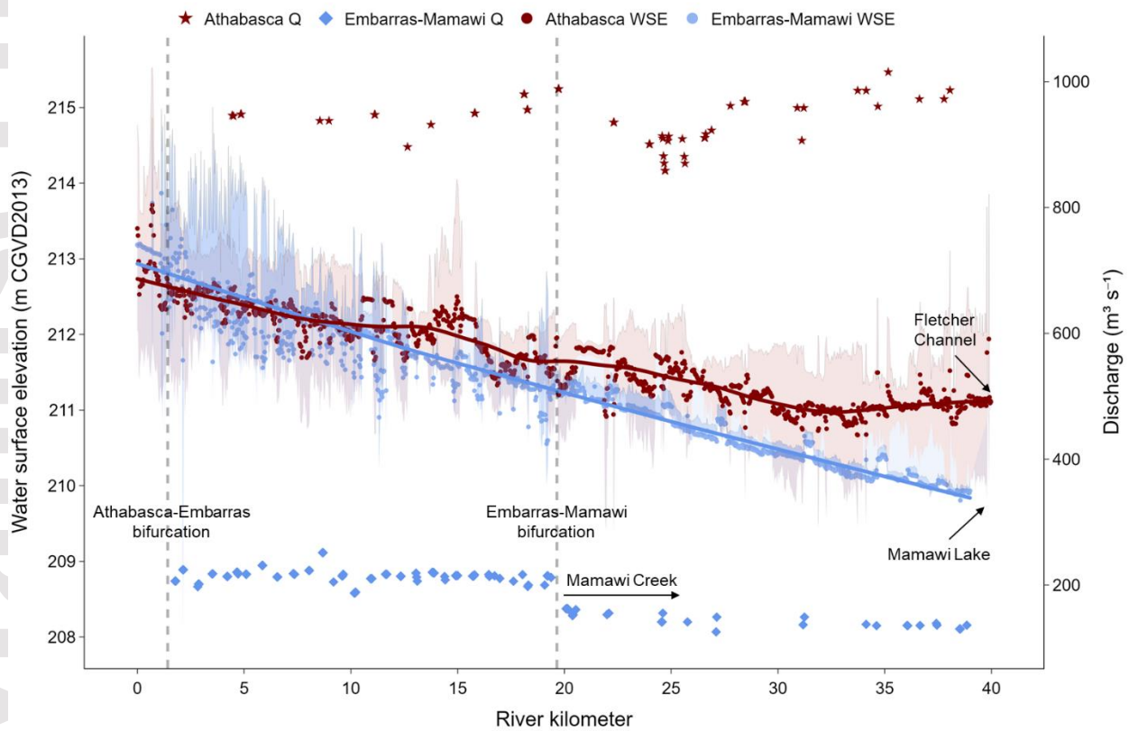
Figure 9. Longitudinal profiles of water surface elevation (WSE) and discharge (Q) collected August 5-13, 2018 along the Athabasca River and the Embarras-Mamawi (EM) channel downstream of the Athabasca-Embarras bifurcation. Regression lines are from locally weighted scatterplot smoothing (LOWESS). Uncertainty bounds (shaded envelopes) represent the standard deviation for each averaged WSE measurement.
