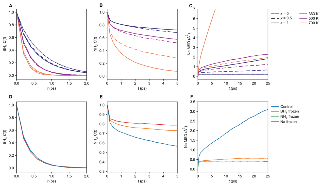
Figure 3. (A,D) Borohydride and (B,E) amide orientation autocorrelation functions and (C,F) sodium MSD. A–C) AIMD simulations of Na 3-x O 1-x (NH 2 ) x (BH 4 ) for x = 0, 0.5, 1, and T = 363, 500, and 700 K. Borohydride rotation is relatively unchanged throughout the anion substitution while amide rotation shows a strong speedup as the proportion of amide to oxide anion increases within the 700 K condition. D–F) Simulations of Na 2 (NH 2 )(BH 4 ) with either sodium, amide, or borohydride ions artificially frozen. Borohydride rotation remains insensitive to freezing of other ionic species, while the rates of amide rotation and sodium migration are slowed by any other ion freezing.
