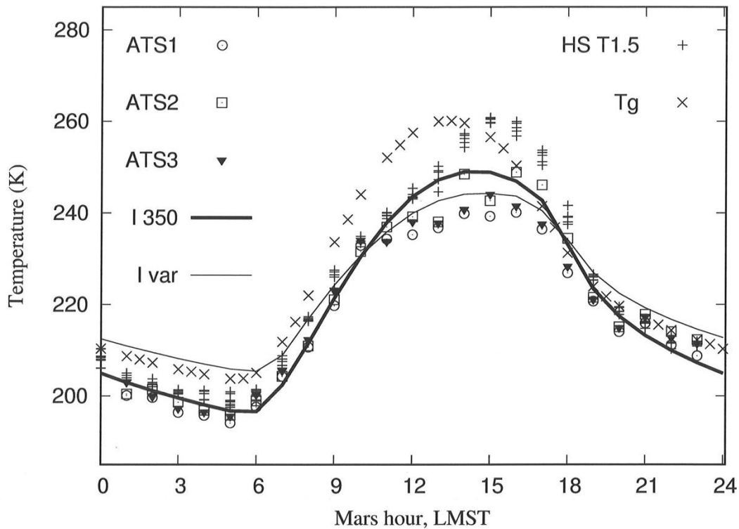
Fig. 7. Air temperatures at \sim 1.45 m height for sol 143 from MEDA ATS and HS (symbols), and from SCM simulations (lines) for I = \text{var} ( \sim 600 ) and for I = 350 . Observed T_g is also shown.
