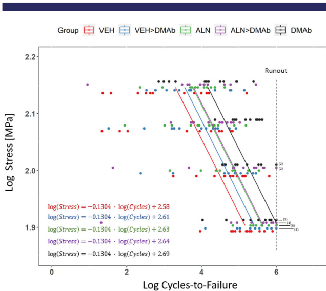
Fig. 3. Stress versus fatigue life relationships from mechanical fatigue tests. Lines indicate the stress-life relationship as predicted by our survival analysis model. these data points are the same as those shown in Fig. 2. Bracketed numbers indicate the number of samples that survived to a runout of 1 million cycles. Group \times stress interactions were not significant.
