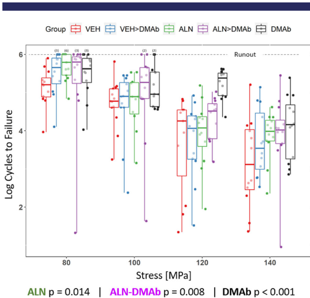
Fig. 2. Results from mechanical fatigue tests. Survival analysis demonstrated a significant effect of load level ( p < 0.001 ), where samples at higher loads survived fewer cycles until failure. Moreover, the analysis also demonstrated that samples from animals treated with ALN (green; p = 0.014 ) ALN-DMAB (purple; p = 0.008 ) and DMAB (black; p < 0.001 ) survived more cycles than samples from animals treated with VEH. Boxes indicate the 25th, 50th, and 75th percentile of data, and whiskers indicate the full range. Bracketed numbers indicate number of samples that survived to a runout of 1 million cycles.
