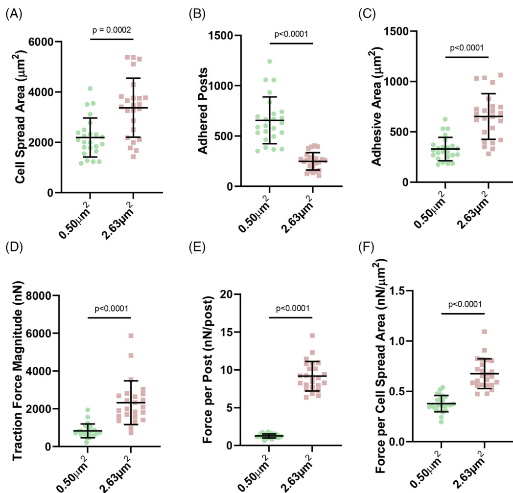
FIGURE 6 Post Area Influence on hMSC Mechanoresponses. (A) Cell spread area (mean \pm SD). Two-sided unpaired t-test p = .0002 . (B) Total number of adhered posts (mean \pm SD). Two-sided t-test with Welch's correction factor p < .0001 . (C) Adhesive Area (mean \pm SD) Two-sided t-test with Welch's correction factor p < .0001 . (D) Traction Force Magnitude (mean \pm SD). Mann-Whitney test p < .0001 . (E) Force per Post (mean \pm SD). Two-sided t-test with Welch's correction factor p < .0001 . (F) Force per Cell Spread Area (mean \pm SD). Two-sided t-test with Welch's correction factor p < .0001 . n = 24 for the 0.50 \mu\text{m}^2 and n = 24 for the 2.63 \mu\text{m}^2 conditions.
