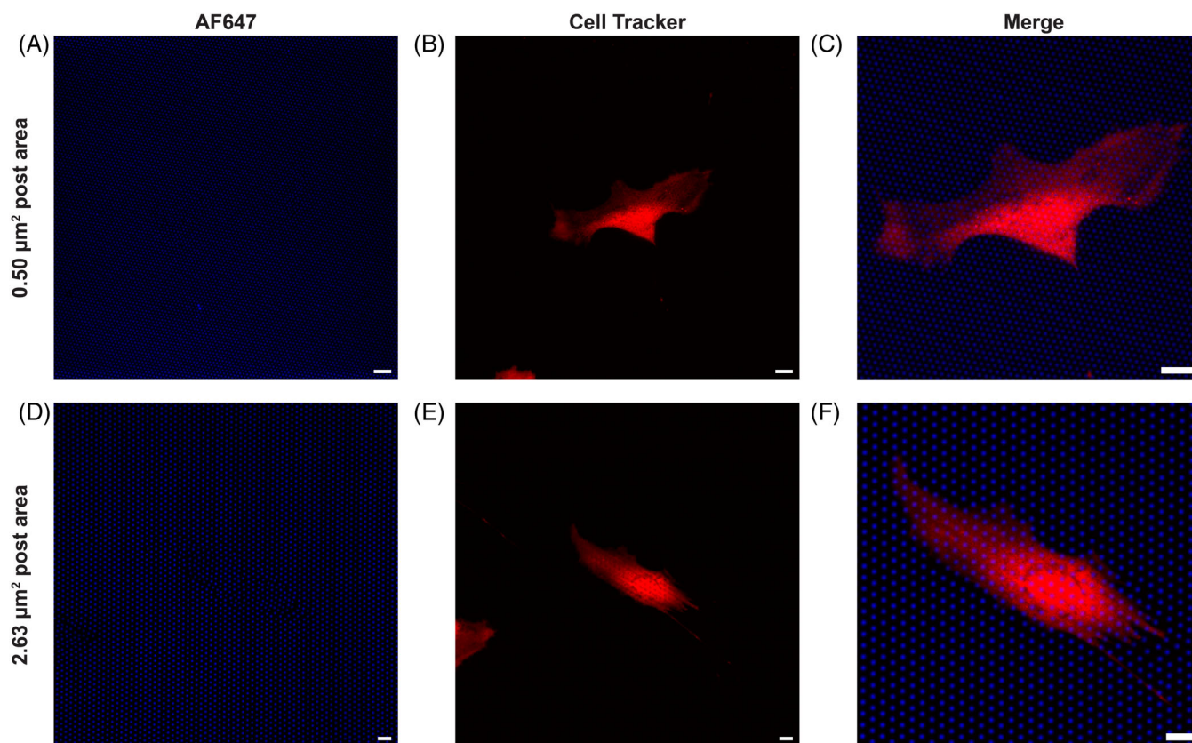
FIGURE 5 Confocal Microscopy Representative Images. (A) Mini ( 0.50 \mu\text{m}^2 post area) post image. (B) Cell tracker image of hMSC on 0.50 \mu\text{m}^2 post area mPAD. (C) Merge image of the post and cell tracker images on 0.50 \mu\text{m}^2 post area mPAD. (D) Regular ( 2.63 \mu\text{m}^2 post area) post image. (E) Cell tracker image of hMSC on 2.63 \mu\text{m}^2 post area mPAD. (F) Merge image of the post and cell tracker images on 2.63 \mu\text{m}^2 post area mPAD. Scale bar 10 \mu\text{m} .
