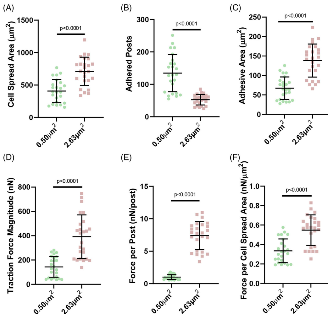
FIGURE 4 Post Area Influence on MEF Mechanoresponses. (A) Cell Spread Area (mean \pm SD). Two-sided unpaired t-test p < .0001 . (B) Total number of adhered posts (mean \pm SD). Two-sided t-test with Welch's correction factor p < .0001 . (C) Adhesive Area (mean \pm SD) Two-sided unpaired t-test p < .0001 . (D) Traction Force Magnitude (mean \pm SD). Two-sided t-test with Welch's correction factor p < .0001 . (E) Force per Post (mean \pm SD). Two-sided t-test with Welch's correction factor p < .0001 . (F) Force per Cell Spread Area (mean \pm SD). Two-sided unpaired t-test p < .0001 . n = 24 for the 0.50 \mu\text{m}^2 and n = 25 for the 2.63 \mu\text{m}^2 conditions.
