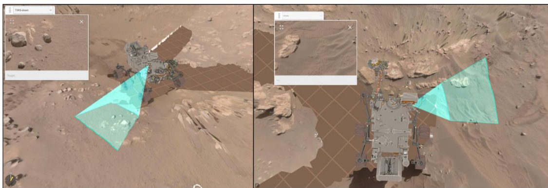
Figure S1. Images showing the modeled TIRS FOV corresponding to the Mars 2020 location for sols 52 - 65 (left) and 287 – 328 (right). Images are obtained from the Mars 2020 Advanced Science Targeting Tool for Robotic Operations (ASTTRO).
