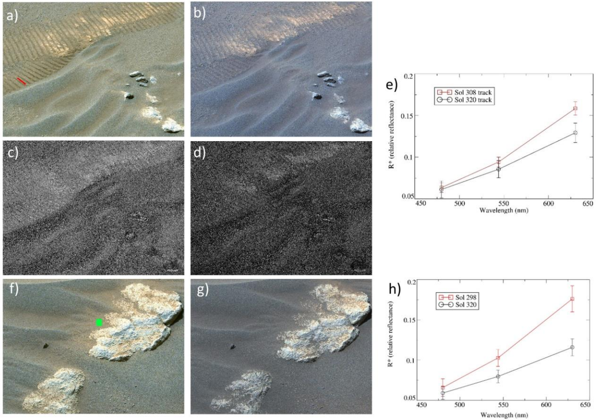
Figure 3. (a,b) Mastcam-Z Bayer filter image of the wheel tracks in the TIRS FOV before (a) and after (b) the storm; (c,d) Green Bayer filter band depth images corresponding to (a,b) images, respectively; (e) Comparison of Bayer-filter (3-band) relative reflectance spectra of rover track (red box in (a)) from before and after the storm; (f,g) Mastcam-Z Bayer filter image of region within the TIRS FOV before (f) and after (g) the storm; (h) Comparison of Bayer-filter relative reflectance spectra of regolith (green box in (f)) from before and after dust storm. Details on images are provided in Table 2.
