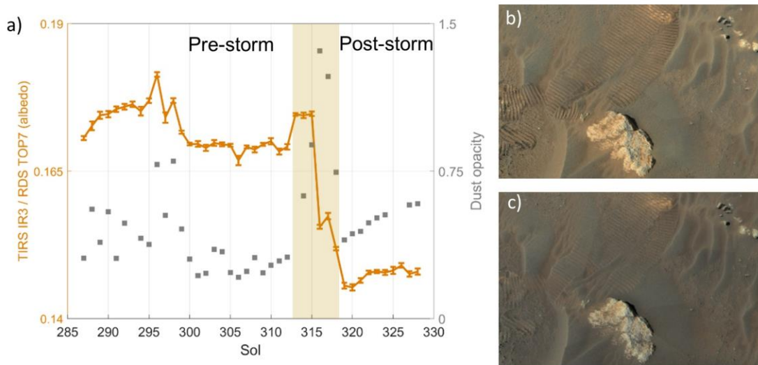
Figure 2. (a) Change in surface albedo at 13:00 LMST (dark orange) and dust opacity around noon (gray) between sols 287 and 328. (b,c) Comparison of portions of Mastcam-Z vertical projection mosaics corresponding to the TIRS field of view before (b) and after (c) the dust storm.
