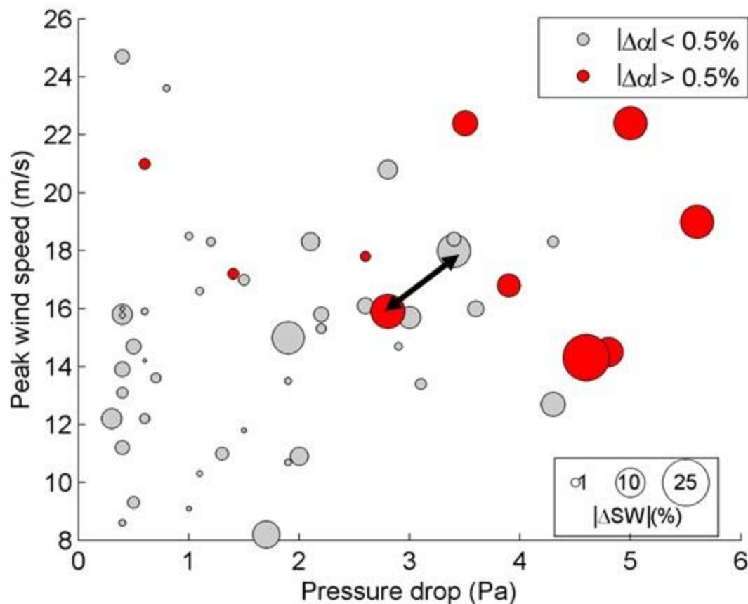
Figure 5. Scatter plot of the dust devil features presented in Section 3. Each dust devil is represented with a circle, distributed as a function of the pressure drop and peak wind speed. The size of the circle represents the measured decrease in shortwave radiation. Dust devils causing an unambiguous albedo change are highlighted in red. The black arrow connects two similar dust devils that occurred 100 minutes apart, which are discussed in Section 5.2.
