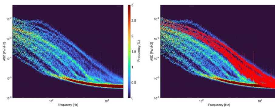
Figure 4. (Left) The probabilistic distribution of the Amplitude Spectral Densities (ASD) of the Supercam microphone recordings as a function of frequency from landing to sol 317 in the period 15:00 - 19:00 LTST. The color code indicates the likelihood of a given spectral density, with blue being the least common. (Right) As in the left panel, but with the three most energetic Supercam microphone recordings on sol 317 highlighted in red.
