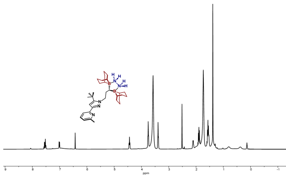
Figure S41. ^1\text{H} NMR spectrum (THF, 23 °C) of (\text{BBN})_2\text{NN}^t\text{Bu}(\text{N}_2\text{H}_4) .
