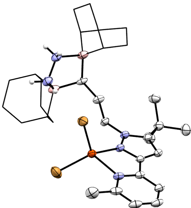
Figure S106. Molecular structure of ((\text{BBN})^2\text{NN}^{\text{tBu}})\text{FeBr}_2(\text{N}_2\text{H}_4) displayed with 50% probability ellipsoids. Hydrogen atoms not attached to hydrazine unit are omitted for clarity. The 9-BBN substituents are displayed in wireframe for improved clarity.
