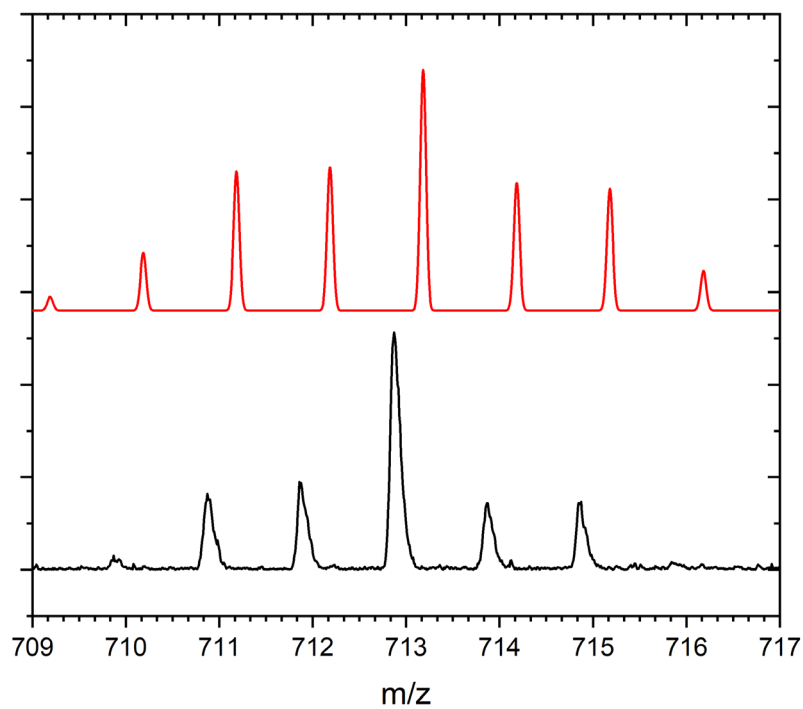
Figure S62. MALDI-TOF spectrum of (\text{BBN})_2\text{NN}^{\text{tBu}}\text{FeBr}_2(\text{N}_2\text{H}_4) (bottom, black) and simulation (top, red).
