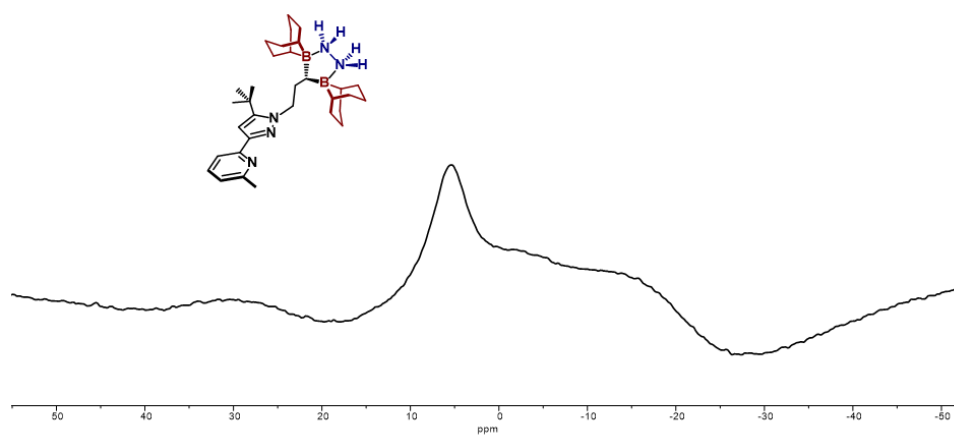
Figure S42. ^{11}\text{B} NMR spectrum (THF, 23 °C) of (\text{BBN})_2\text{NN}^t\text{Bu}(\text{N}_2\text{H}_4) .
