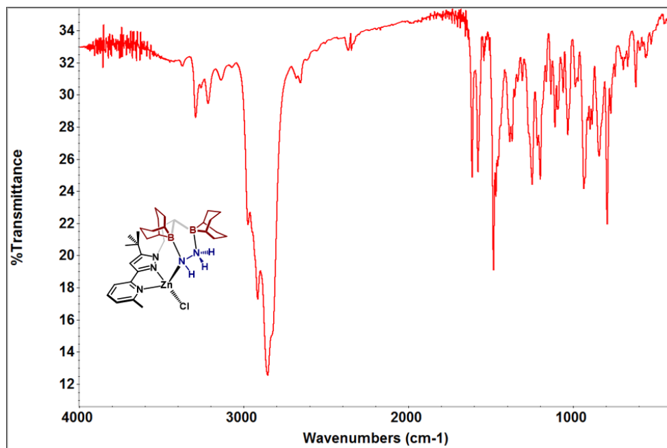
Figure S73. Infrared spectrum (KBr) of (^{(BBN)2}NN^{tBu})ZnCl(N_2H_3) .
