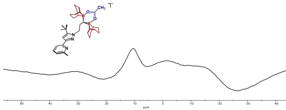
Figure S26. ^{11}\text{B} NMR spectrum ( \text{THF} , 23 °C) of [(\text{BBN})_2\text{NN}^{\text{tBu}}(\text{OAc})](\text{K-18-crown-6}) .
