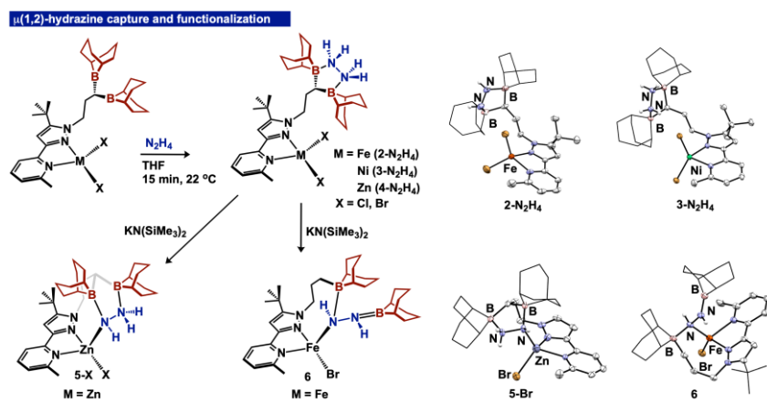
Figure 5. \mu(1,2) -hydrazine capture using 2-4 to yield 2-4-N 2 H 4 and hydrazine reactivity of 2-N 2 H 4 and 4-N 2 H 4 to generate hydrazido and diazene complexes 5-X and 6 ( \text{X} = \text{Br, Cl} ). Molecular structures of 2-N 2 H 4 , 3-N 2 H 4 , 5-Br and 6 (right). Thermal ellipsoids displayed at 50% probability. Non-diazene or hydrazine H-atoms are omitted, and the 9-BBN substituents are displayed in wireframe for improved clarity.
