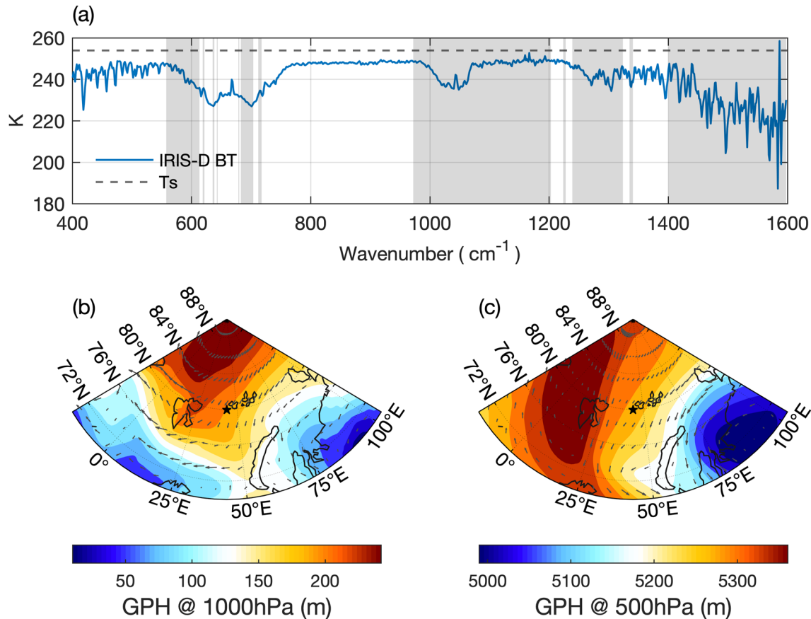
Figure 1. (a) The Infrared Interferometer Sounder-D (IRIS-D) spectra of Case 1 shown in brightness temperature. It was measured on 21 April 1970 at 80.0°N, 43.4°E. The dashed line denotes the corresponding surface skin temperature from the ERA5 hourly reanalysis data. The gray shades denote the IRIS-D channels not used in the retrieval due to (1) absorption of greenhouse gases other than H 2 O and CO 2 , that is, O 3 , CO, N 2 O, and CH 4 , and (2) large measurement noises (1,400–1,600 cm -1 ). (b) ERA5 1,000-hPa geopotential height (GPH) in color and the horizontal wind field for the time of observation. The black pentagram marks the geolocation of Case 1. (c) Same as (b) but on 500 hPa pressure level.
