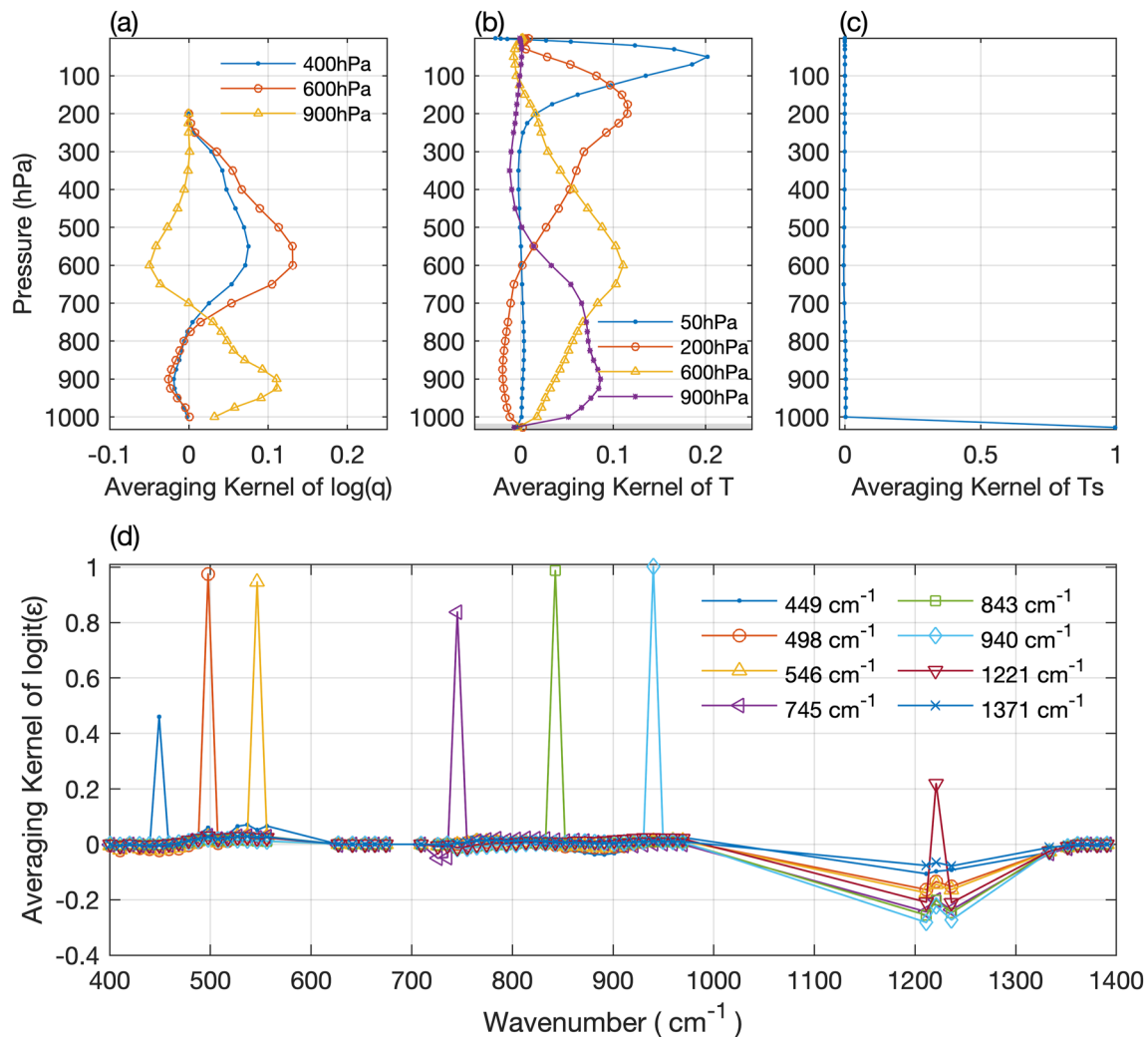
Figure 5. Averaging kernels of selected state variables in Case 1: (a) for logarithmic specific humidity on pressure levels of 400, 600, and 900 hPa, (b) for air temperature on four pressure levels from middle stratosphere to lower troposphere (c) for surface skin temperature, and (d) for logit-transformed surface spectral emissivity on eight random channels. The shaded layer in subpanel (b) is to highlight the pressure level of surface skin temperature. For better visualization, the averaging kernels for humidity and temperature at other pressure levels are not shown.
