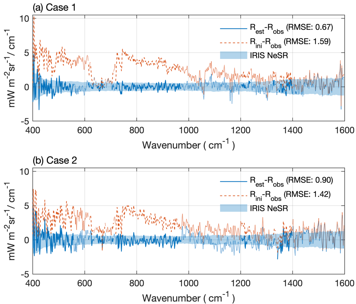
Figure 6. (a) The blue curve represents the difference between the radiances based on the retrieved state variables and the Infrared Interferometer Sounder-D (IRIS-D) observations, that is, the residual radiances for Case 1 on 21 April 1970, and the root-mean-squared error (RMSE) is 0.67 \text{ mW m}^{-2} \text{ sr}^{-1} / \text{cm}^{-1} . The red dash curve represents the residual radiances based on the initial guess which consists of the temperature and humidity fields from the ERA5 hourly reanalysis and constant surface spectral emissivity at 0.95. Its RMSE is 1.59 \text{ mW m}^{-2} \text{ sr}^{-1} / \text{cm}^{-1} . As in previous figures, solid part denotes the selected channels used in the retrieval while the dotted part denotes the channels not used in the retrieval. The blue shade represents the IRIS-D noise-equivalent spectral radiance ( \pm 1\sigma ). (b) Same as (a), but for the Case 2 measured on 13 July 1970.
