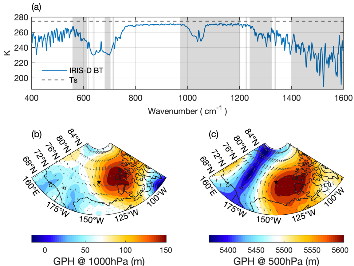
Figure 2. Same as Figure 1, but for the Case 2 observed on 13 July 1970 at 76.2°N, 215.4°E.
