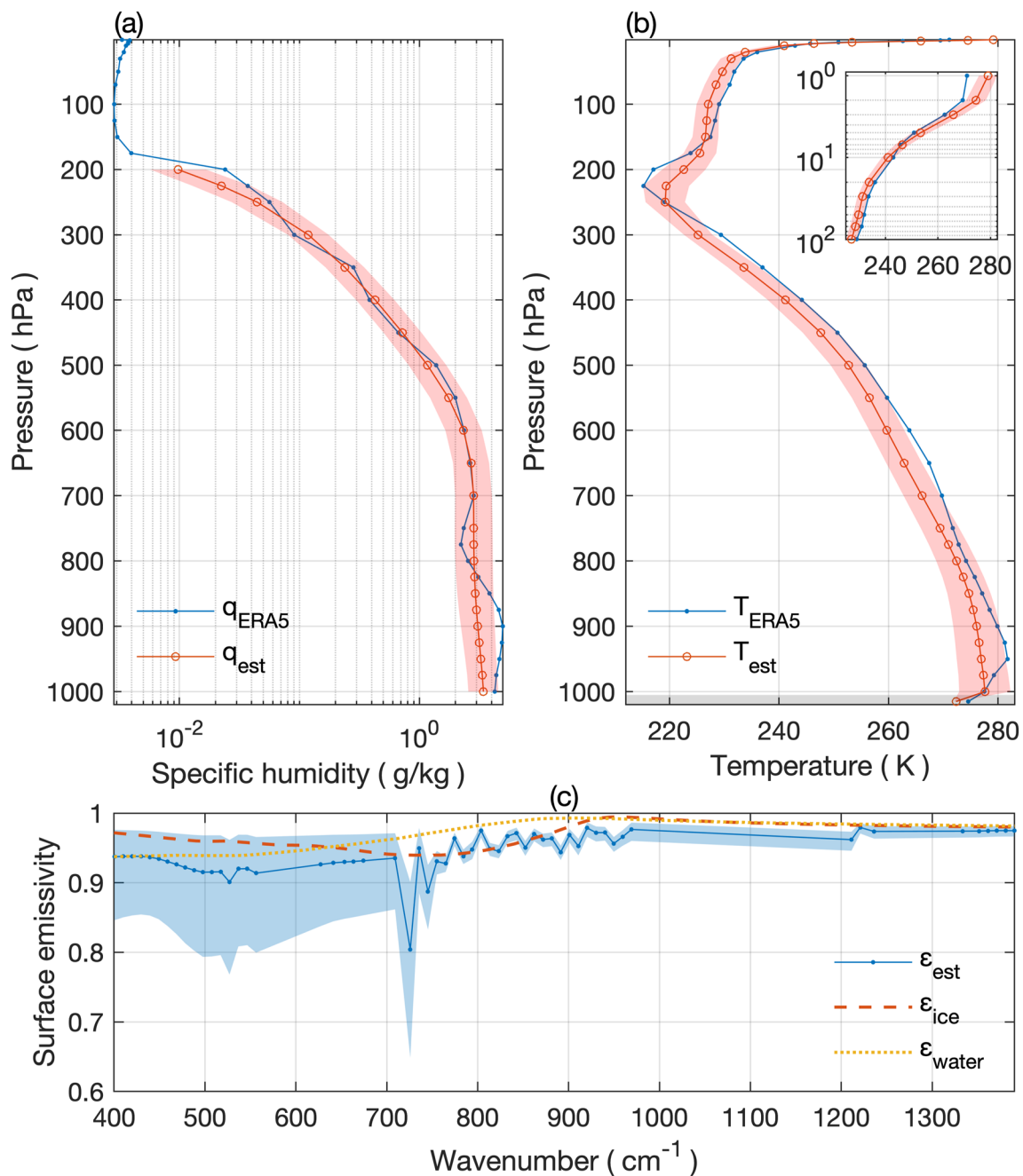
Figure 8. Same as Figure 7, but for the Case 2 observed on 13 July 1970.
