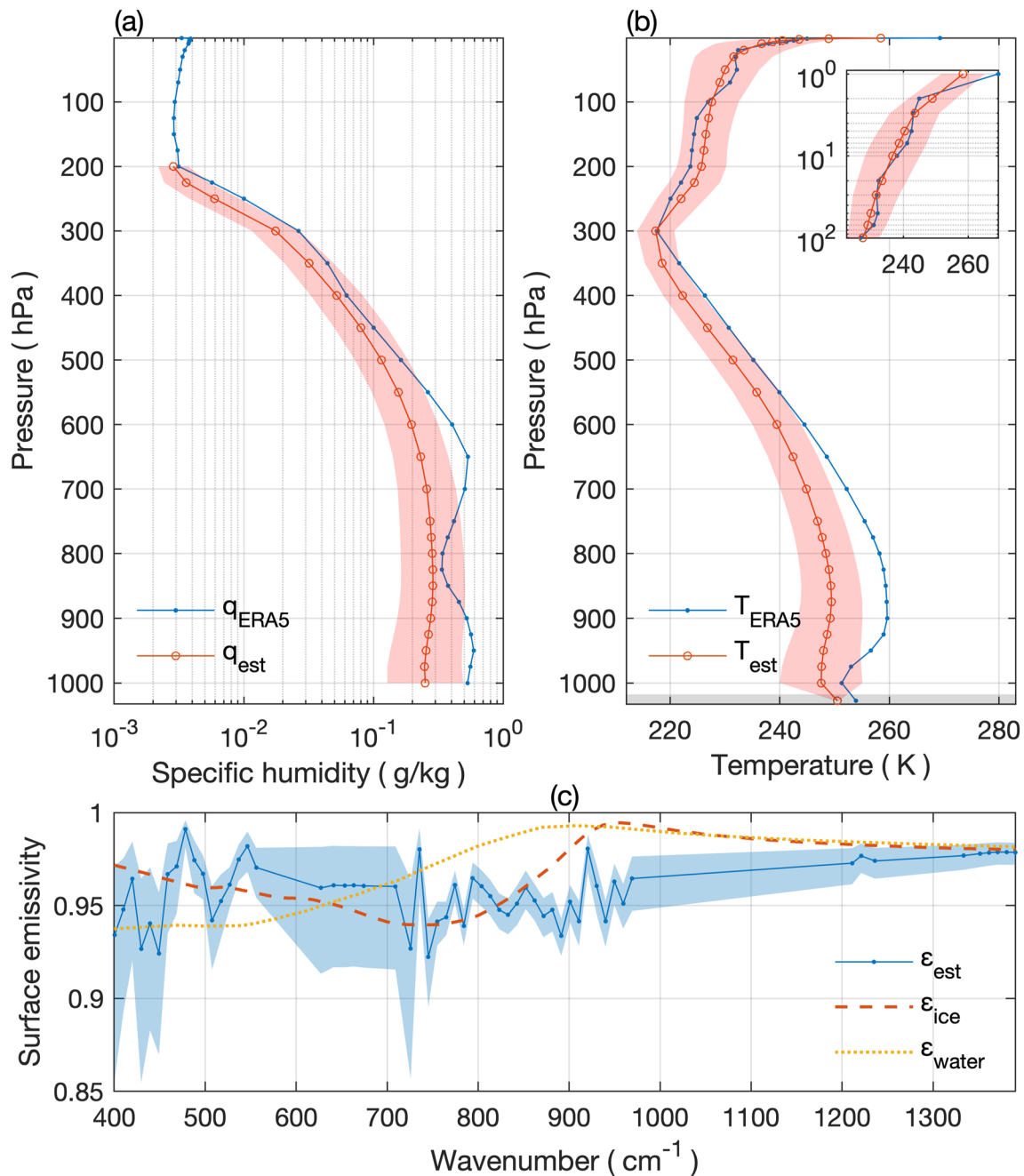
Figure 7. Retrieval estimates of the state variables for Case 1 on 21 April 1970. (a) The blue curve represents the specific humidity profile from the ERA5 hourly reanalysis up to 1 hPa (i.e., initial guess). The red curve represents the retrieved specific humidity between 200 and 1,000 hPa with the retrieval uncertainty denoted by the red shade. (b) Similar to (a), but for the temperature profile from 1 hPa to the surface. The shaded layer is to highlight the pressure level of surface skin temperature. (c) The blue curve represents the retrieved surface spectral emissivity with the retrieval uncertainty denoted by the blue shade. The surface emissivity spectra for ice and water are from a global surface emissivity database (Huang et al., 2016).
