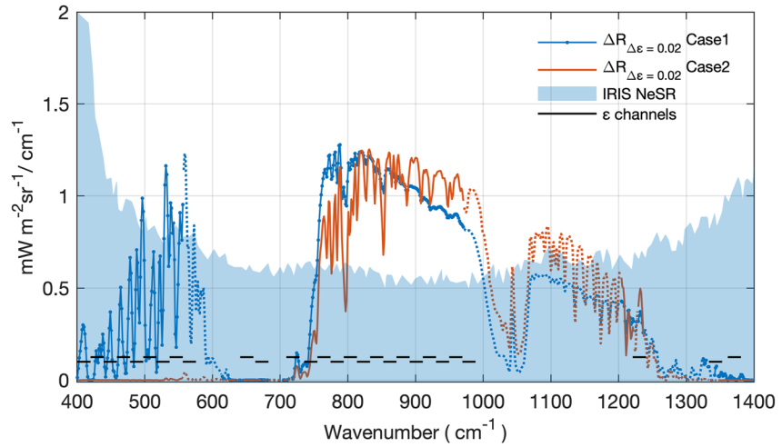
Figure 4. Radiances change at top-of-atmosphere in response to an increase of surface spectral emissivity by 0.02 for Case 1 and Case 2, denoted by blue curve with dot and red curve, respectively. For both curves, solid part represents the selected Infrared Interferometer Sounder-D (IRIS-D) channels used in the retrieval, while the dotted part represents the channels not used in the retrievals (refers to Section 2.1 for further details.) The blue shade denotes the IRIS-D noise-equivalent spectral radiance ( 1\sigma ). The black horizontal lines, each covering a 10 \text{ cm}^{-1} spectral interval, indicate channels on which surface spectral emissivity are retrieved.
