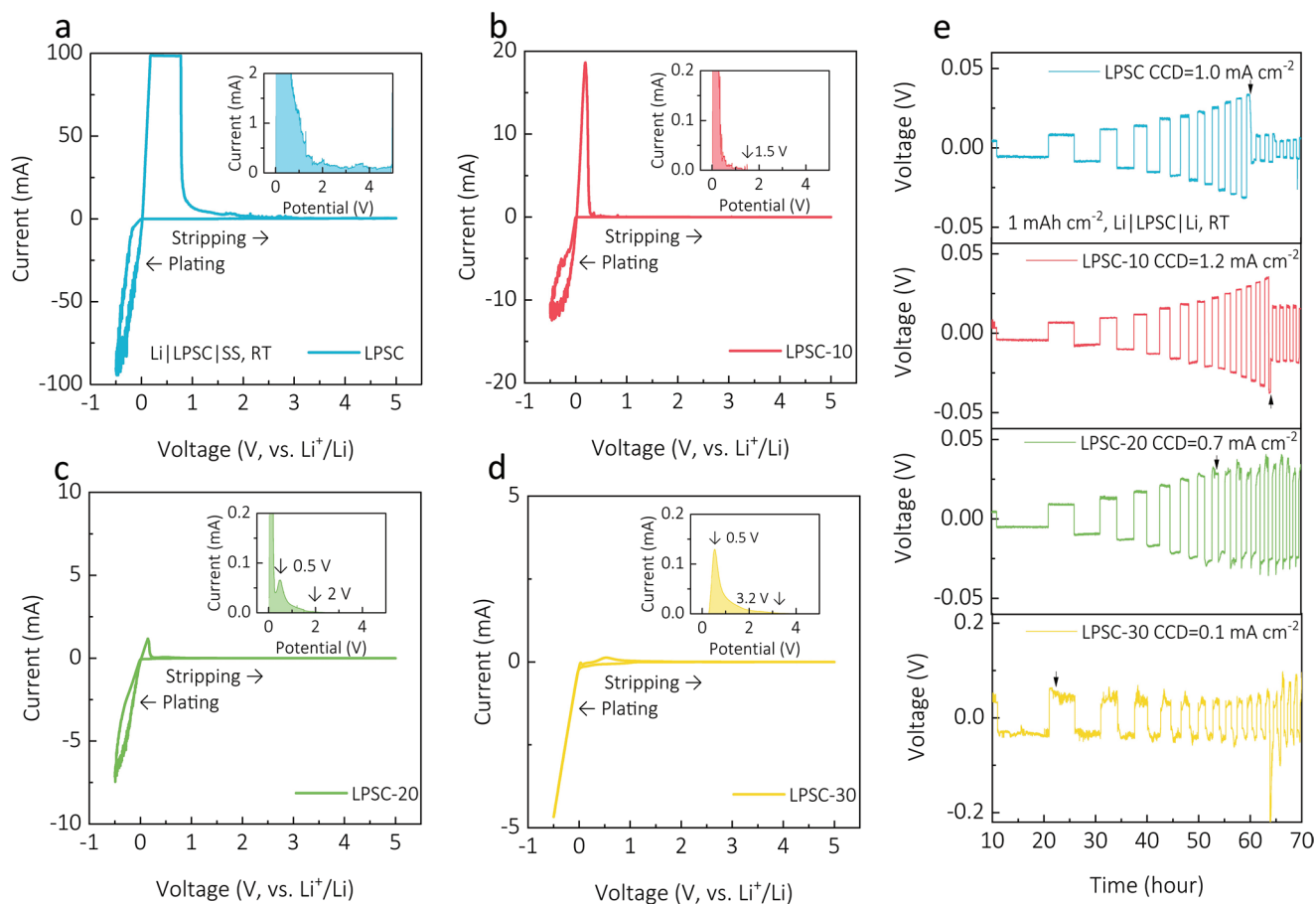
Figure 3. Lithium-anode compatibility of the sulfide samples sintered at 500 °C. The cyclic voltammety plots of the asymmetric Li|SE|SS cells: a) LPSC; b) LPSC-10; c) LPSC-20; d) LPSC-30. e) The voltage profiles of the symmetric Li|SE|Li cells for the galvanostatic test. Employing the increased step size current density (0.1 mA cm -2 ) to obtain CCD values, where the cut-off capacity of each step is fixed as 1 mAh cm -2 .
