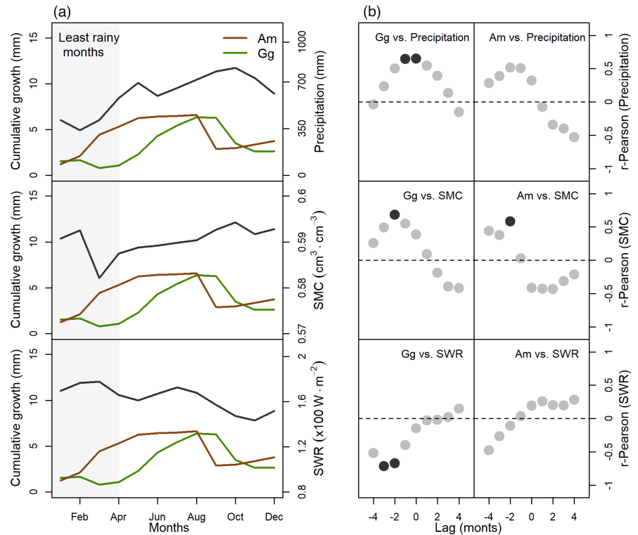
FIGURE 6 (a) Comparison between mean monthly growth for two species (Am: Apeiba macropetala , and Gg: Goupia glabra ) and environmental factors (precipitation in millimetres, soil moisture content [SMC] expressed in volumetric units \text{cm}^3 \text{cm}^{-3} and short-wave radiation [SWR] in \text{W m}^{-2} ). (b) Cross-correlation function between tree species and the same environmental factors. The gapless annual dendrometer records become from different individuals: n = 3 ( A. macropetala ) and n = 6 ( G. glabra ). Grey shading: represents the least rainy months which not implying water deficit. Black dots indicate significant correlation ( p < 0.05 ).
