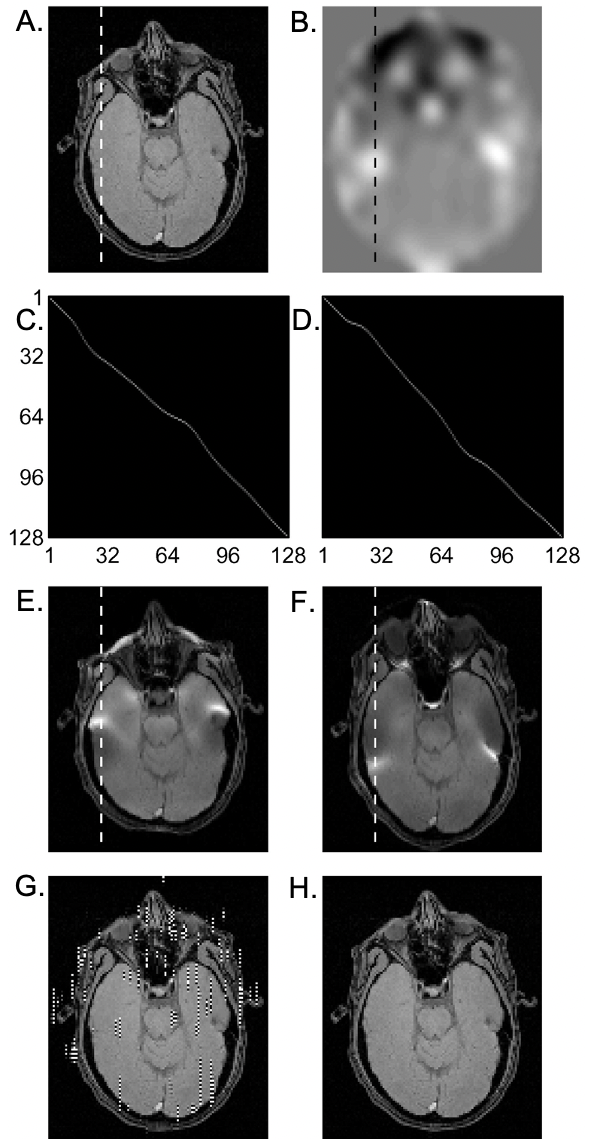
Figure 8: Illustration of EPI distortion correction using Eq. (14). (A) Ground-truth (undistorted) object and (B) fieldmap. (C,D) \mathbf{K}_{+,i} and \mathbf{K}_{-,i} for the dashed lines in (E,F). (E,F) Distorted images \mathbf{f}_+ and \mathbf{f}_- . (G) Distortion correction attempt using only \mathbf{f}_+ . (H) Successful distortion correction using Eq. (14). (Images reused from Andersson et al., 2003 [75] with permission.)
