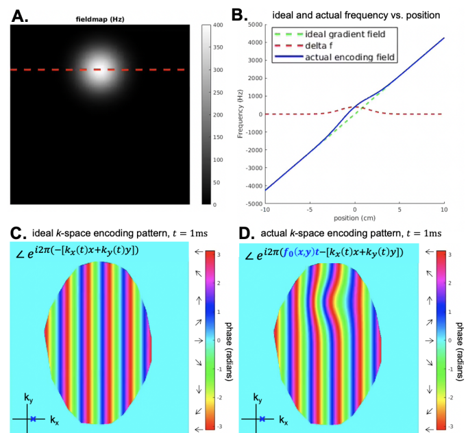
Figure 5: Ideal vs. actual encoding phase at a single k-space location. A. Simulated off-resonance fieldmap in Hz. B. 1D plots of the encoding fields as a function of position, where the red dotted line correspond to the dotted red line in A. C. The ideal k-space encoding phase for (k_x, k_y) = (0, 0.426 \text{ cm}^{-1}) . D. The actual k-space encoding phase for (k_x, k_y) = (0, 0.426 \text{ cm}^{-1}) . Combined with k-space encoding errors at other k-space sampling locations, this phase error will lead to off-resonance image artifacts.
