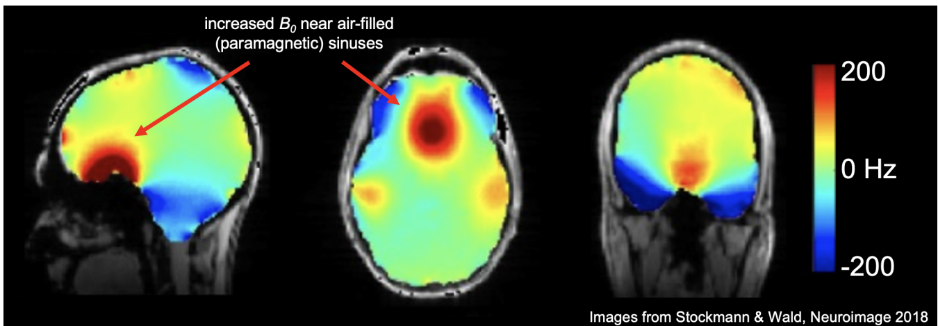
Figure 2: B_0 magnetic field in the brain at 7T with 2 nd order shimming. This fieldmap shows the spatially varying patterns of the B_0 field in the human brain (superimposed over an anatomical image). Even after 2 nd order shimming has been applied to flatten the field, higher order field inhomogeneities persist. Arrows show that near the air-filled, and therefore paramagnetic, sinuses, the B_0 field is higher than areas in the center of the mostly diamagnetic brain tissue. (Images reused from Stockmann & Wald, 2018 [35] with permission.)
