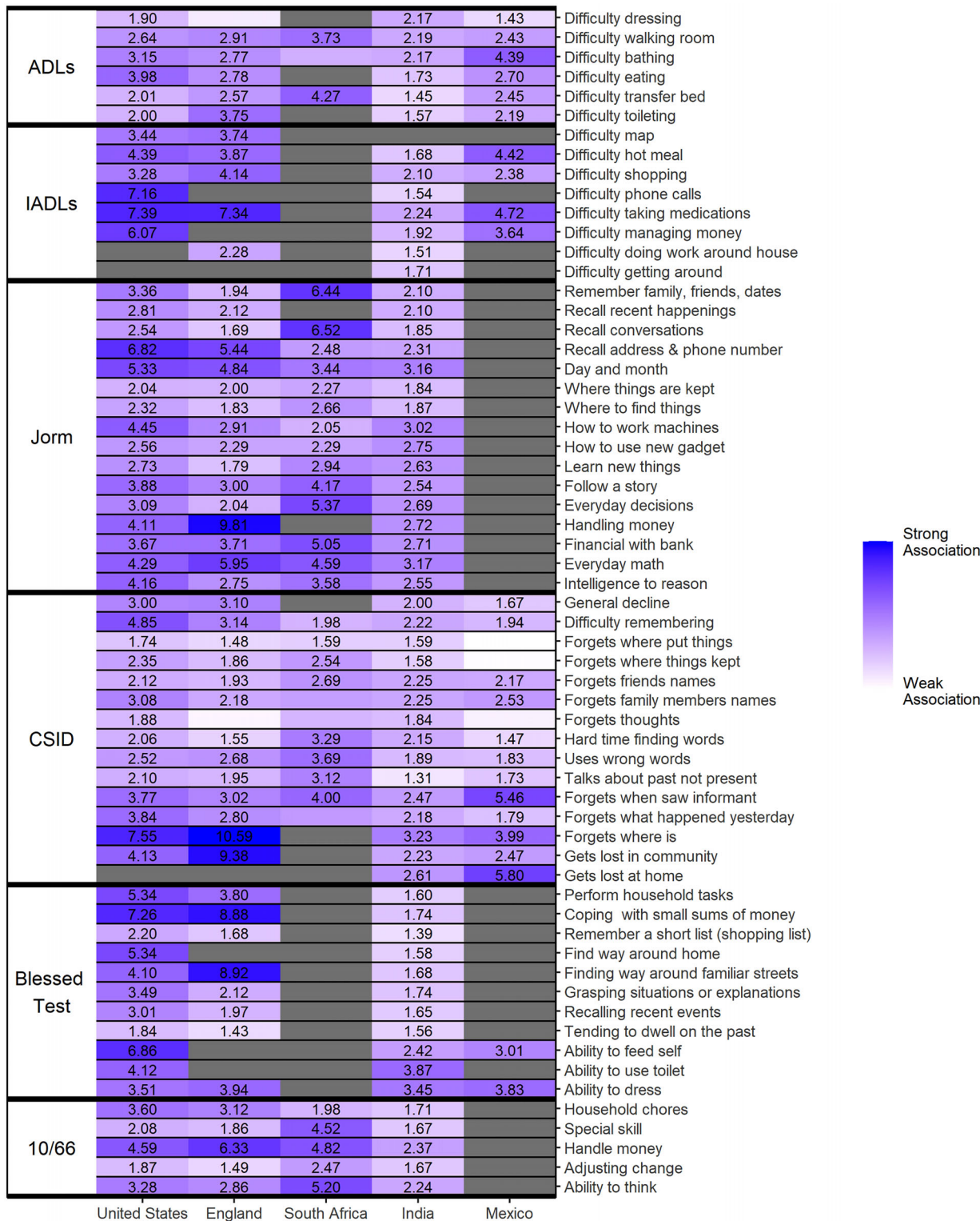
FIGURE 1 Associations between each item on functional limitations and cognitive impairment by domain for each HCAP conducted in the United States (N = 3329), England (N = 1255), South Africa (N = 560), India (N = 4095), and Mexico (N = 2011) from logistic regression models, controlling for age and sex. Odds ratios are displayed for significant associations. For example, the number 1.90 in the upper left corner indicates that in the United States, individuals who had difficulty dressing had an odds of cognitive impairment that was 1.90 times the odds of dementia for those who did not have difficulty dressing. Grey boxes represent instances where an item was not administered or an odds ratio was suppressed due to small cells. Color scale shows differences in associations on the log odds scale. HCAP, Harmonized Cognitive Assessment Protocol Studies.
