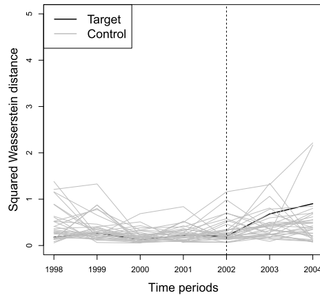
FIGURE 3.—Placebo permutation test following Algorithm 2 with target AK.
