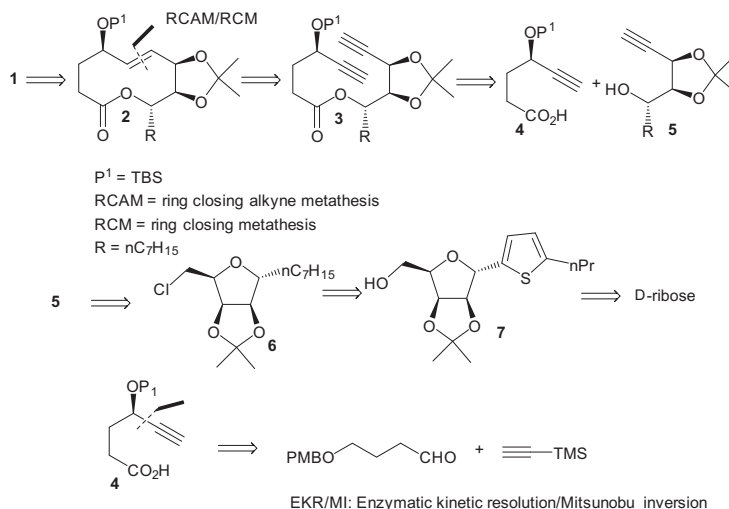
Scheme 1. Retrosynthetic analysis of mangiferaelactone 1 using C-alkylglycosides.
