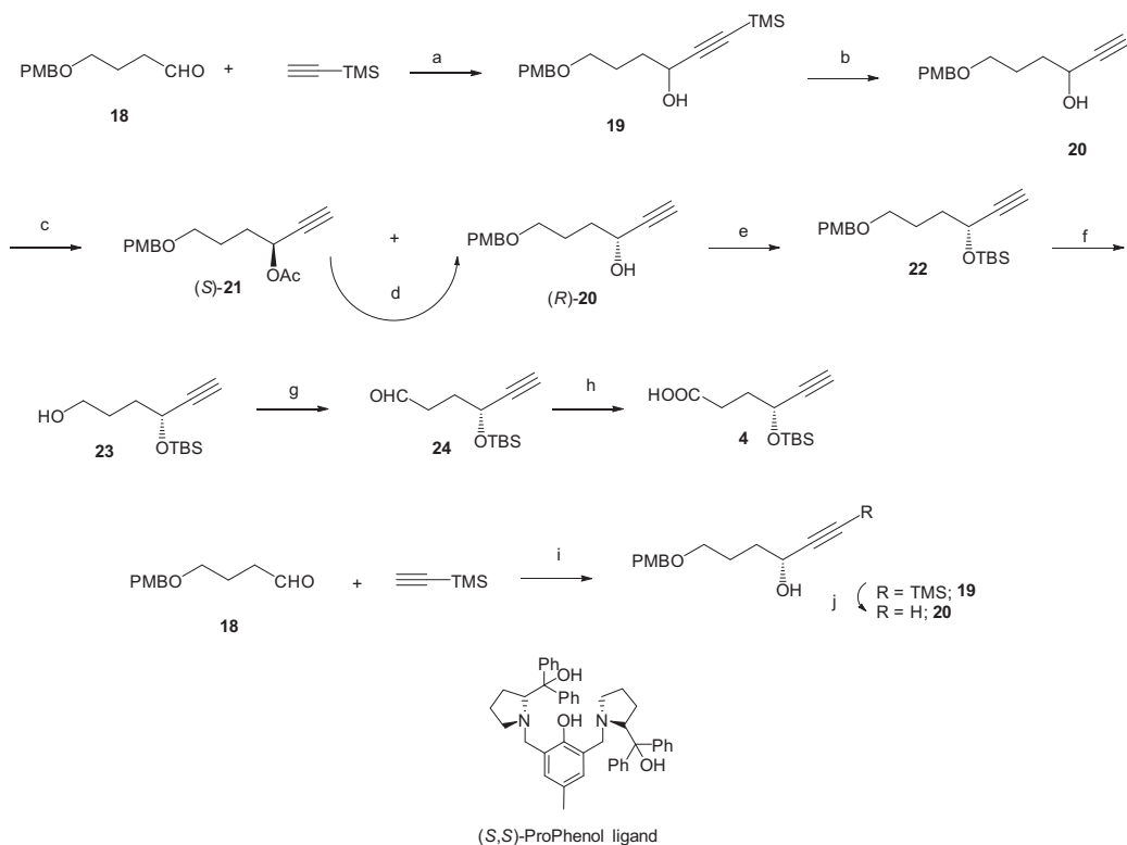
Scheme 3. Reagents and conditions: (a) n -BuLi, TMS acetylene, THF, –78 °C–rt, 90%; (b) K 2 CO 3 , MeOH, 0 °C, 95%; (c) CAL-B, vinyl acetate, 1 Pr 2 O, 4 Å-MS, 1 h; (d) (i) K 2 CO 3 , MeOH; (ii) PPh 3 , DIAD, PhCOOH; (iii) 1% NaOH in MeOH; (e) imidazole, TBS-Cl, DCM, rt, 95%; (f) DDQ, DCM/H 2 O (19:1), rt, 1 h, 96%; (g) (COCl) 2 , DMSO, Et 3 N, DCM, –78 °C, 90%; (h) NaClO 2 , NaH 2 PO 4 , 2-methyl-2-butene, t -BuOH/H 2 O (1:1), rt, 2 h 80%; (i) (S,S)-Pro-Phenol, Ph 3 PO, Me 2 Zn, toluene, 60%; (j) same as b, 95%.
