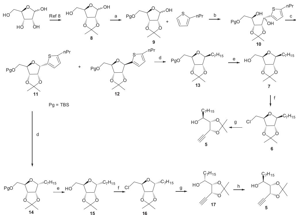
Scheme 2. Reagents and conditions: (a) TBDMSCl, imidazole, DCM, rt, 98%; (b) n -BuLi, THF 0 °C–rt, 2 h, 75%; (c) DIAD, Ph 3 P, THF 0 °C–rt, 3 h, 91%; (d) Raney-Ni, EtOH, 80 °C, 4 h, 75%; (e) 1 M TBAF, THF, 88%; (f) Ph 3 P, CCl 4 , 5 h, reflux 88%; (g) LiNH 2 , NH 3 (l), –30 °C, THF, 5 h, 85%; (h) DIAD, Ph 3 P, PhCO 2 H, 1% NaOH, 86% (for two steps).
