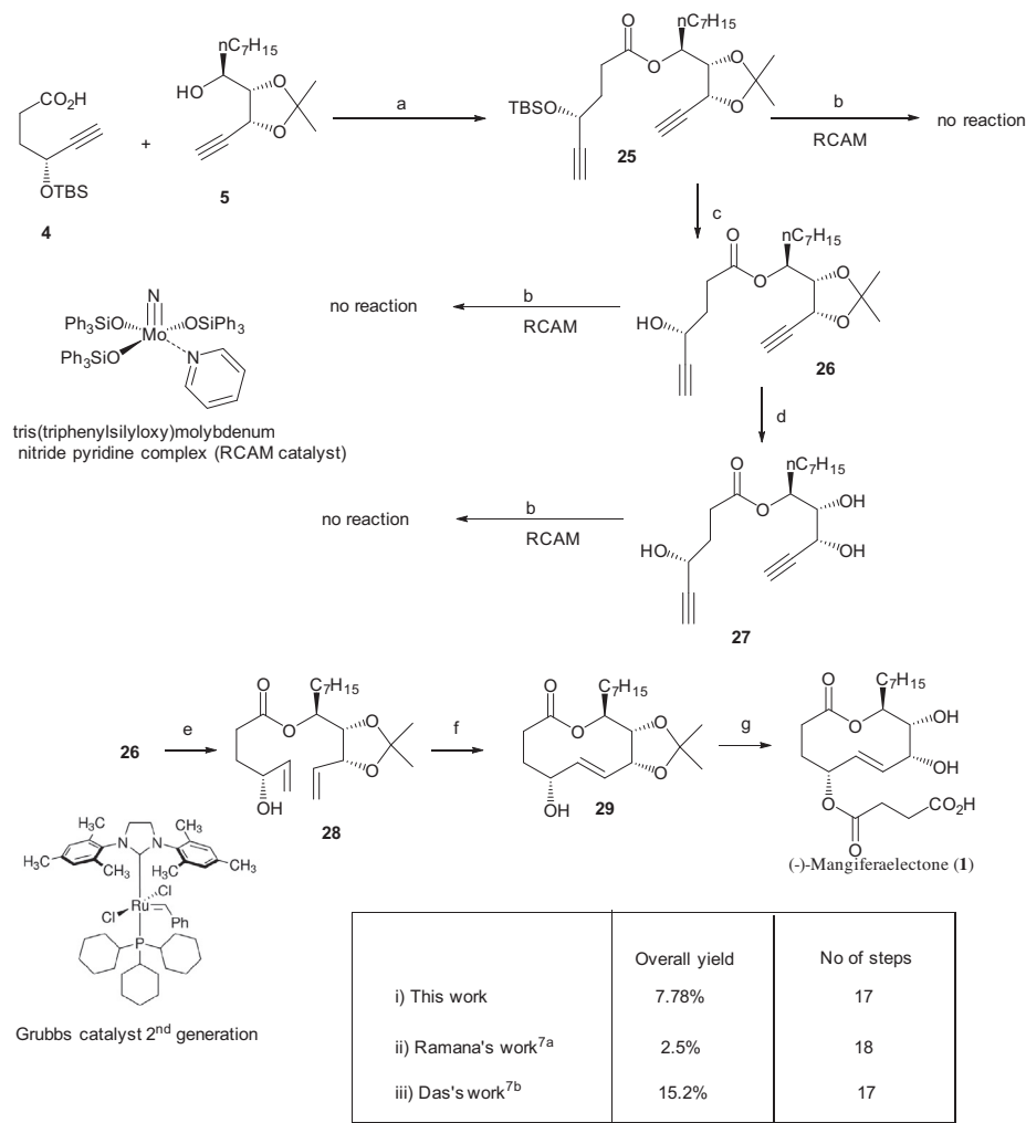
Scheme 4. Reagents and conditions: (a) 2,4,6-trichlorobenzoyl chloride, Et 3 N, DMAP, toluene 0 °C to rt, 6 h, 96%; (b) tris(triphenylsilyloxy)molybdenum nitride pyridine complex, toluene, 80 °C; (c) HF-pyridine, THF, 4 h, 88%; (d) 2 N HCl, THF, rt, 6 h, 90%; (e) Lindlar's catalyst, H 2 , Pd-C, EtOAc, 80%; (f) G-II (10 mol %), DCM, 10 h, 85%; (g) succinic anhydride, EDCI-HCl, DMAP, and then same as d.
