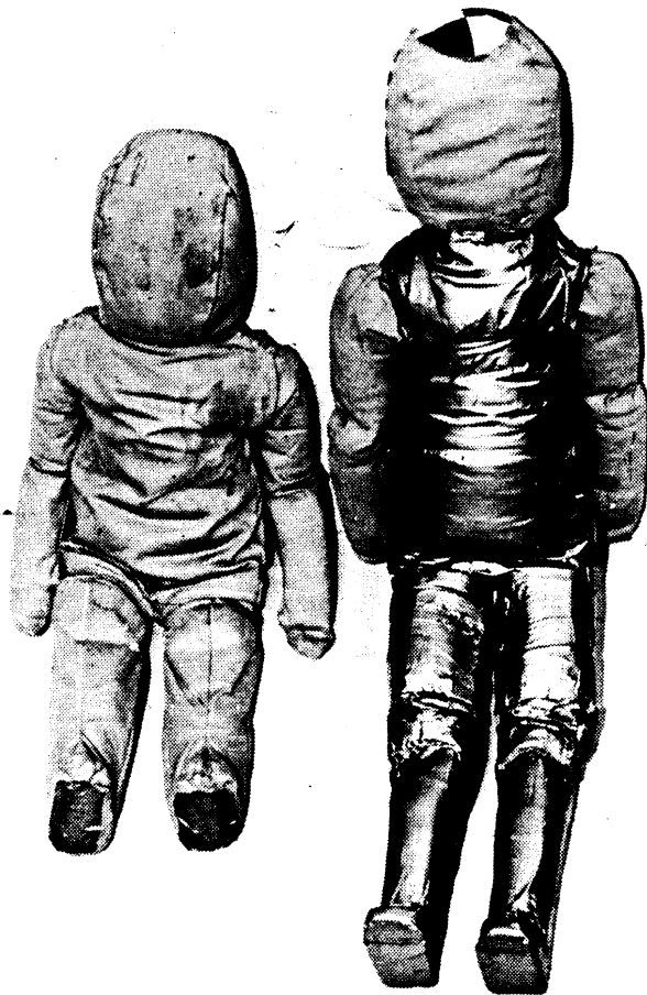
FIGURE 20. Part 572 6-Month and UMTRI 1-Year Dummies
