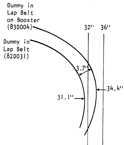
FIGURE 34. Head Arc Comparison With and Without Booster
