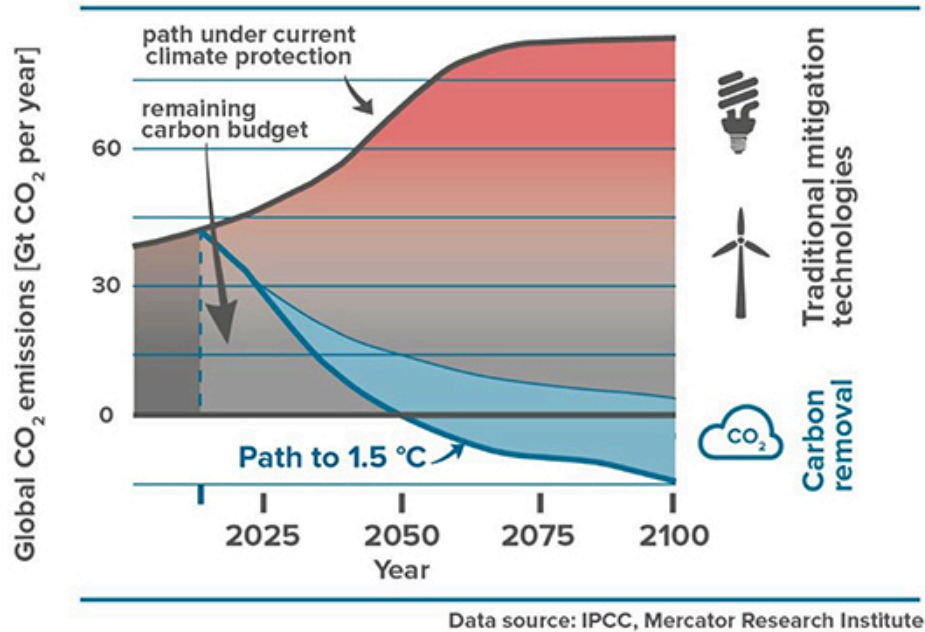
Figure 2. Global CO 2 Emissions Reduction Scenarios (IPCC, 2018)
