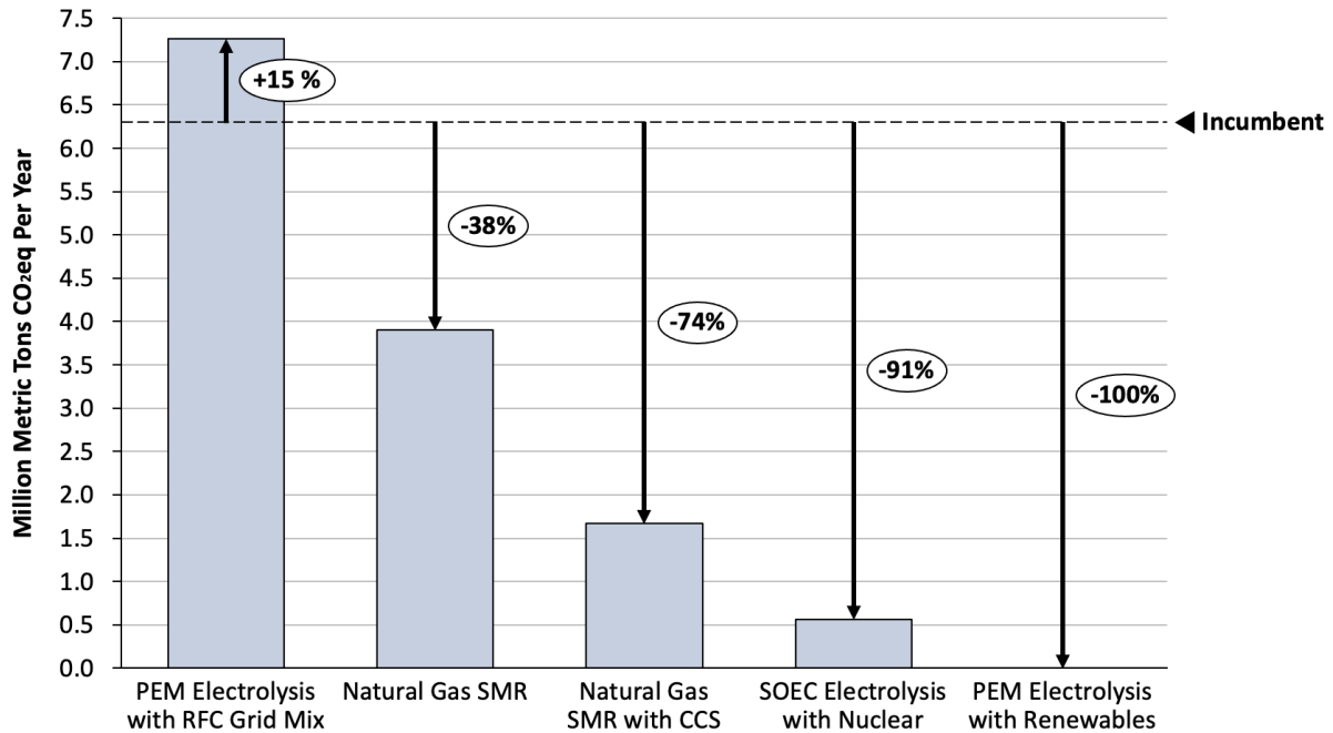
Figure 17. Total GHG emissions for the “Complete Hydrogen Substitution” scenario compared to “Incumbent Technology” scenario emissions (dashed line) in transportation.
