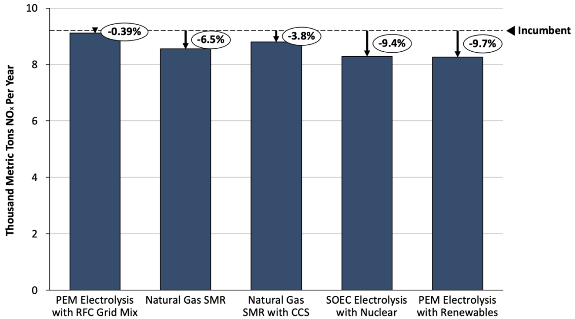
Figure 6. Total NO x emissions for the “Near-Term Opportunities” scenario compared to “Incumbent Technology” scenario emissions (dashed line) in industry.
