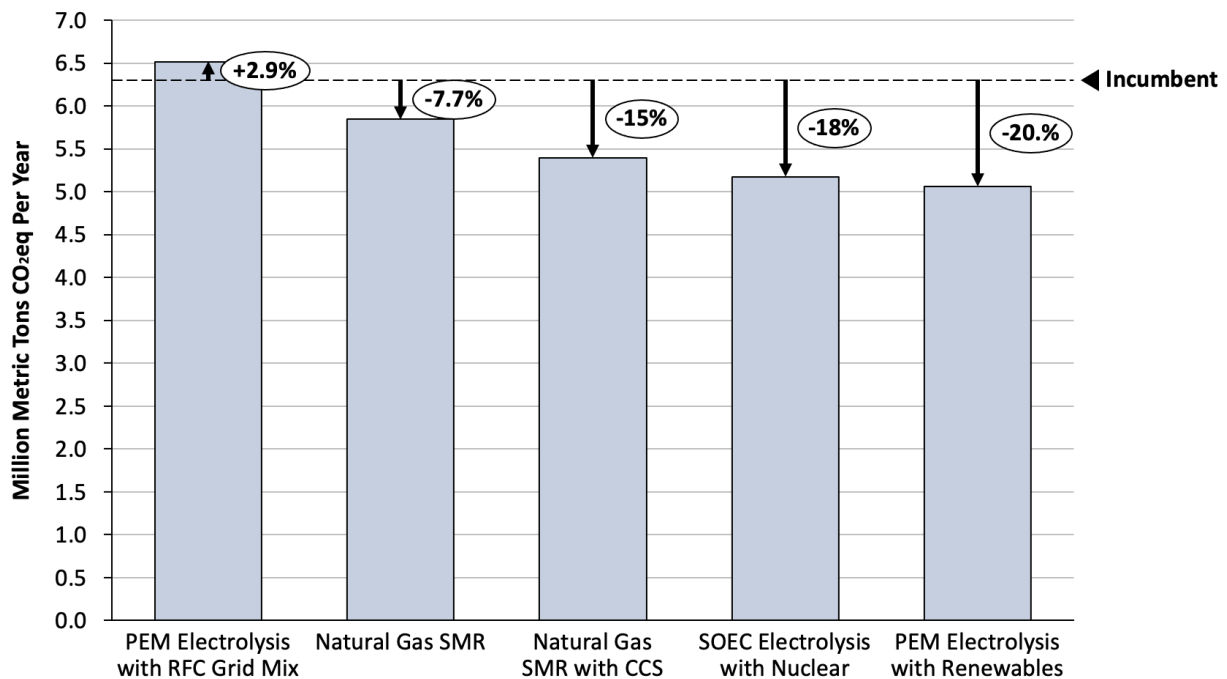
Figure 11. Total GHG emissions for the “2050 High Hydrogen Use” scenario compared to “Incumbent Technology” scenario emissions (dashed line) in transportation.
