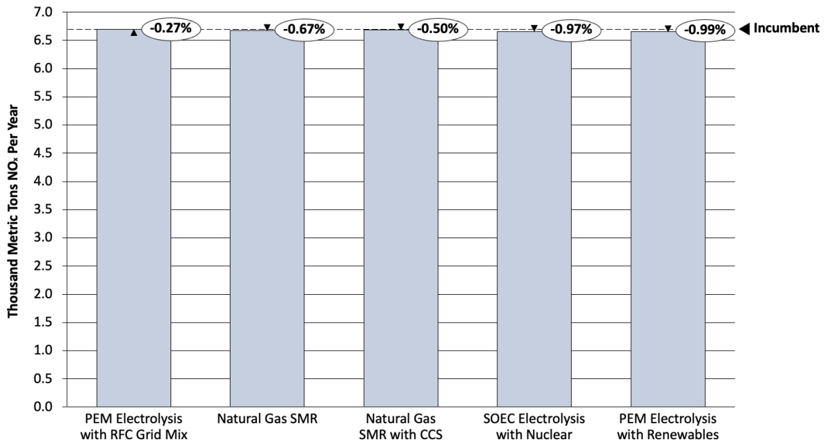
Figure 5. Total NO x emissions for the “Near-Term Opportunities” scenario compared to “Incumbent Technology” scenario emissions (dashed line) in transportation.
