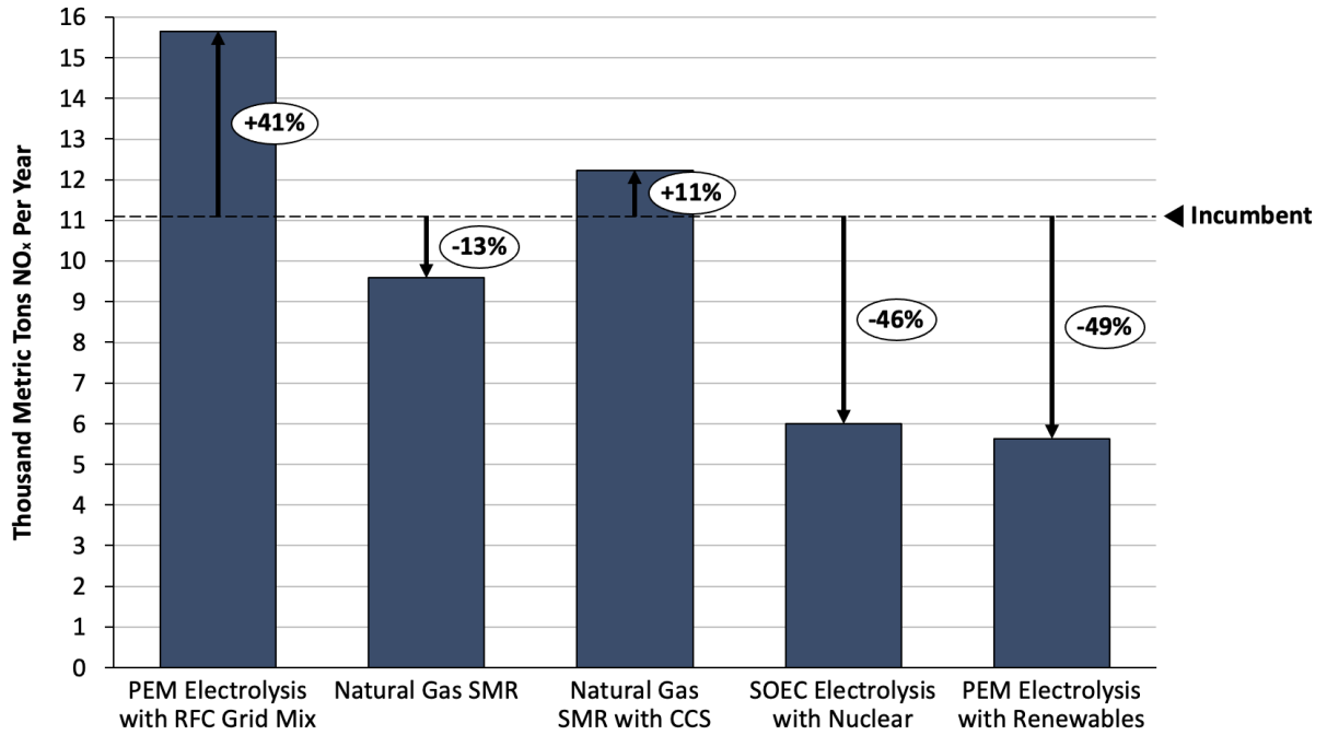
Figure 20. Total NO x emissions for the “Complete Hydrogen Substitution” scenario compared to “Incumbent Technology” scenario emissions (dashed line) in industry.
