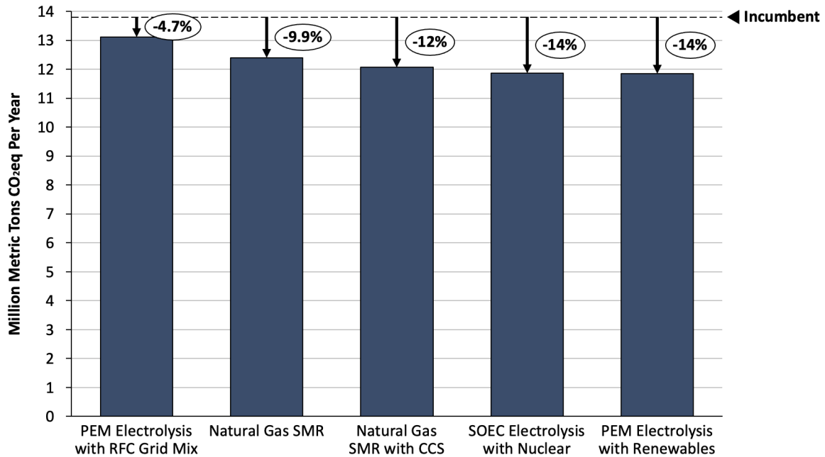
Figure 4. Total GHG emissions for the “Near-Term Opportunities” scenario compared to “Incumbent Technology” scenario emissions (dashed line) in industry. Due to rounding, the emission reduction potentials appear to be the same for SOEC electrolysis with nuclear and PEM electrolysis with renewables. However, PEM electrolysis with renewables leads to a slightly higher emission reduction.
