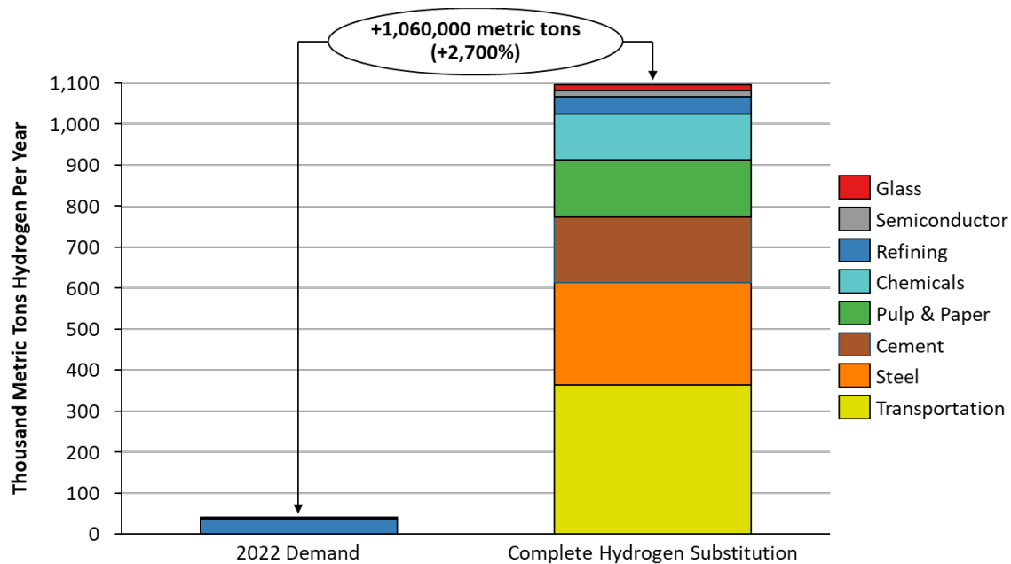
Figure 8. Long-term (2050) potential hydrogen demand in the “Complete Hydrogen Substitution” scenario as compared to current (2022) hydrogen demand.
