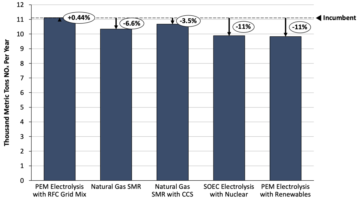
Figure 13. Total NO x emissions for the “2050 Low Hydrogen Use” scenario compared to “Incumbent Technology” scenario emissions (dashed line) in transportation.
