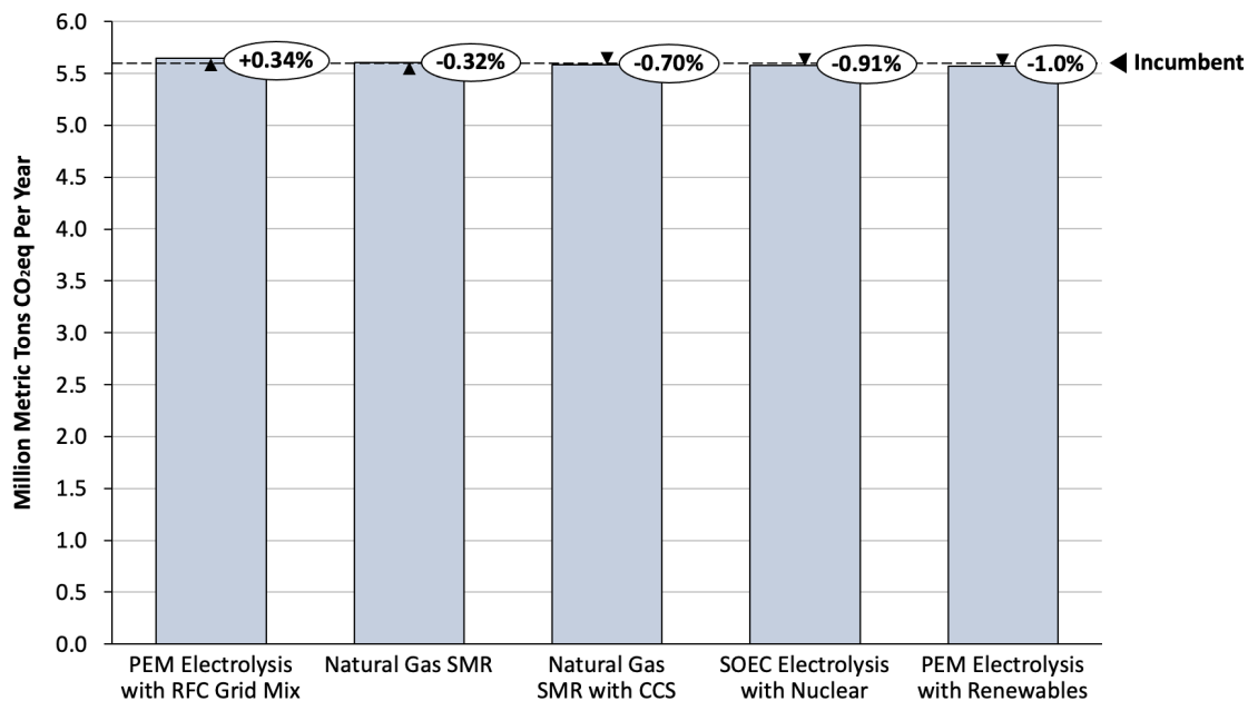
Figure 3. Total GHG emissions for the “Near-Term Opportunities” scenario compared to “Incumbent Technology” scenario emissions (dashed line) in transportation.
