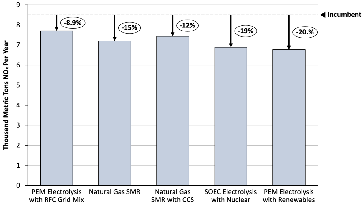
Figure 15. Total NO x emissions for the “2050 High Hydrogen Use” scenario compared to “Incumbent Technology” scenario emissions (dashed line) in transportation.
