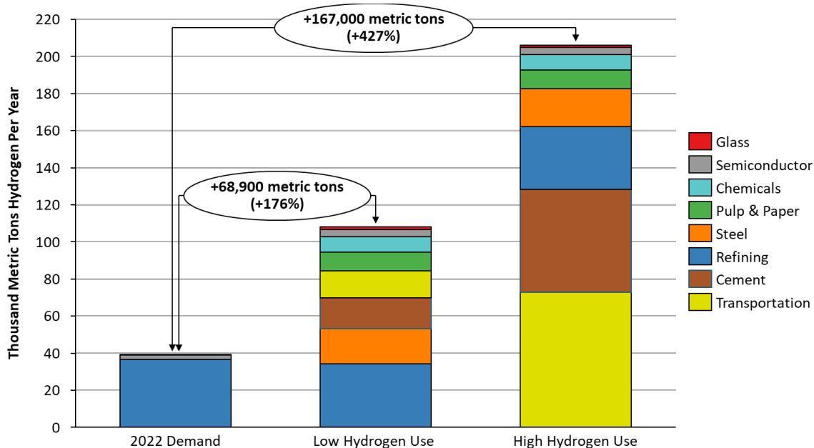
Figure 7. Long-term (2050) potential hydrogen demand in the “Low Hydrogen Use” and “High Hydrogen Use” scenarios as compared to current (2022) hydrogen demand.
