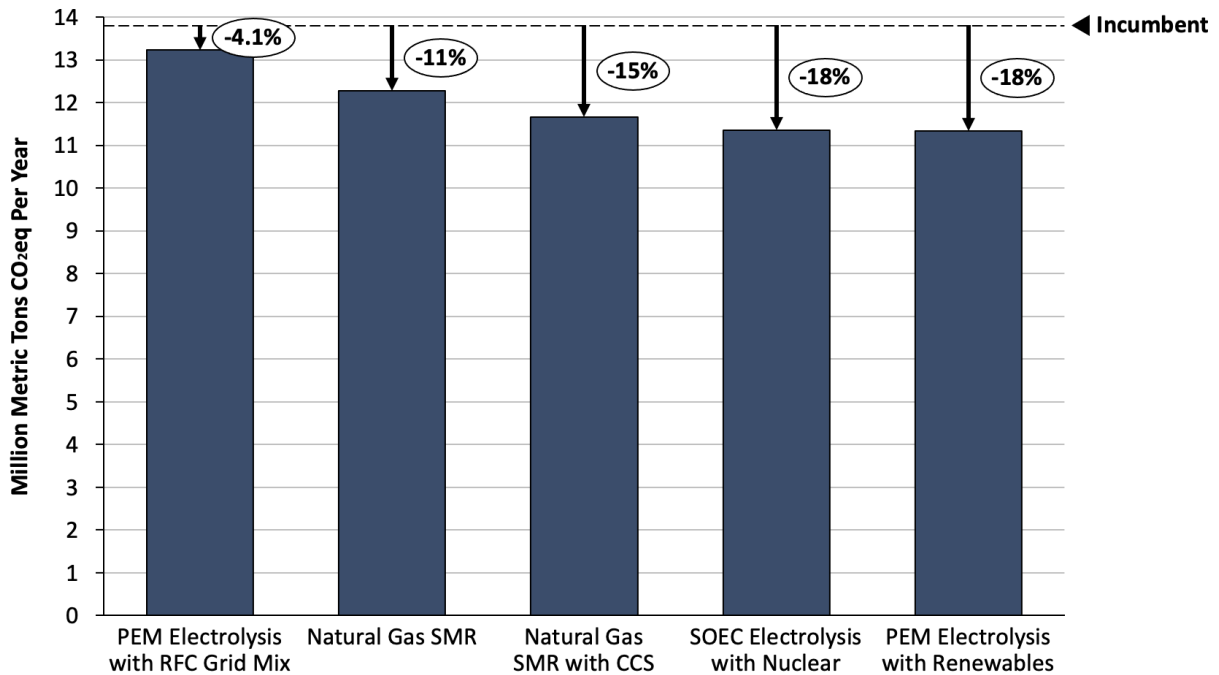
Figure 10. Total GHG emissions for the “2050 Low Hydrogen Use” scenario compared to “Incumbent Technology” scenario emissions (dashed line) in industry. Due to rounding, the emissions reduction potentials appear to be the same for SOEC electrolysis with nuclear and PEM electrolysis with renewables. However, PEM electrolysis with renewables leads to a slightly higher emissions reduction.
