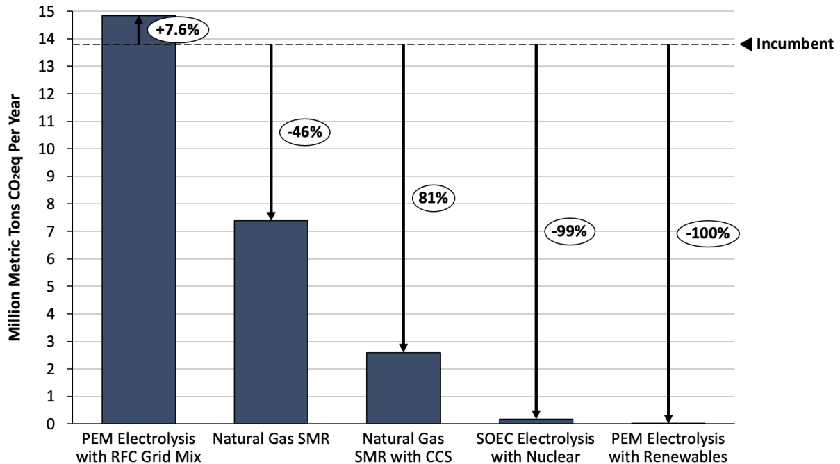
Figure 18. Total GHG emissions for the “Complete Hydrogen Substitution” scenario compared to “Incumbent Technology” scenario emissions (dashed line) in industry. Though the emissions reduction potential from hydrogen produced via PEM electrolysis with renewables rounds to 100%, some GHG emissions remain from oxygen produced for oxy-fuel combustion in the glass sector.
