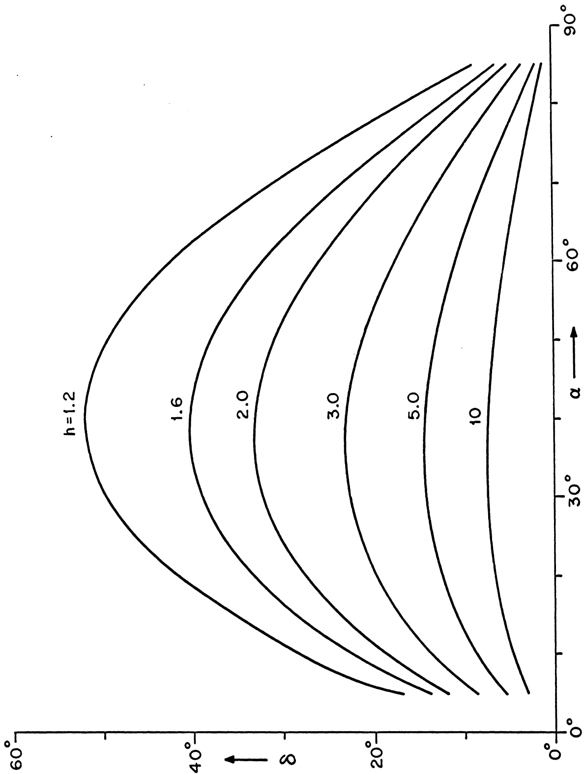
FIG. 2-6: DEVIATION ANGLE VS. ANGLE OF INCIDENCE
