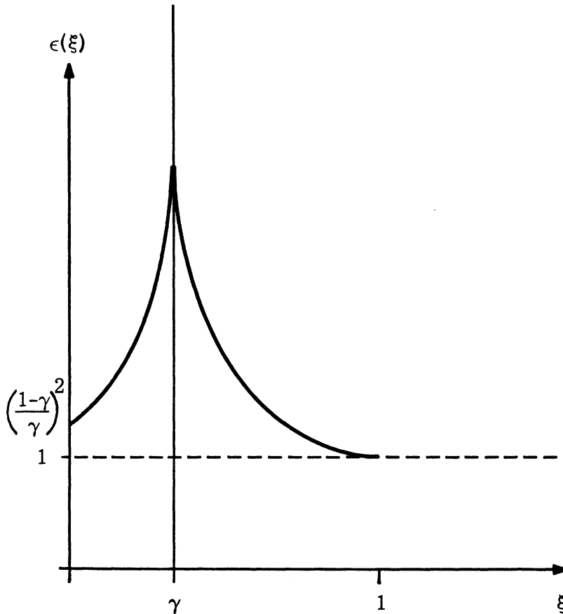
FIG. 2-1: Case 1: 0 \leq \gamma < 1
