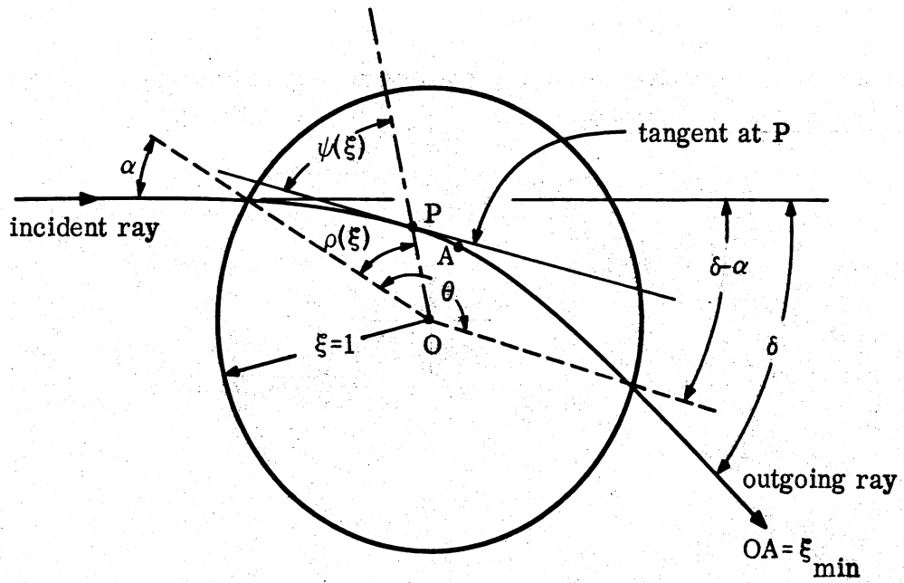
FIG. 2-4: RAY PATH THROUGH THE INHOMOGENEOUS DIELECTRIC:
