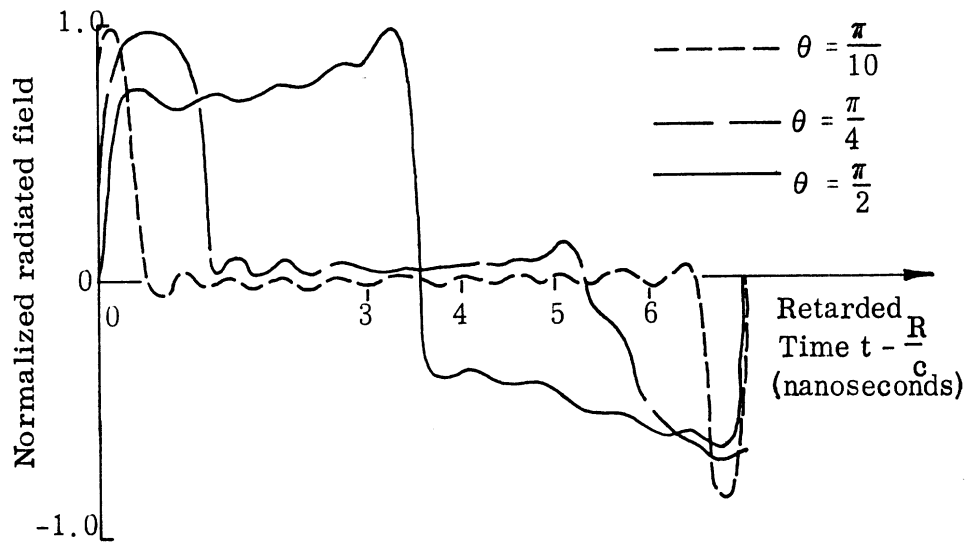
(A) Radiated Waveform for Step Function Input Current
