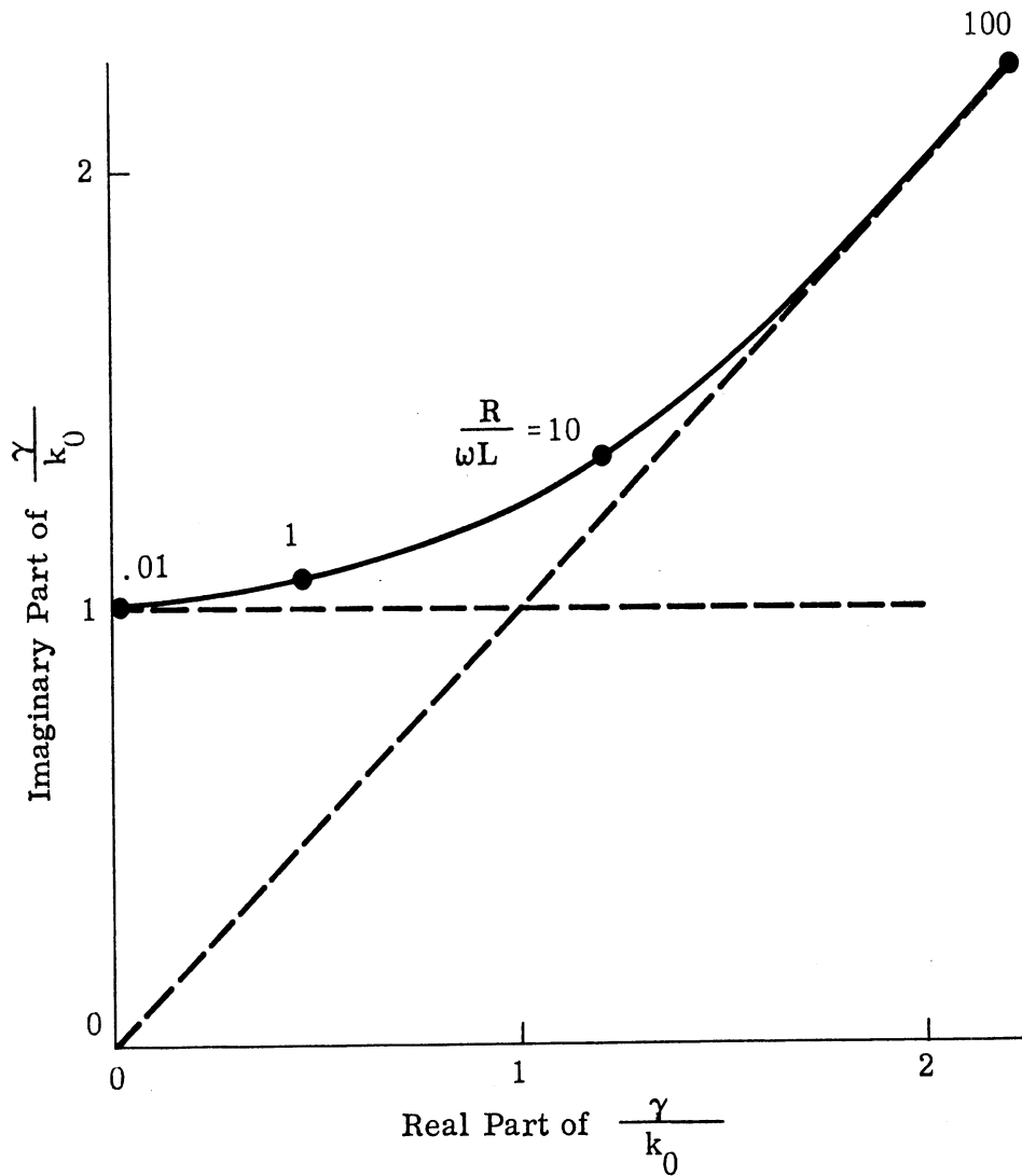
FIG. 2-2: COMPLEX PROPAGATION FACTOR \gamma FOR UNIFORM RESISTANCE-LOADED TRANSMISSION LINE.
