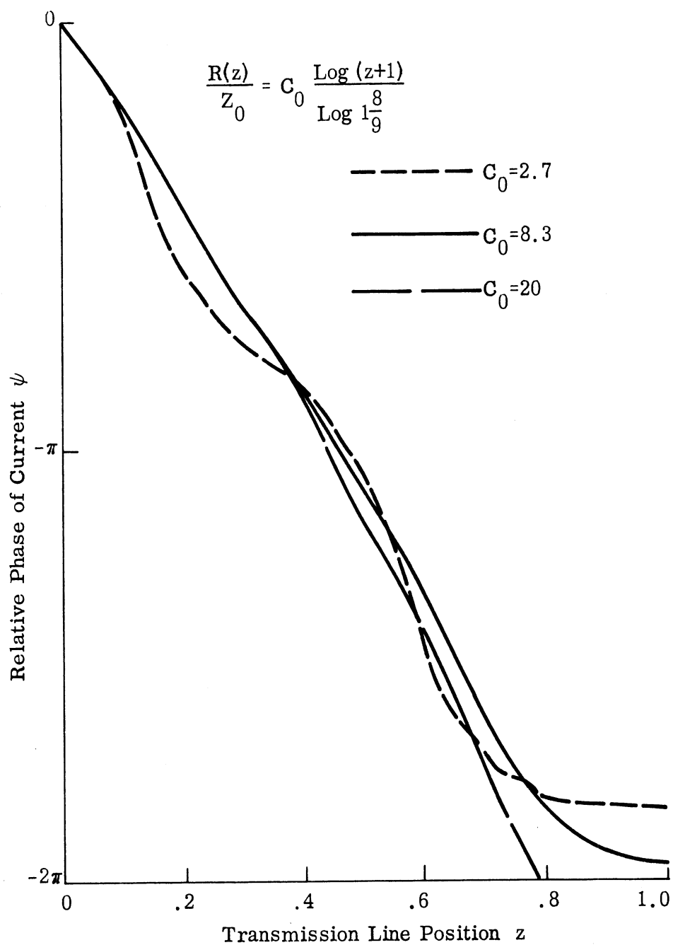
FIG. 2-7: PHASE OF CURRENT ALONG TRANSMISSION LINE PRODUCED BY CONTINUOUS LOGARITHMIC RESISTANCE LOADING.
