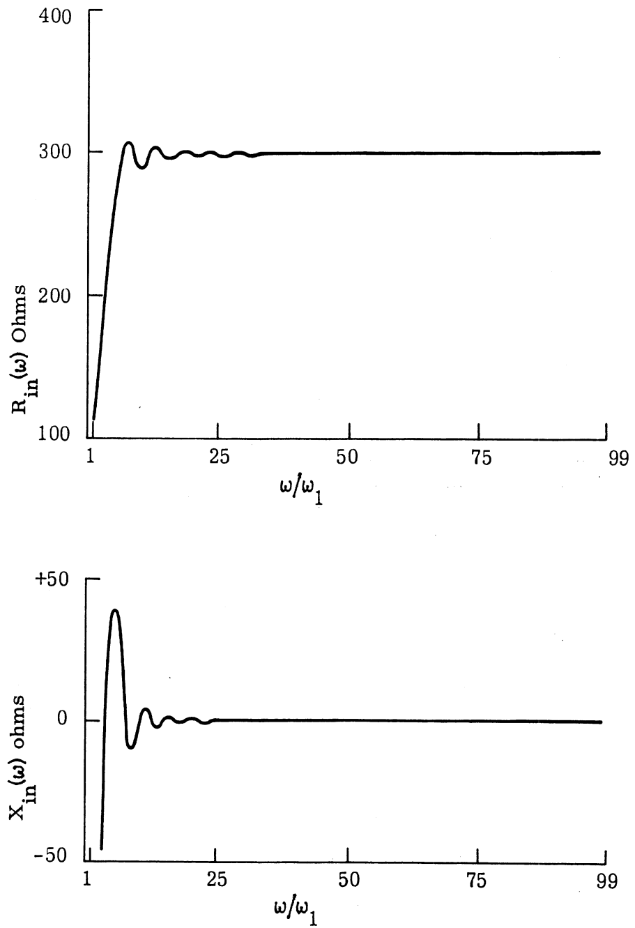
FIG. 2-45: INPUT IMPEDANCE VERSUS FREQUENCY FOR OPTIMUM RESISTANCE-LOADED TRANSMISSION LINE.
