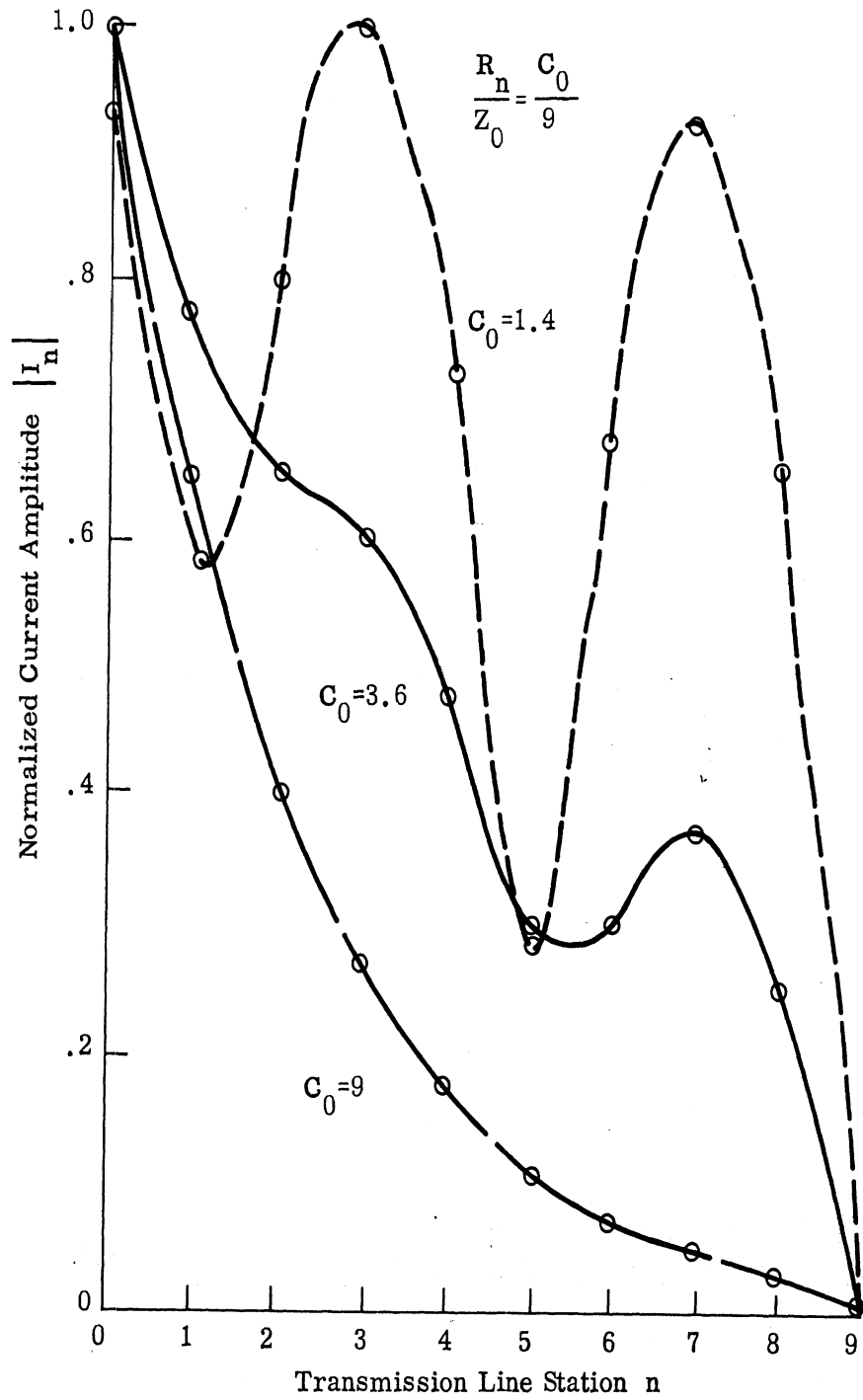
FIG. 2-24: AMPLITUDE OF CURRENT ALONG TRANSMISSION LINE PRODUCED BY DISCRETE UNIFORM RESISTANCE LOADING.
