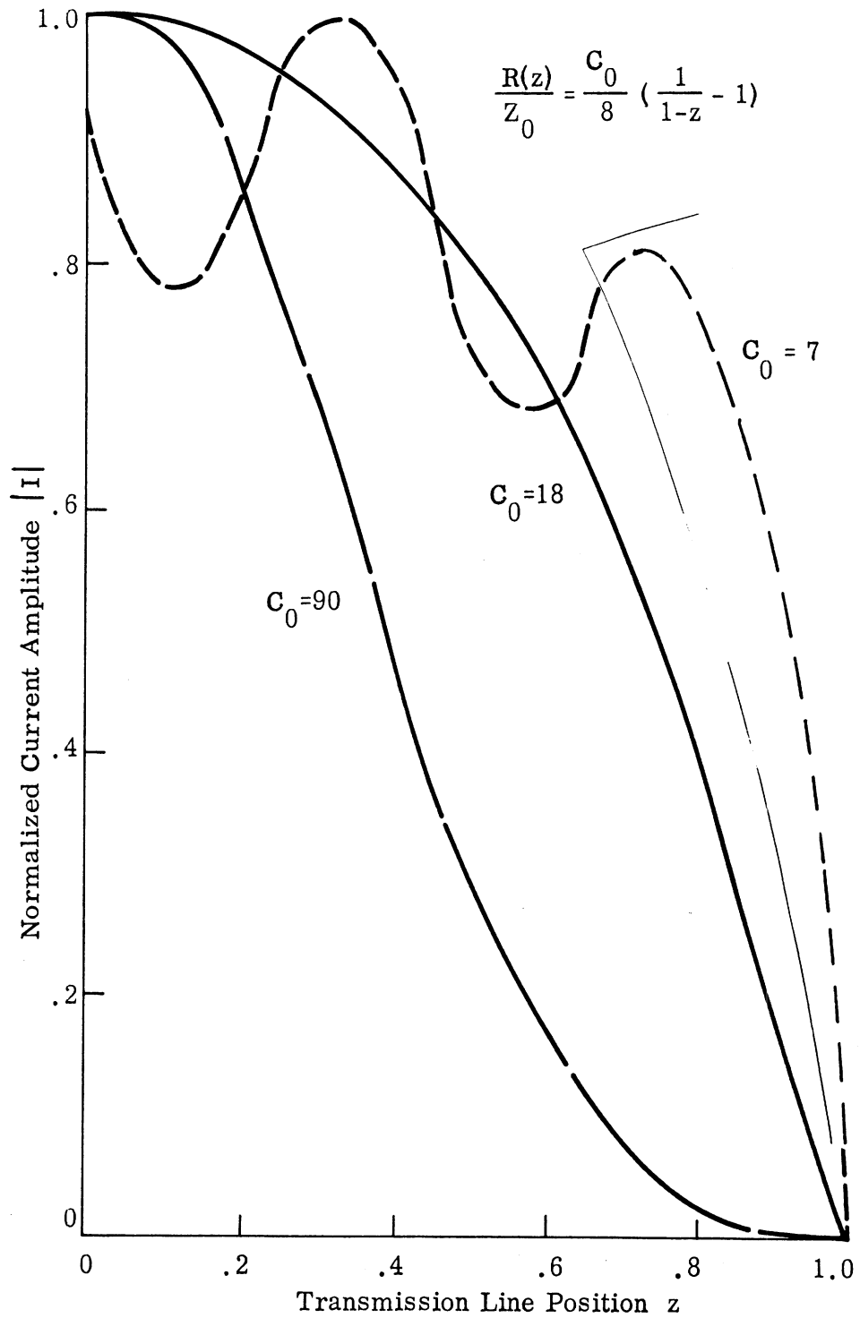
FIG. 2-10: AMPLITUDE OF CURRENT ALONG TRANSMISSION LINE PRODUCED BY CONTINUOUS INVERSE RESISTANCE LOADING.
