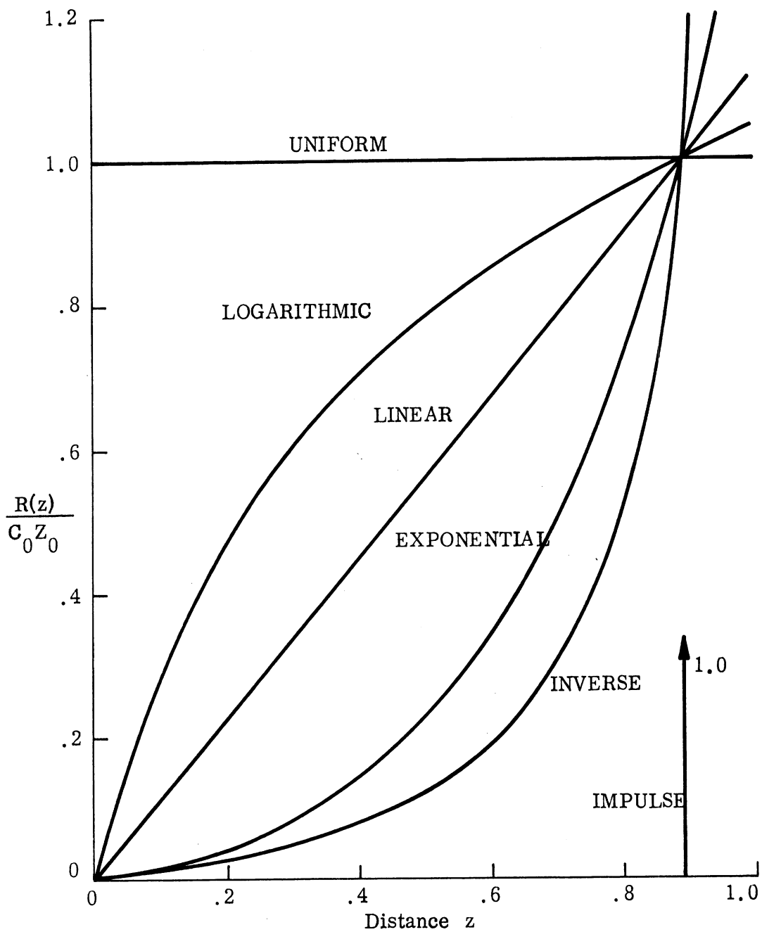
FIG. 2-3: NORMALIZED RESISTANCE DISTRIBUTIONS.
