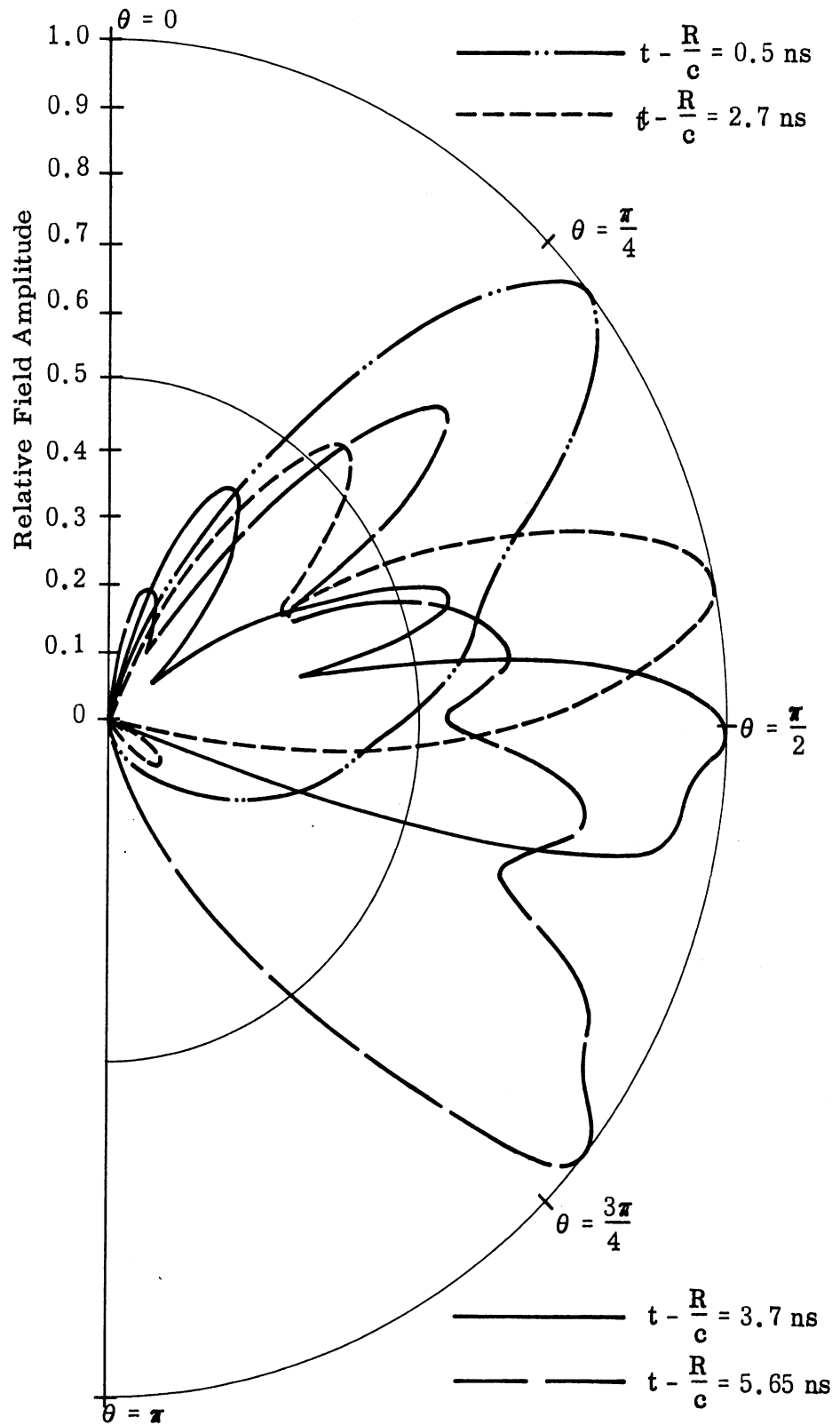
FIG. 2-52: TIME SEQUENCE OF RADIATION PATTERNS FOR OPTIMALLY LOADED TRANSMISSION LINE EXCITED BY APPROXIMATE STEP VOLTAGE.
