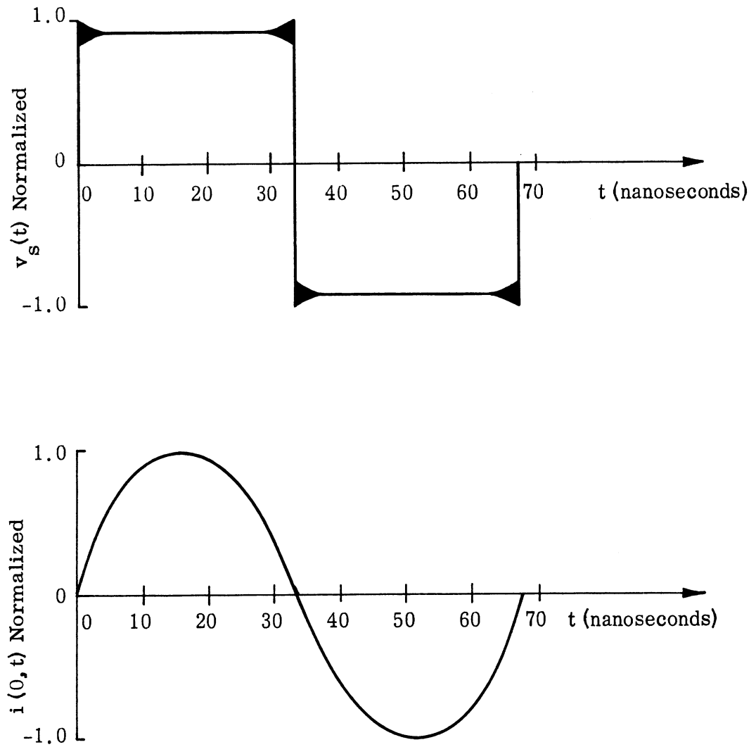
FIG. 3-3: TIME WAVEFORMS OF SOURCE VOLTAGE v_s(t) AND INPUT CURRENT i(0,t) OF BICONICAL ANTENNA.
