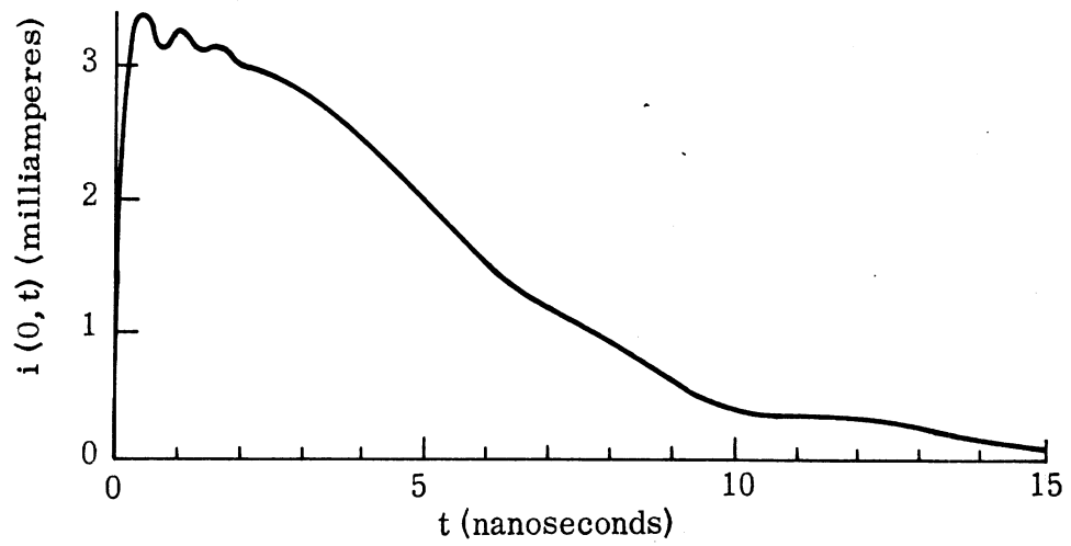
FIG. 2-47: TIME WAVEFORMS OF SOURCE VOLTAGE v_s(t) AND INPUT CURRENT i(0, t) . K = 50 .
