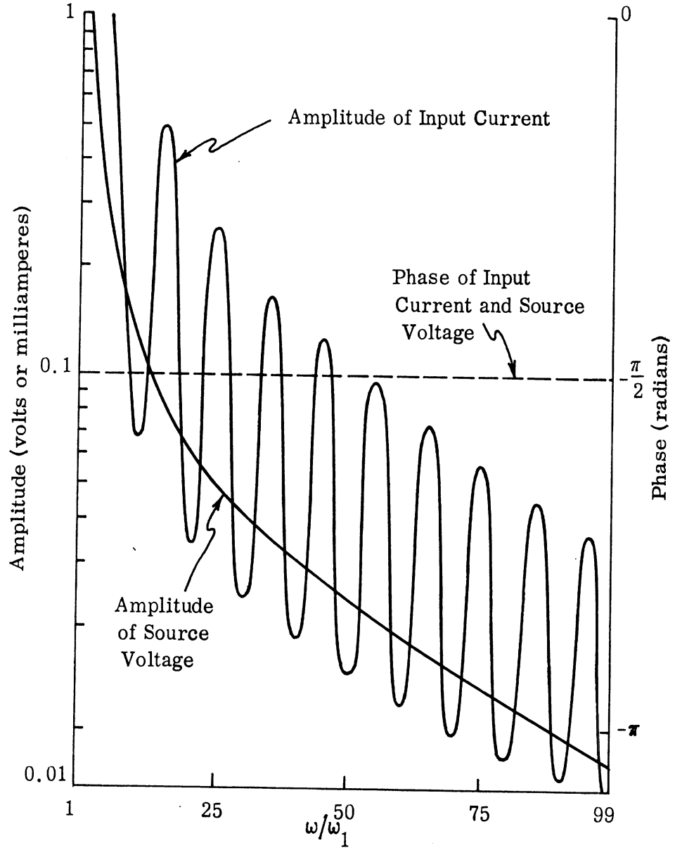
FIG. 3-2: FREQUENCY DOMAIN INPUT CURRENT OF BICONICAL ANTENNA, K = 50 .
