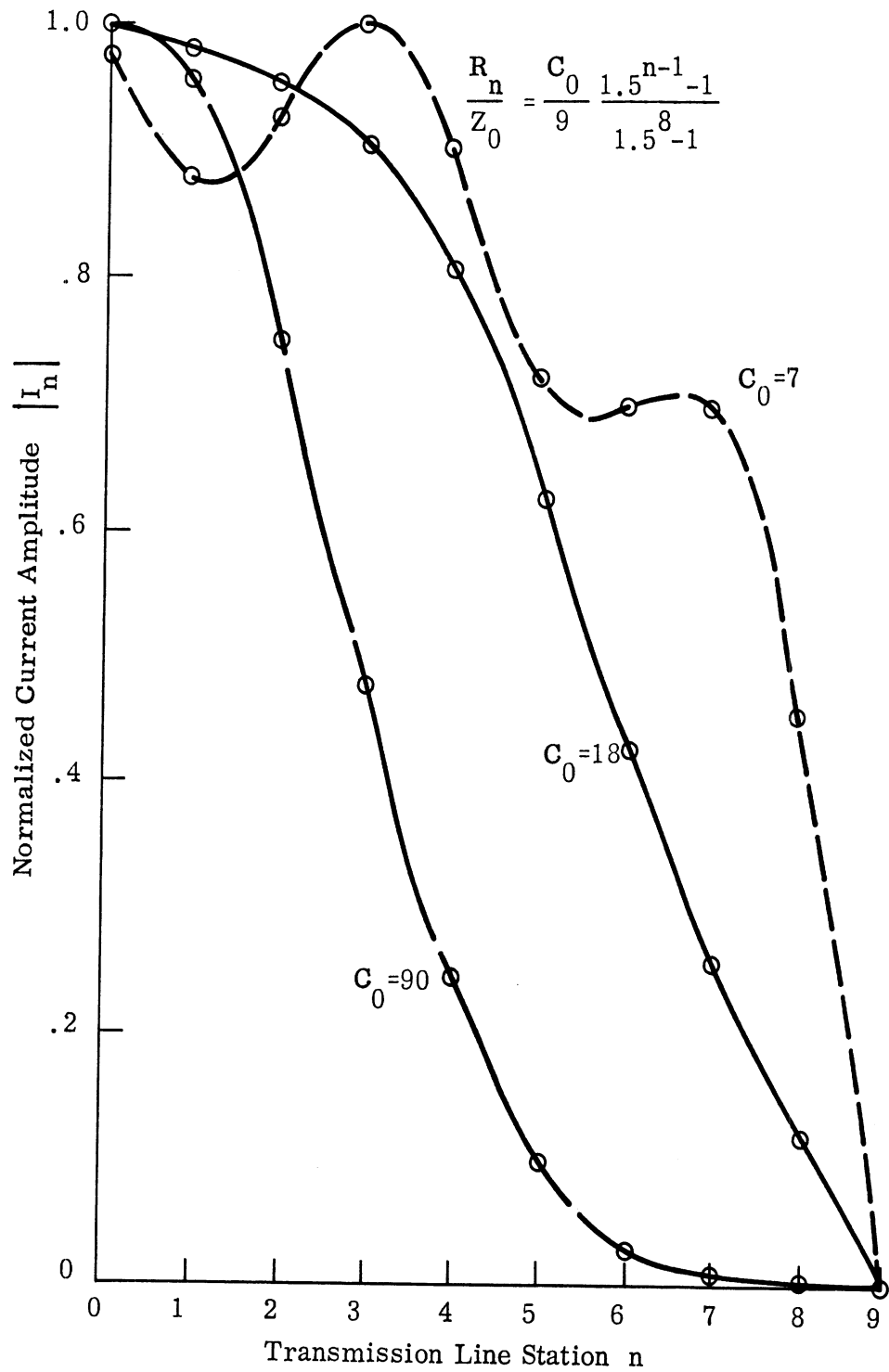
FIG. 2-32: AMPLITUDE OF CURRENT ALONG TRANSMISSION LINE PRODUCED BY DISCRETE EXPONENTIAL RESISTANCE LOADING.
