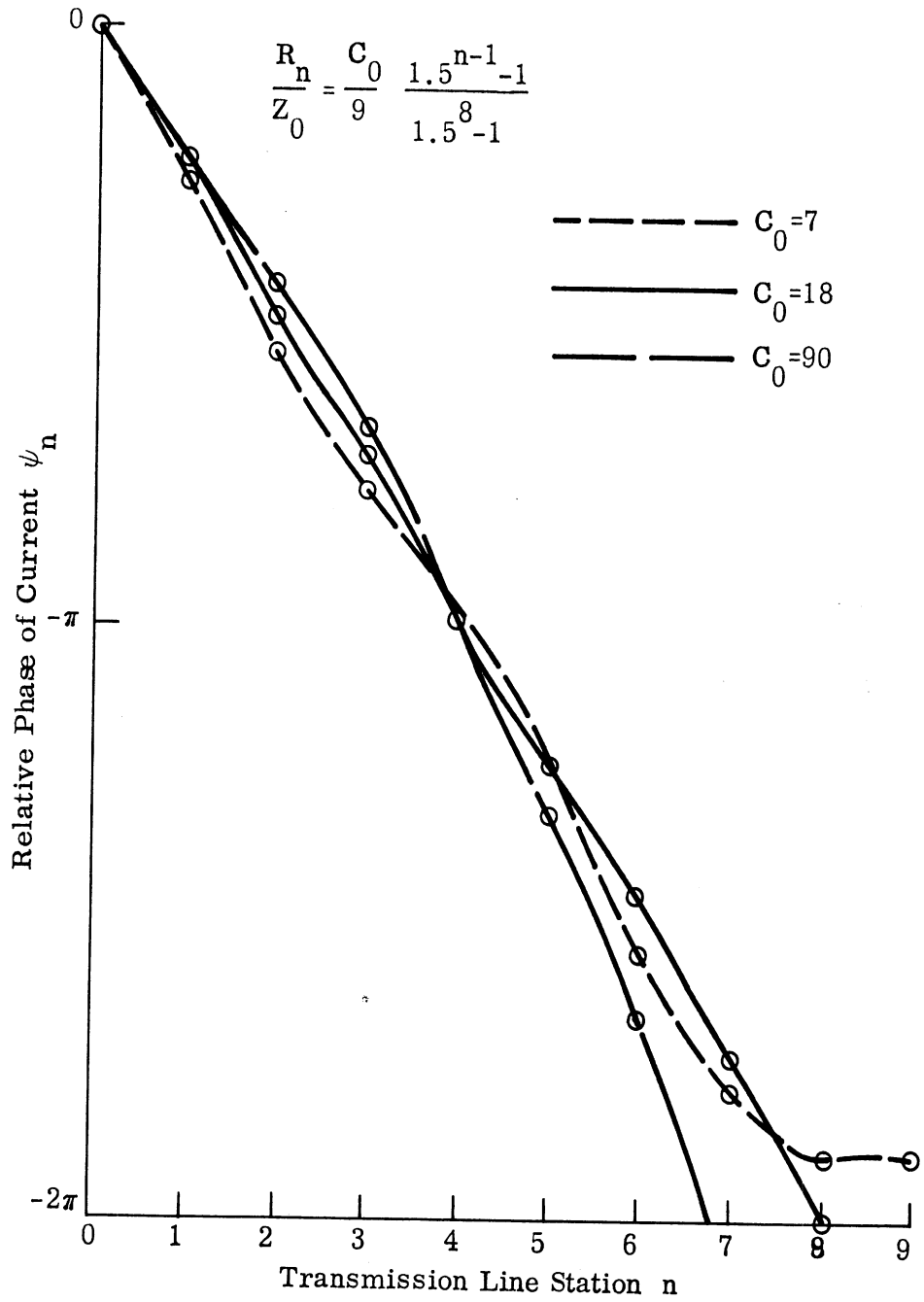
FIG. 2-33: PHASE OF CURRENT ALONG TRANSMISSION LINE PRODUCED BY DISCRETE EXPONENTIAL RESISTANCE LOADING.
