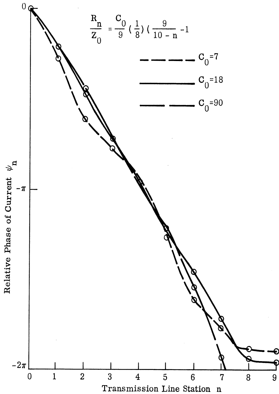
FIG. 2-31: PHASE OF CURRENT ALONG TRANSMISSION LINE PRODUCED BY DISCRETE INVERSE RESISTANCE LOADING.
