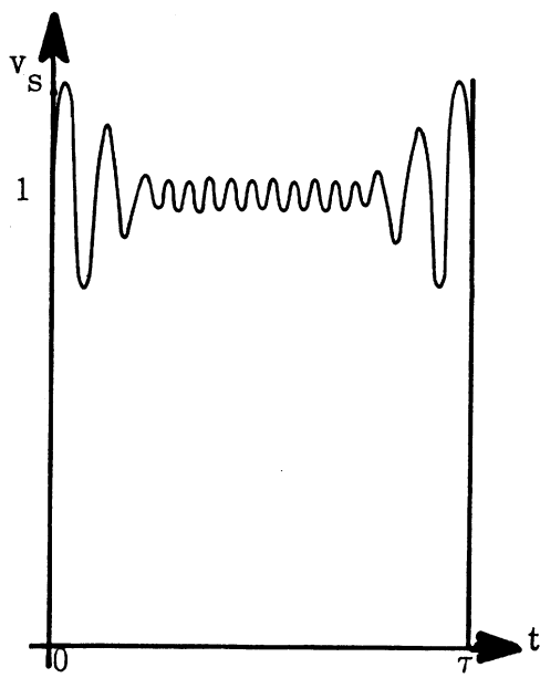
(B) 25-Term Approximation to Square Wave.
