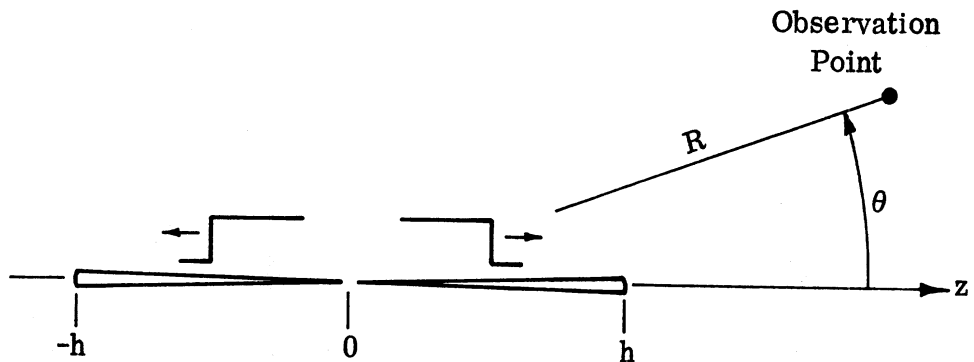
(A) Initial Outward Traveling Waves \bar{i}_+(z, t) .
