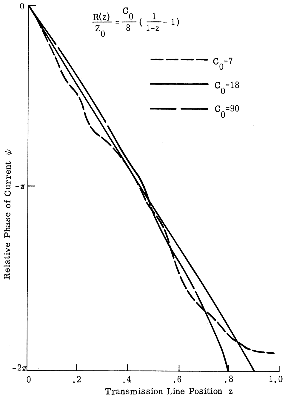
FIG. 2-11: PHASE OF CURRENT ALONG TRANSMISSION LINE PRODUCED BY CONTINUOUS INVERSE RESISTANCE LOADING.
