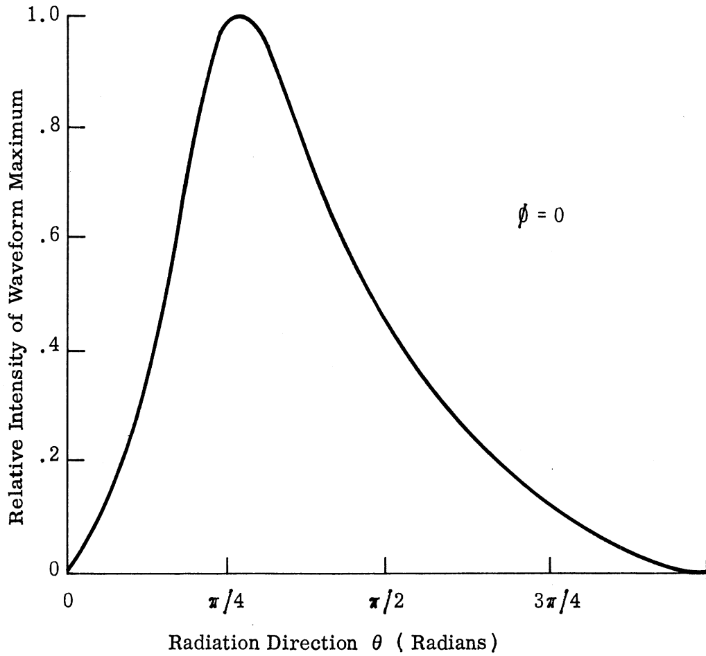
FIG. 2-51: MAXIMUM AMPLITUDE OF RADIATED TRANSIENT WAVEFORM AS A FUNCTION OF RADIATION DIRECTION.
