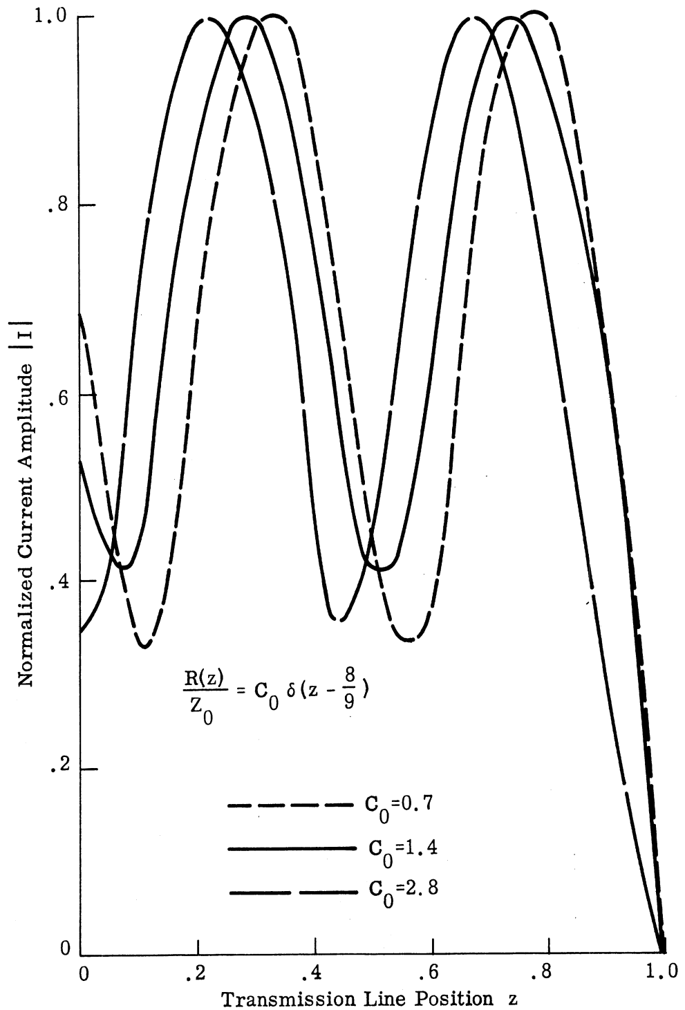
FIG. 2-14: AMPLITUDE OF CURRENT ALONG TRANSMISSION LINE PRODUCED BY CONTINUOUS IMPULSE RESISTANCE LOADING.
