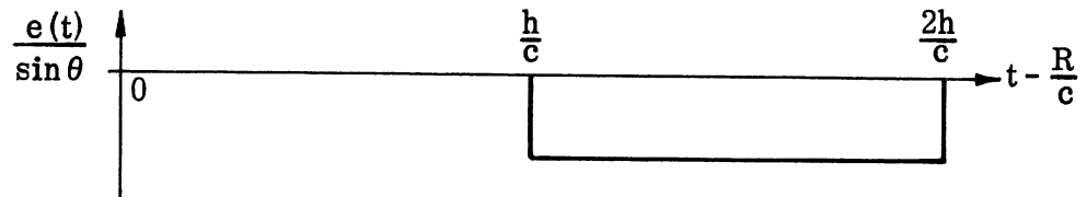
(C) Radiation from Current Step Traveling Inward on +z.
