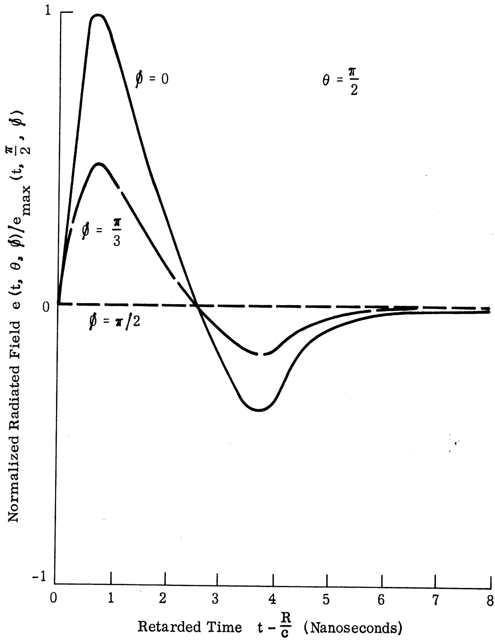
FIG. 2-53: TRANSIENT TIME WAVEFORMS RADIATED IN VARIOUS BROADSIDE DIRECTIONS FROM STEP-EXCITED TRANSMISSION LINE WITH OPTIMUM RESISTANCE LOADING.
