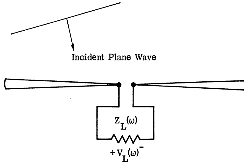
(A) Antenna with Load Impedance.
