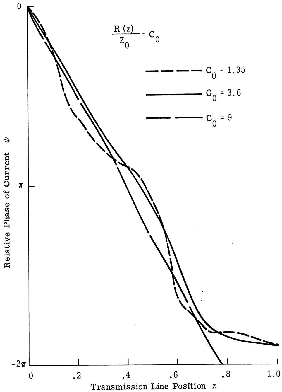
FIG. 2-5: PHASE OF CURRENT ALONG TRANSMISSION LINE PRODUCED BY CONTINUOUS UNIFORM RESISTANCE LOADING.
