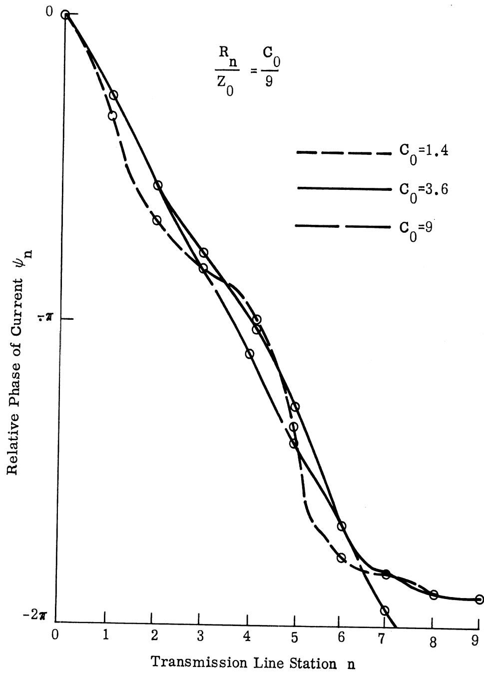
FIG. 2-25: PHASE OF CURRENT ALONG TRANSMISSION LINE PRODUCED BY DISCRETE UNIFORM RESISTANCE LOADING.
