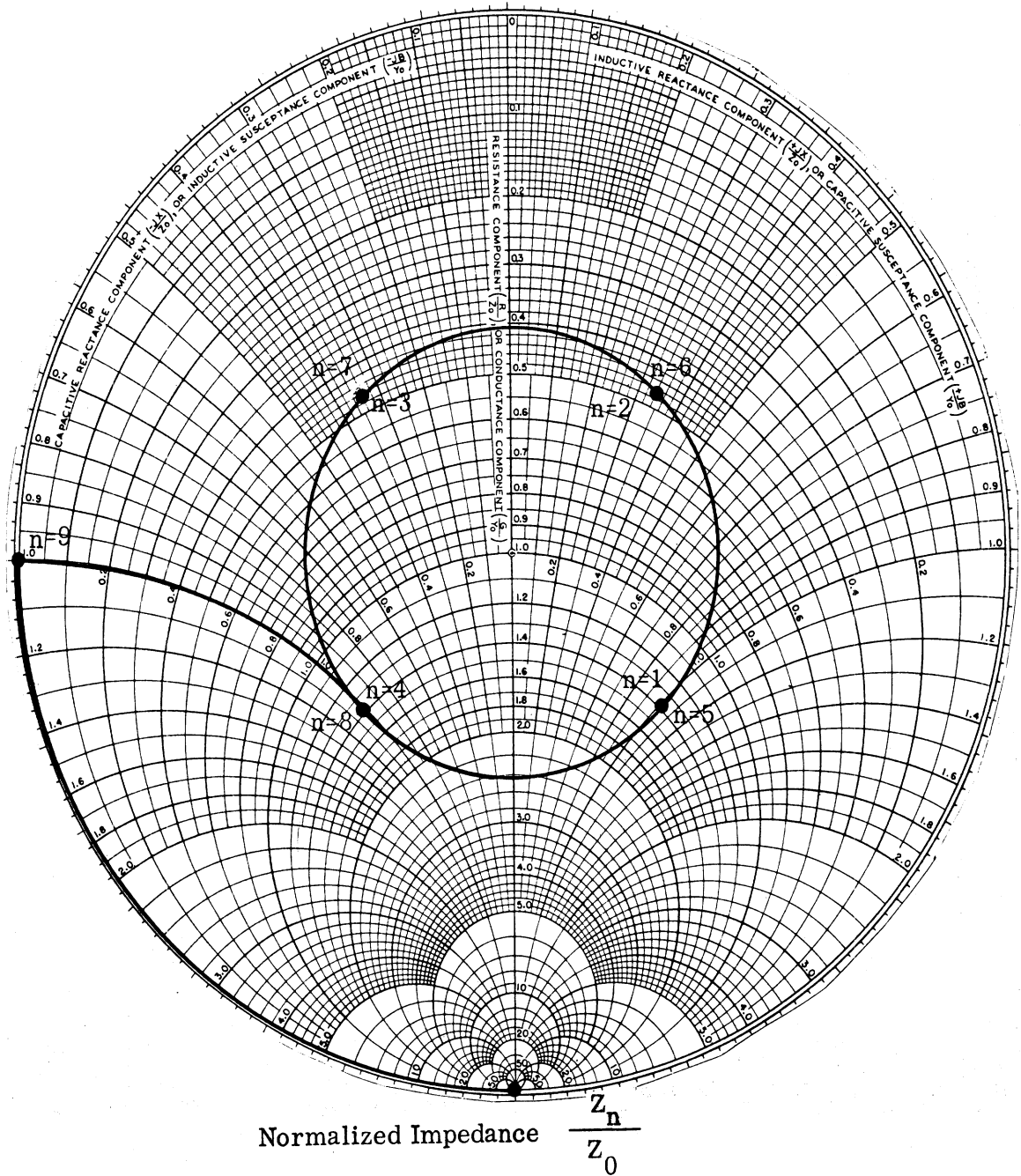
FIG. 2-41: IMPEDANCES ALONG TRANSMISSION LINE WITH IMPULSE DISCRETE RESISTANCE LOADING
