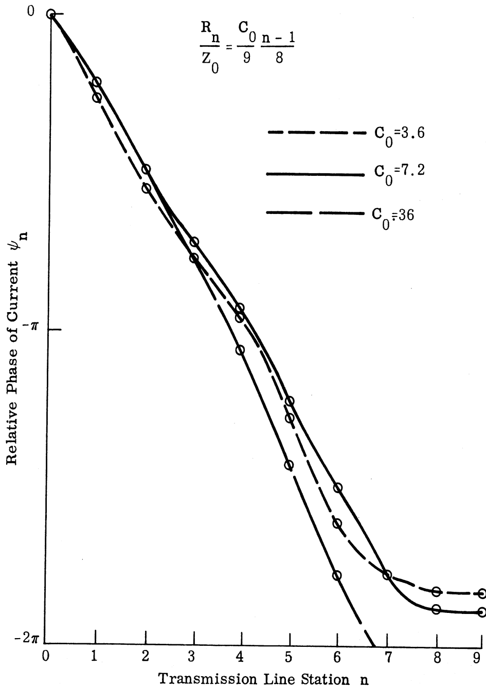
FIG. 2-29: PHASE OF CURRENT ALONG TRANSMISSION LINE PRODUCED BY DISCRETE LINEAR RESISTANCE LOADING.
