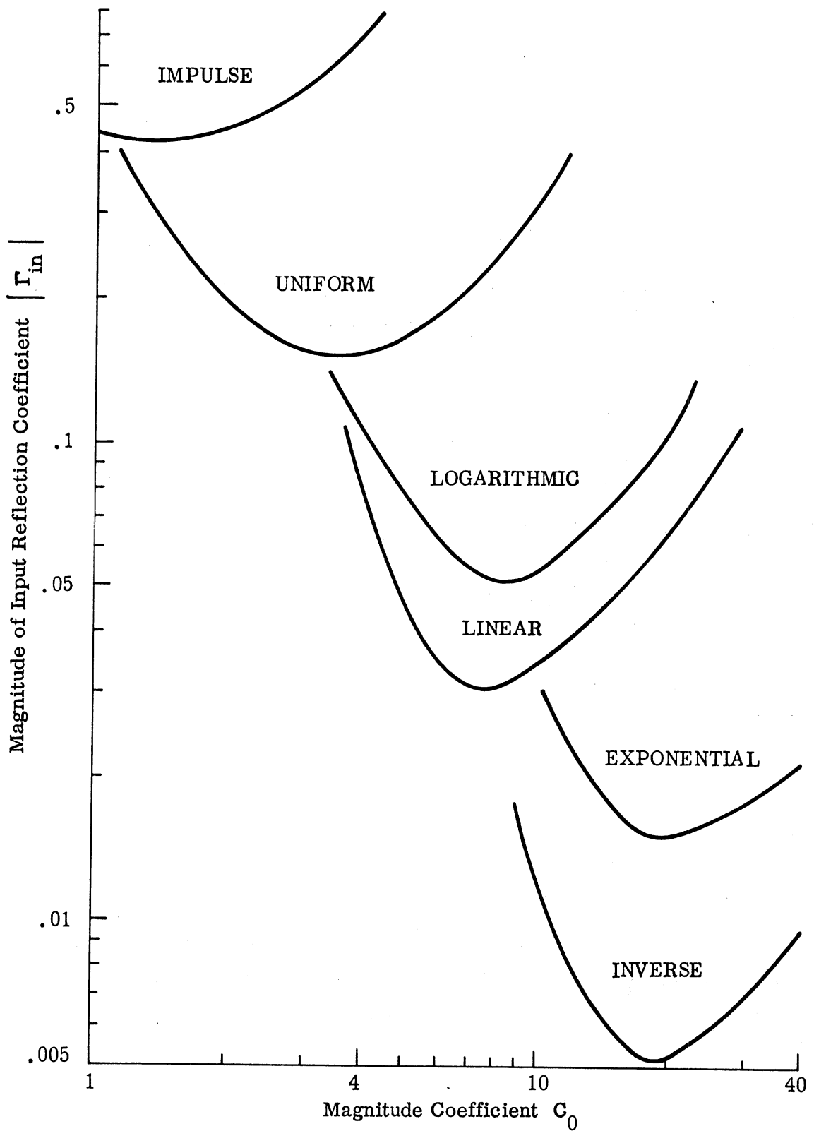
FIG. 2-22: INPUT REFLECTION COEFFICIENTS PRODUCED BY VARIOUS CONTINUOUS RESISTANCE DISTRIBUTIONS.
