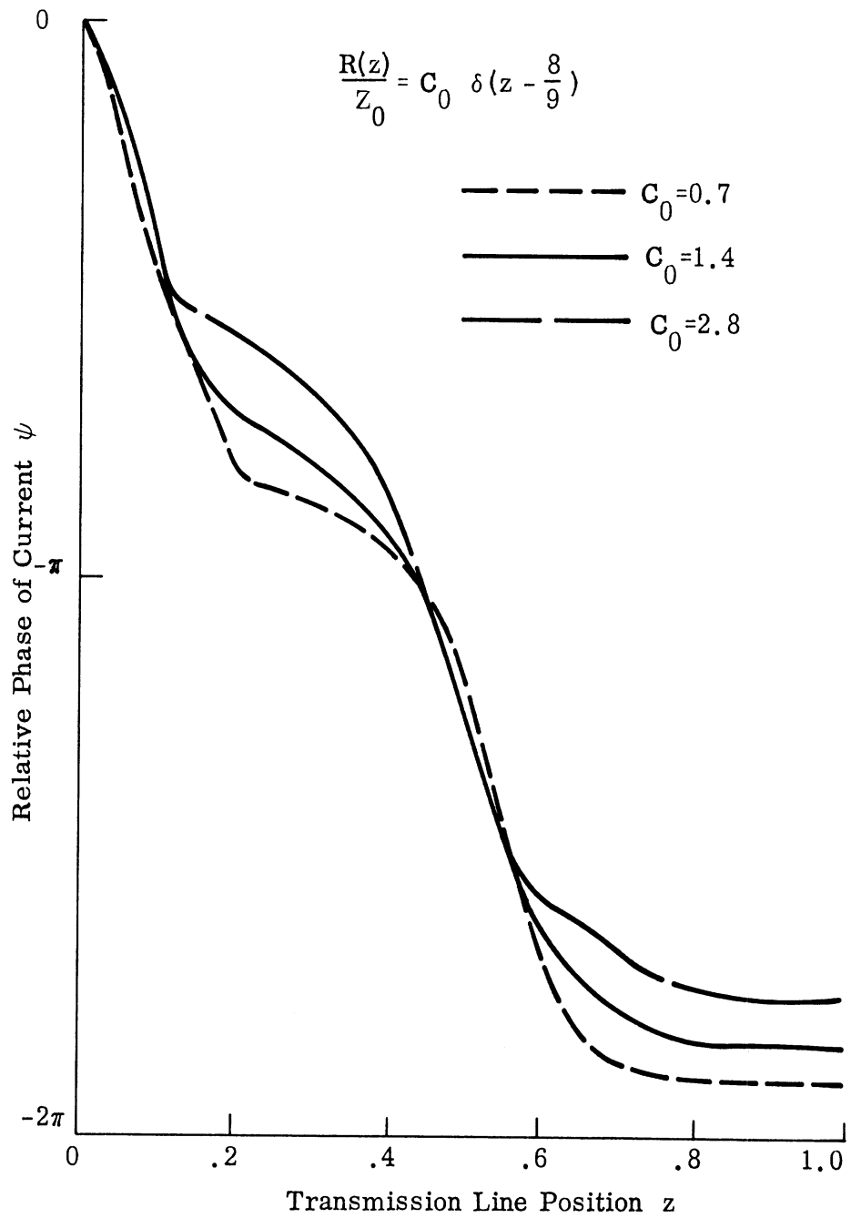
FIG. 2-15: PHASE OF CURRENT ALONG TRANSMISSION LINE PRODUCED BY CONTINUOUS IMPULSE RESISTANCE LOADING.
