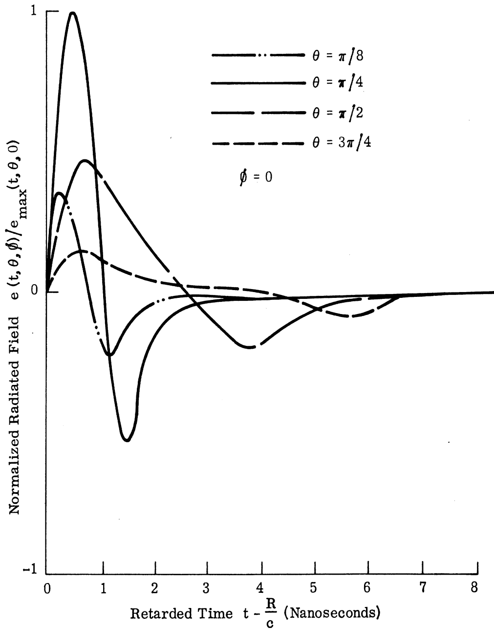
FIG. 2-50: TRANSIENT TIME WAVEFORMS RADIATED IN VARIOUS \theta DIRECTIONS FROM STEP-EXCITED TRANSMISSION LINE WITH OPTIMUM RESISTANCE LOADING.
