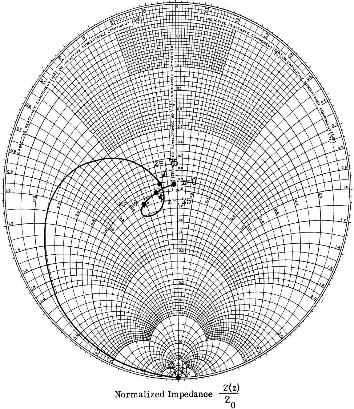
FIG. 2-17: IMPEDANCES ALONG TRANSMISSION LINE WITH LOGARITHMIC CONTINUOUS RESISTANCE LOADING \frac{R(z)}{Z_0} = 8.3 \frac{\log(z+1)}{\log 1 \frac{8}{9}} .
