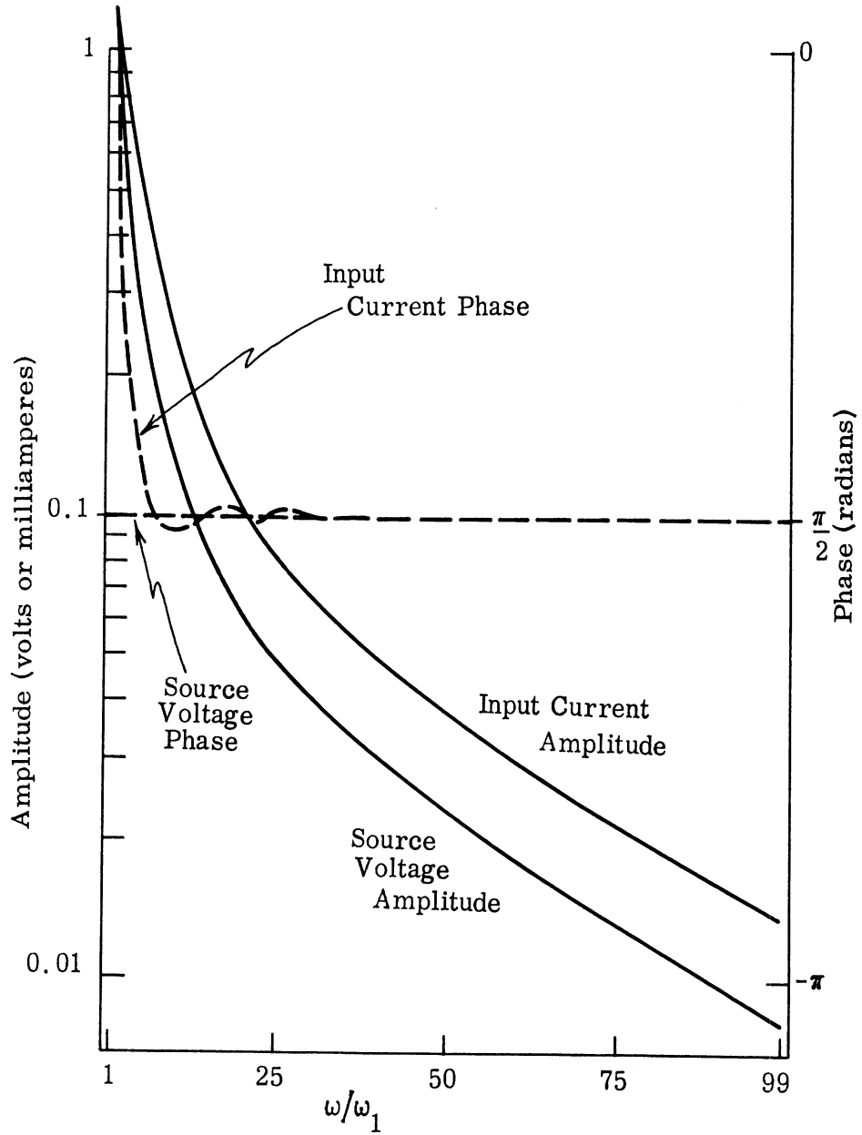
FIG. 2-46: FREQUENCY DOMAIN AMPLITUDE AND PHASE OF SOURCE VOLTAGE V_s(\omega) AND INPUT CURRENT I(0, \omega) . K = 50^S .
