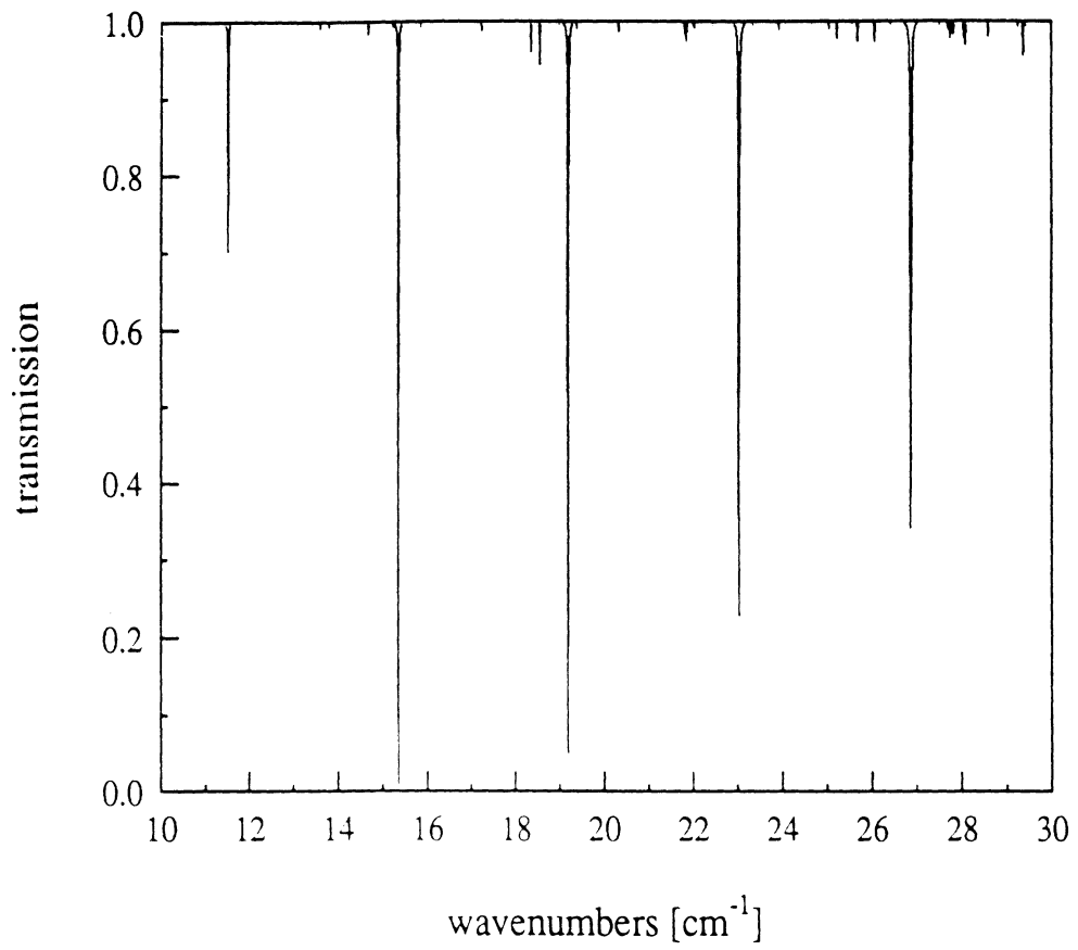
Figure (7.4): Far-infrared Transmission at Zenith for the Martian Northern Polar Region
