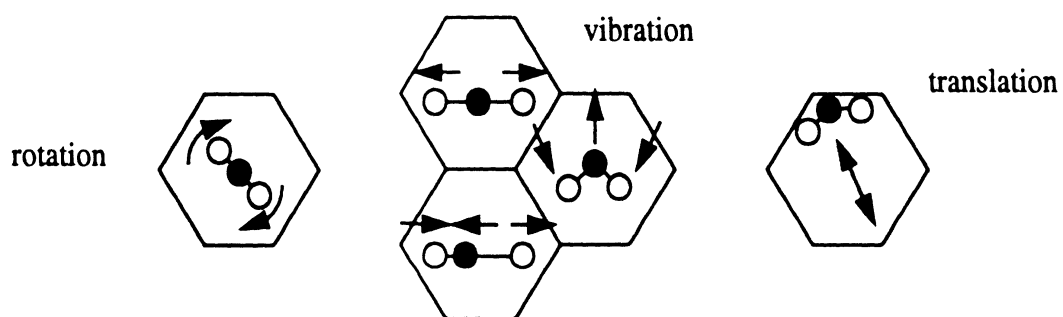
(c): CO 2 Guest Molecule Motion
