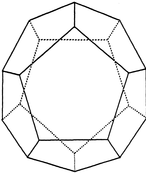
pentagonal dodecahedron
