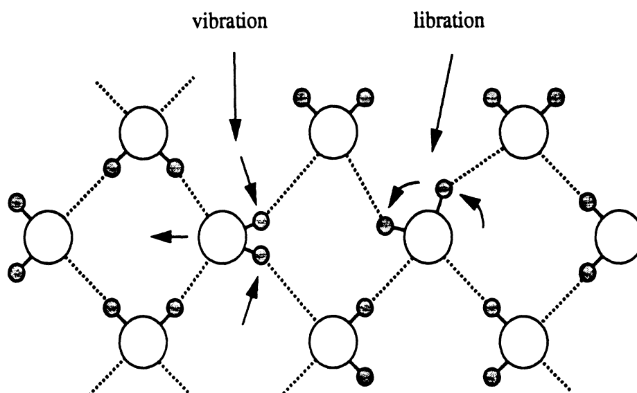
(b): Individual H 2 O molecule motion
