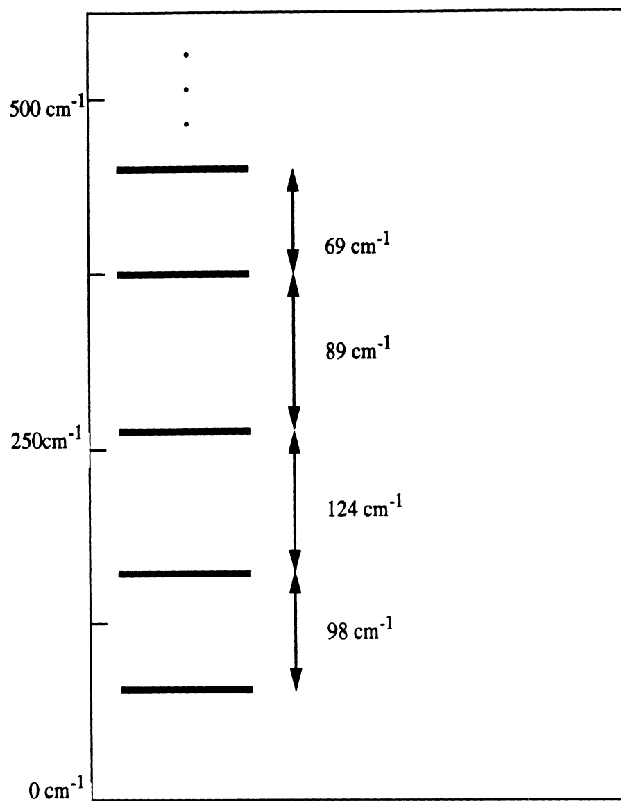
Figure (3.1): Energy Spectrum of the Translational Modes of the \text{CO}_2 Guest in the Smaller Structure I Cage
