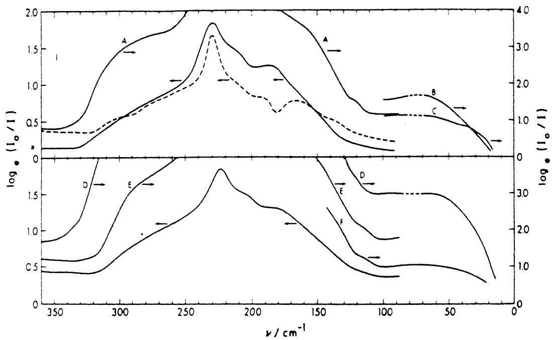
Figure (2.2): Lattice Mode Absorptions of Infrared Mulls (reproduced from Bertie and Othen, 1972). The solid lines are hydrate (top figure) and deuterate (bottom figure) of ethylene oxide. The dotted line is undeuterated water ice. Letters identify different mulls, with absorption scales indicated with arrows.
