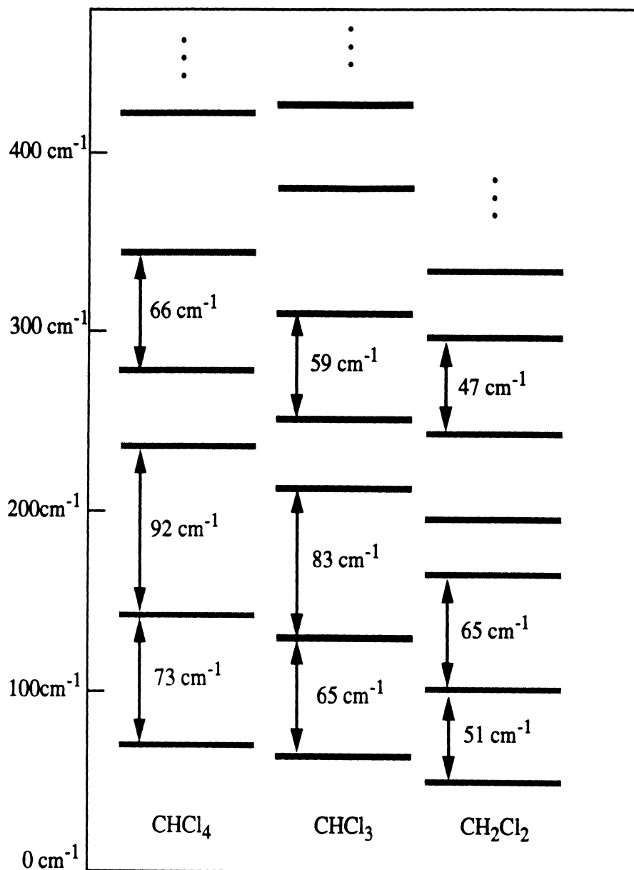
Figure (3.3): Energy Spectrum of the Translational Modes of CCl 4 , CHCl 3 , CH 2 Cl 2 Guests in the Larger Structure II Cage
