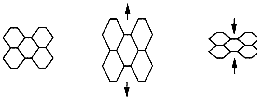
(a): Host Lattice Vibrations
