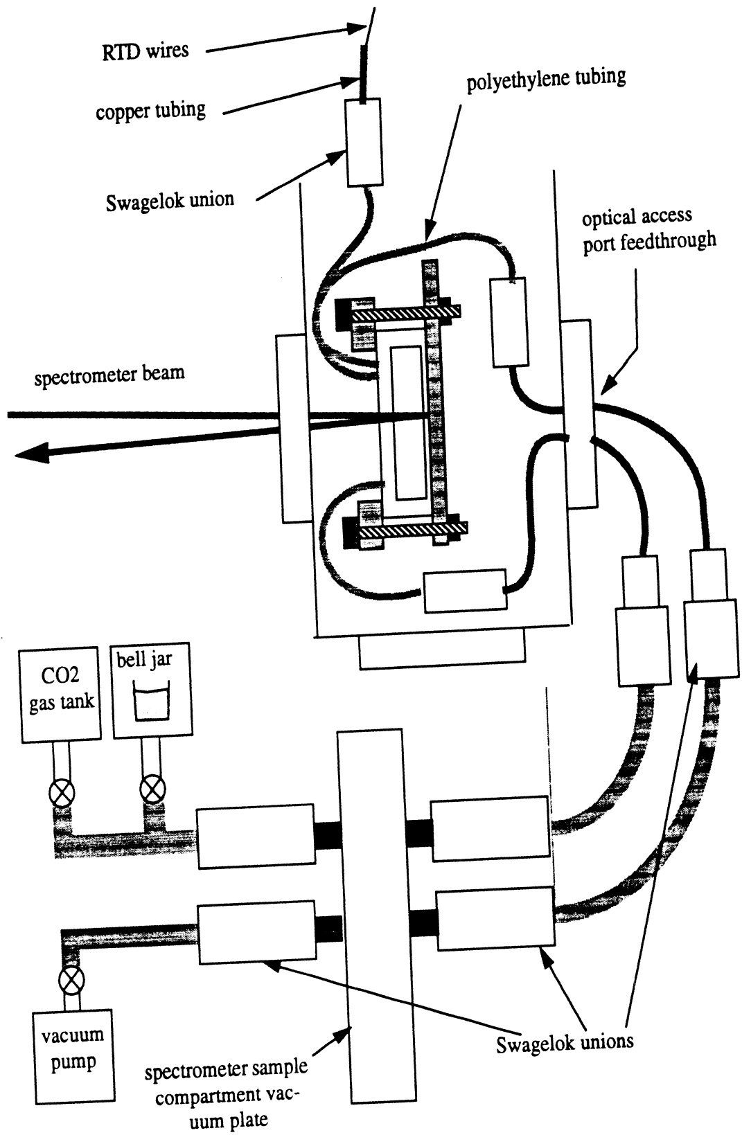
Figure (4.8): Hydrate Frost Production System
