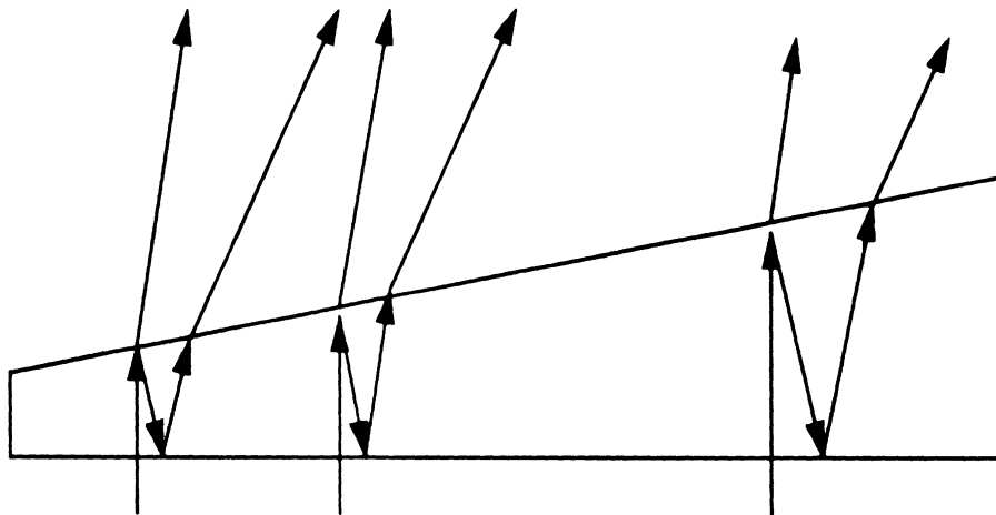
(a): Low frequency phase scrambling in a wedged substrate.
