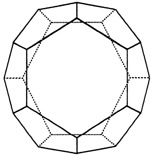
tetrakaidecahedron
