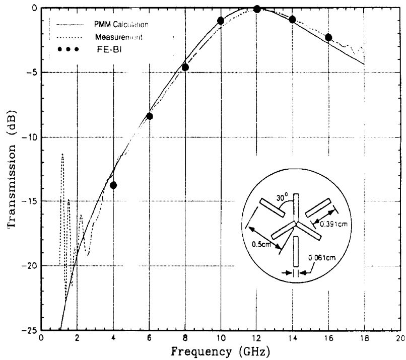
Figure 5.7: Calculations and comparisons of transmission through the FSS structure shown in fig. 5.6
