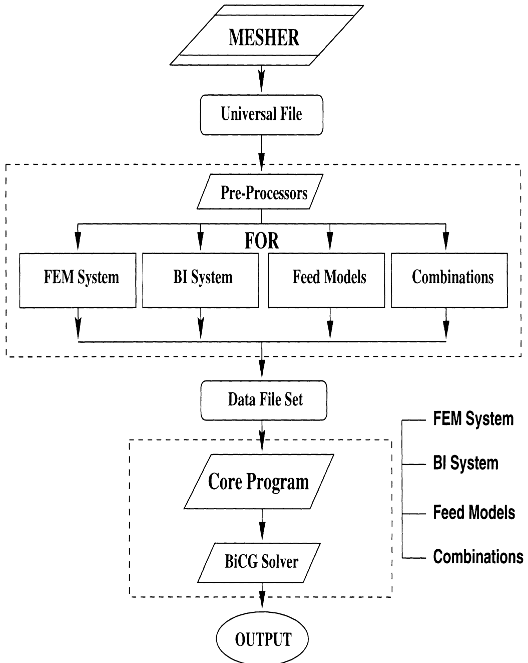
Figure 3.5: A flow chart describes the major implementation procedures from the mesh generation, a few data preprocessors, the FE–BI kernel, to the BiCG solution and finally the data output.
