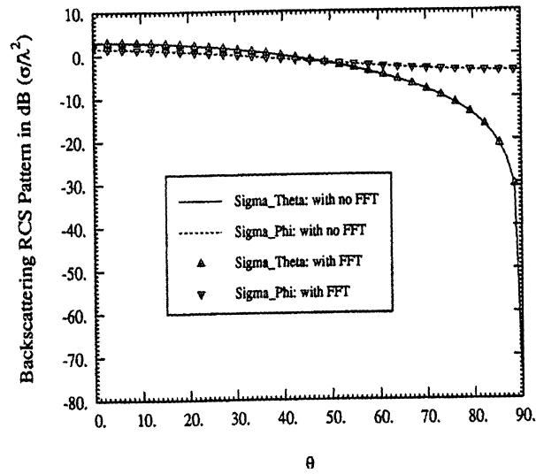
Figure 4.7: Comparisons of the monostatic radar cross section scattering by a 2 \times 2 triangular patch array shown in fig. 4.6. The results were computed using the regular BiCG FE-BI technique described in chapter 3 and using the BiCG-FFT proposed in this chapter.
