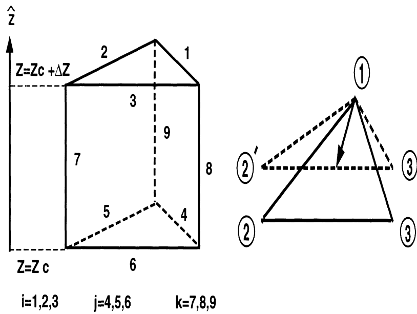
Figure 5.3: Right angled prism
