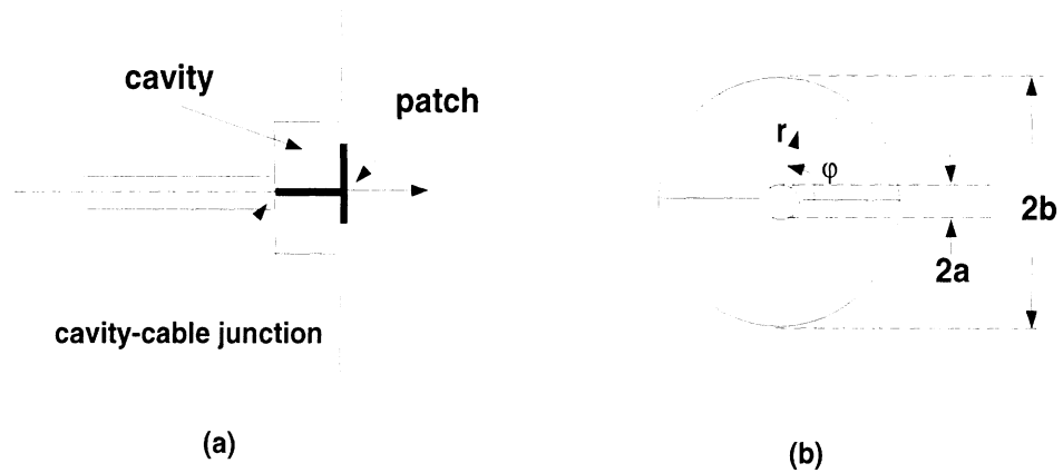
Figure 6.4: (a) Side view of a cavity-backed antenna with a coax cable feed; (b) Illustration of the FEM mesh at the cavity-cable junction (the field is set to zero at the center conductor surface).
