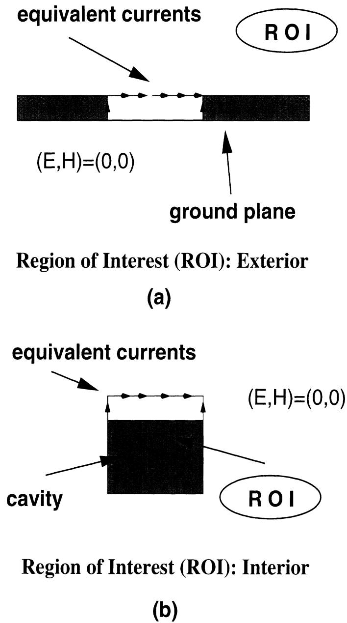
Figure 1.3: Illustrations of equivalence principle when applied to the structure shown in fig. 1.1b.
