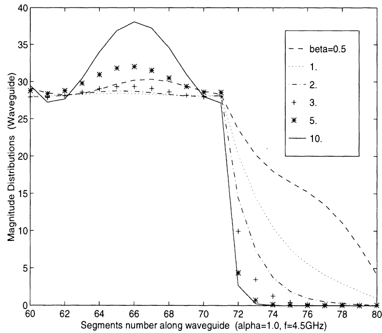
Figure 7.6: Field values of the TE_{10} mode inside a waveguide terminated by a perfectly matched uniaxial layer. The absorber is 10 elements thick and each element was 0.5 cm which translates to about 13 samples per wavelength at 4.5 GHz.
