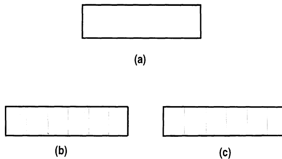
Figure 6.2: slot and its discretization (a) slot aperture; (b) typical mesh from cavity region; (c) uniform mesh from microstrip line region.
