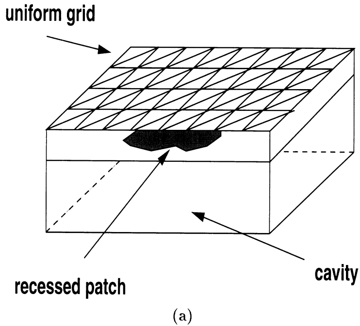
Circular Patch Recessed Underneath the Ground Plane
