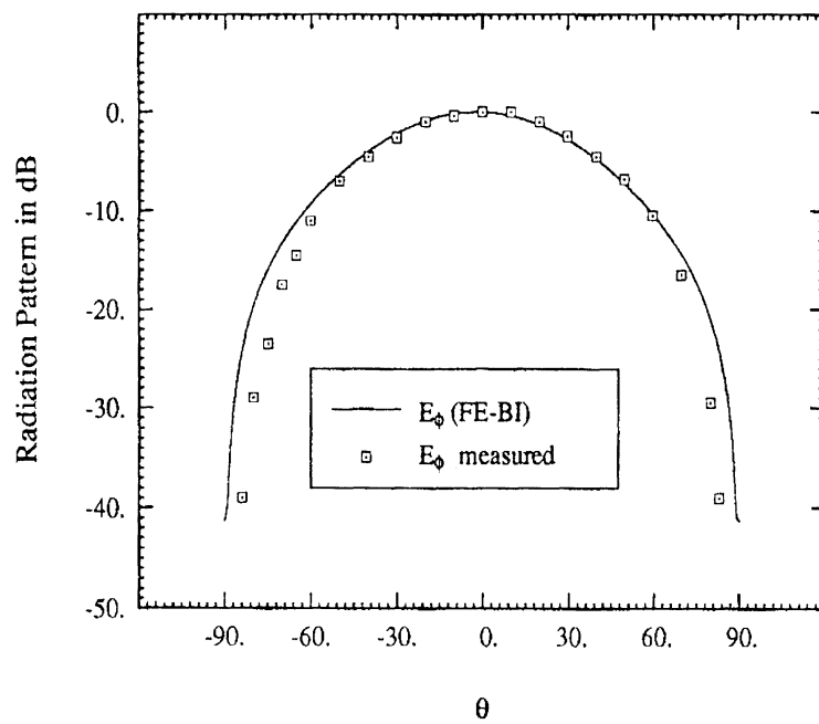
Figure 3.9: Comparison of the calculated radiation pattern ( E_\phi ), taken in the \phi = 90^\circ -plane, with data in reference [35] for the one-arm conical spiral shown in fig. 3.8
