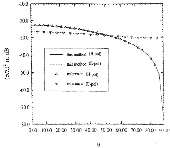
Figure 4.8: Comparisons of the monostatic radar cross section scattering by an empty aperture with the same cavity size and dielectric filling ( \epsilon_r=1 ) as the structure shown in fig. 4.6. Again, the results were calculated using the regular BiCG FE-BI technique described in chapter 3 and using the BiCG-FFT proposed in this chapter.
