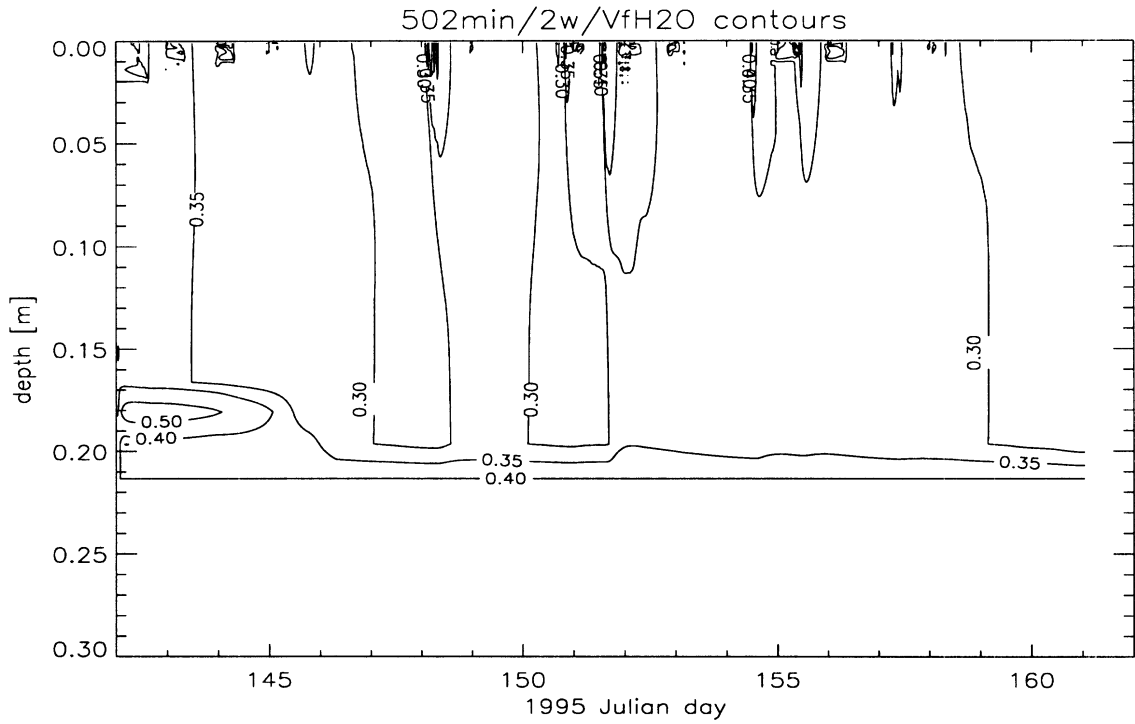
Figure 3.5: Model predicted total moisture content contours [volume fraction].
