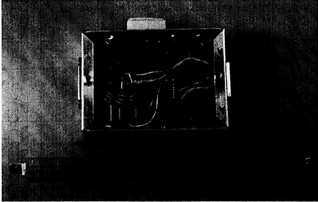
Figure 2.7: Compact radiometer signal multiplexer, A/D, and control interface module (one per microwave radiometer).
