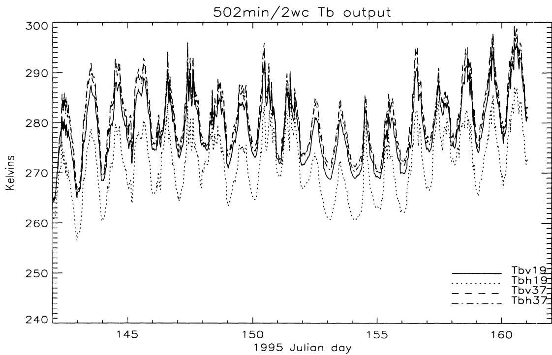
Figure 3.10: Model predicted 19 and 37 GHz brightnesses.
