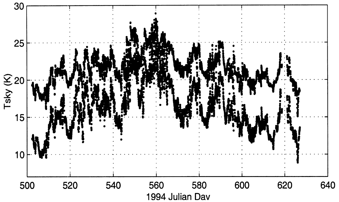
Figure 4.15: Estimated downwelling brightness, T_{SKY} , at 53^\circ seen from the surface. Lower curve: 19 GHz channels, upper curve: 37 GHz channels.
