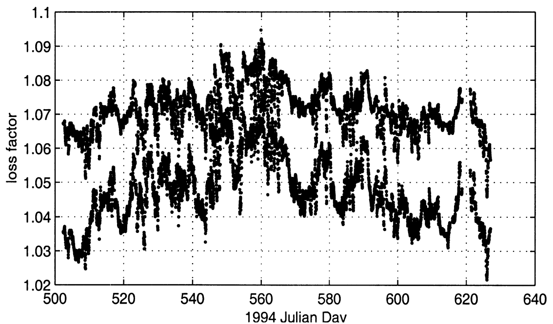
Figure 4.16: Estimated atmospheric loss factor, L(\theta, f) , at 53^\circ . Lower curve: 19 GHz channels, upper curve: 37 GHz channels.
