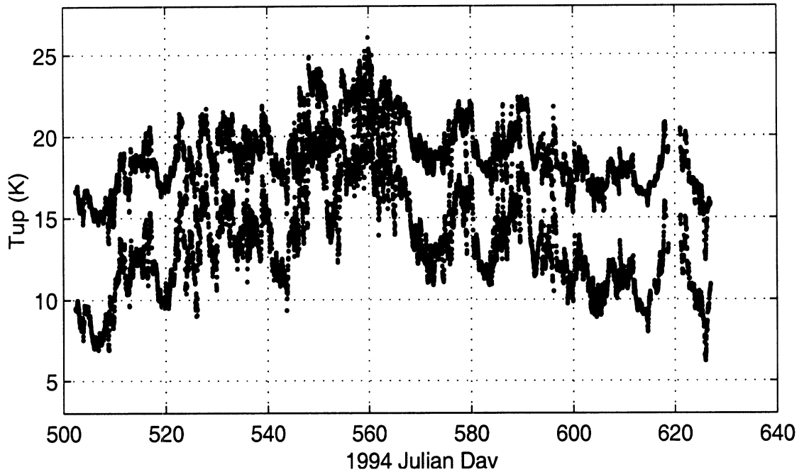
Figure 4.14: Estimated upwelling atmospheric brightness, T_{UP} , at 53^\circ seen from the TOA. Lower curve: 19 GHz channels, upper curve: 37 GHz channels.
