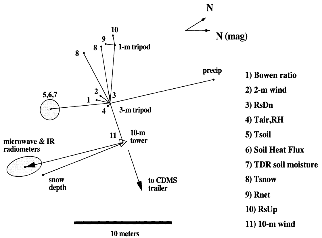
Figure 2.19: Plan view of REBEX-3 instrument locations.
