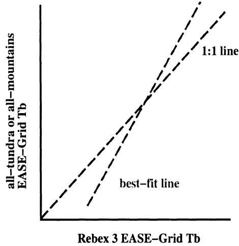
Figure 4.13: Scatter plot template for comparing all-tundra and all-mountain EASE-Grid pixels vs. REBEX-3 EASE-Grid pixel.
