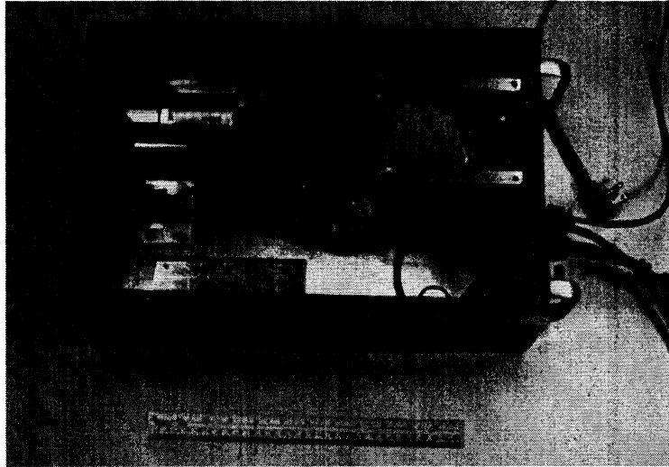
Figure 2.10: Photo of box containing the thermal IR radiometer (upper left) and fiber optic downlink circuitry (right). Video camera (removed) occupied the lower half of the box.
