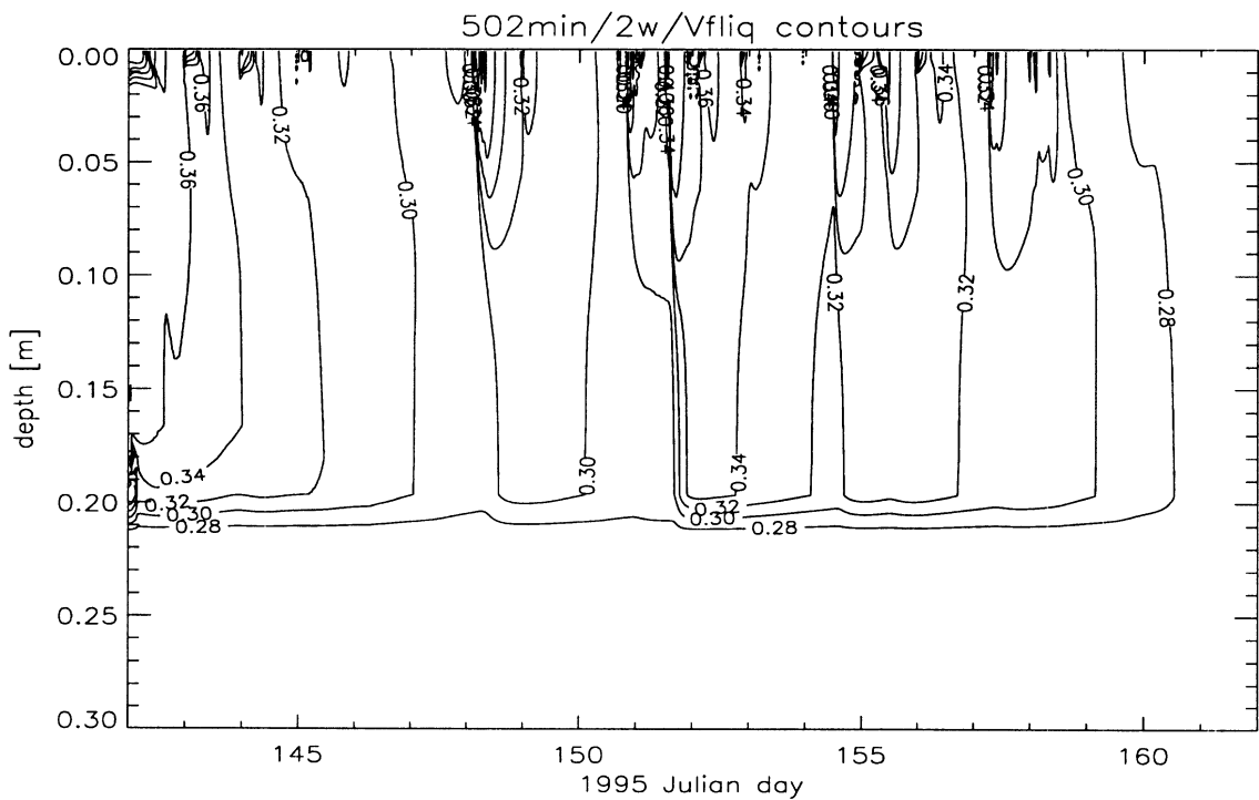
Figure 3.6: Model predicted liquid water content contours [volume fraction].
