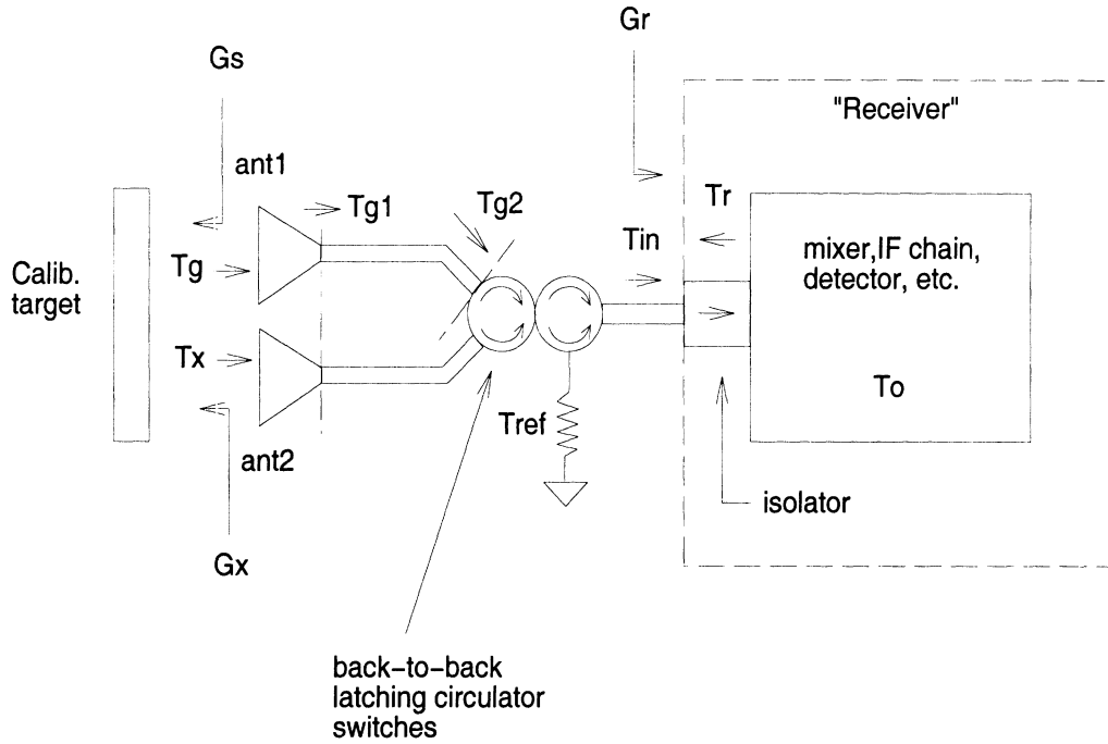
Figure 2.21: Simplified diagram of TMRS2 radiometer front end model. G_s, G_x, G_r are reflection coefficients, T_g and T_x are brightnesses entering antennas 1 and 2, respectively. T_{g1} is the brightness exiting antenna 1 and entering the waveguide. T_{g2} is the brightness available at the waveguide output. T_{ref} is the brightness temperature of the internal waveguide load. T_{in} is the brightness available to the rest of the receiver from the front end. T_r is the brightness of the rest of the receiver seen by the front end. And, T_o is the physical temperature of the receiver and circulators, assumed equal to T_{ref} .
