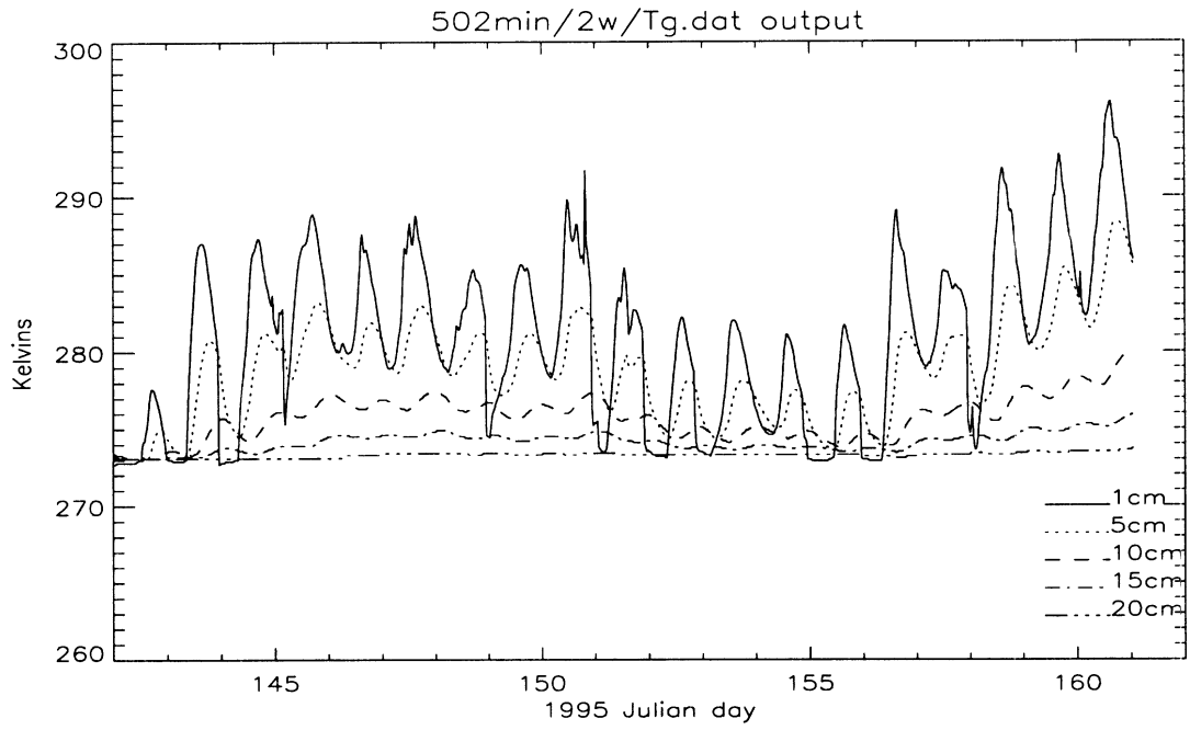
(a) Model predicted soil temperatures.
