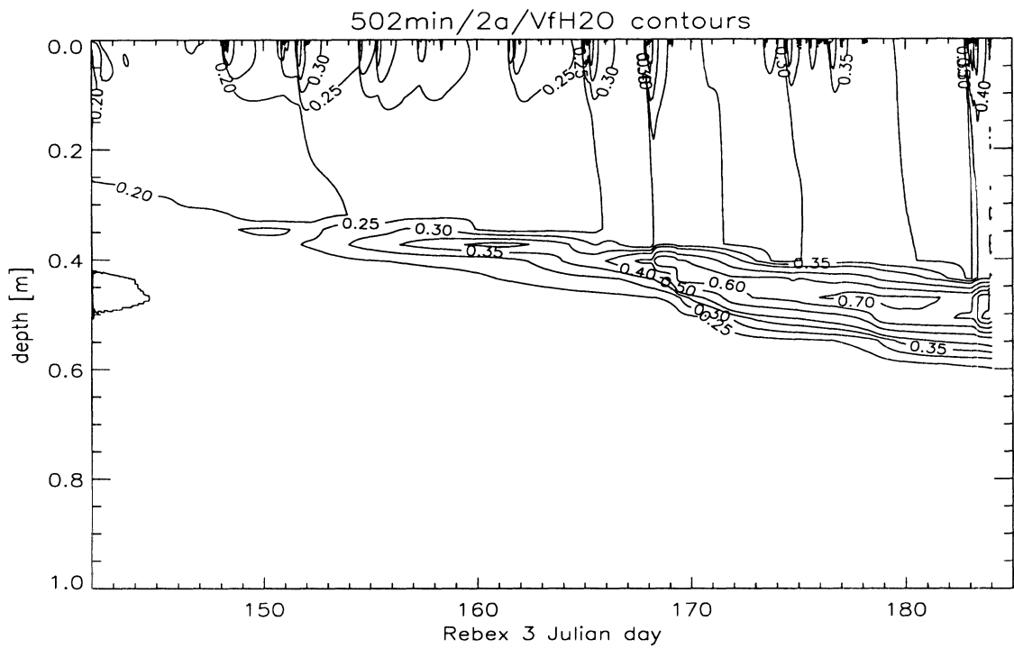
Figure 3.4: Model predicted total moisture content contours for a 60-layer run [volume fraction]. Concentration at the freezing front is qualitatively realistic, but quantitatively unphysical. Thaw depth vs. time, however, is close to measured values.
