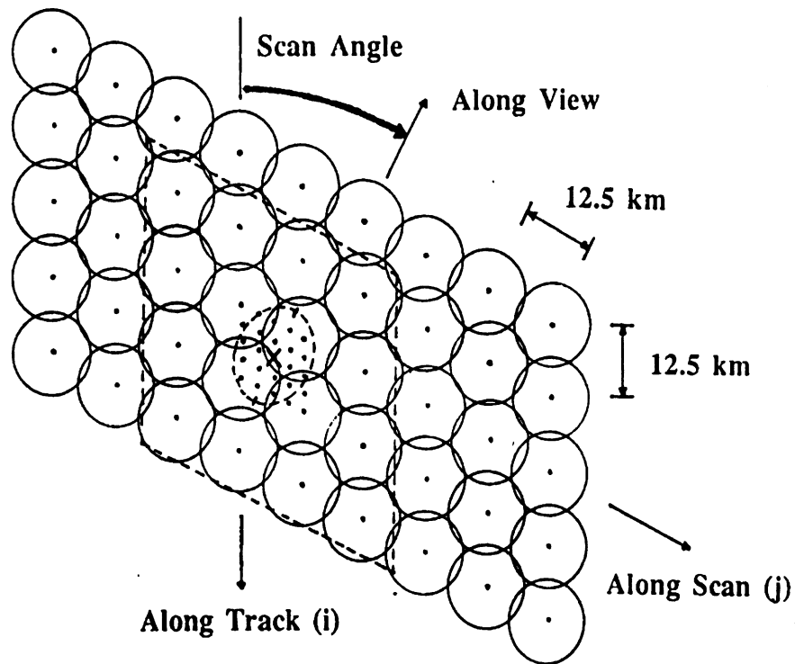
Figure 4.4: A portion of 5 consecutive scans is shown. Circles represent raw swath pixels (note: actual footprints are not circles). Weighted brightness values from the 16 pixels within the dashed box are combined to generate interpolated observations on the densified grid. The dashed oval represents the footprint of the desired resampled observation, with the 'X' marking the center. The data from the nearest-neighbor pixel on the densified grid is re-registered to the EASE-Grid cell located at 'X'. From [28] with permission.
