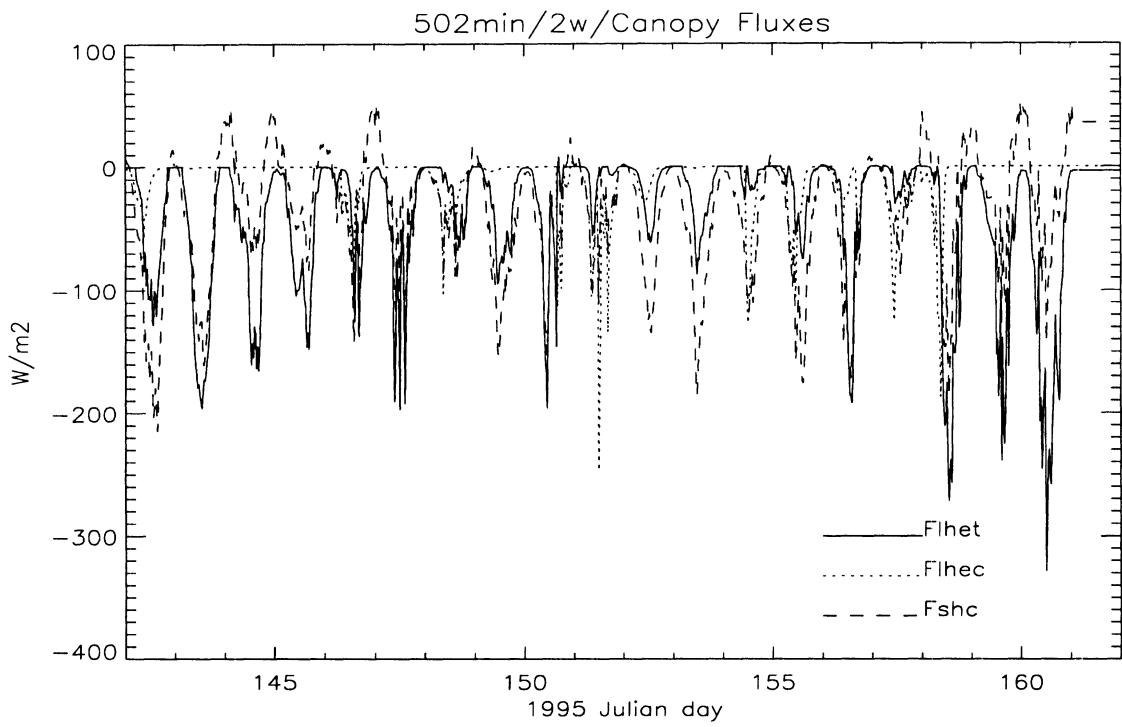
Figure 3.9: Model predicted canopy fluxes.
