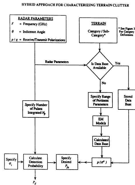
Figure 2. Flow-chart representation of the radar-detection performance simulation package.
