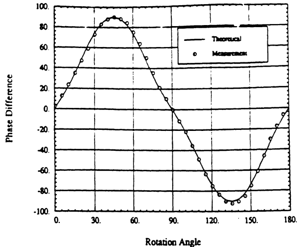
Fig. 4. The measured and calculated phase difference of the signals at the OMT output ( A and B ).
