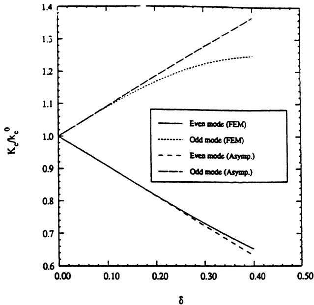
Fig. 2. First two cutoff wave number for an elliptical waveguide with axial ratio \frac{1+\delta}{1-\delta} normalized to the dominant cutoff wave number of the circular waveguide ( \delta = 0 ).
