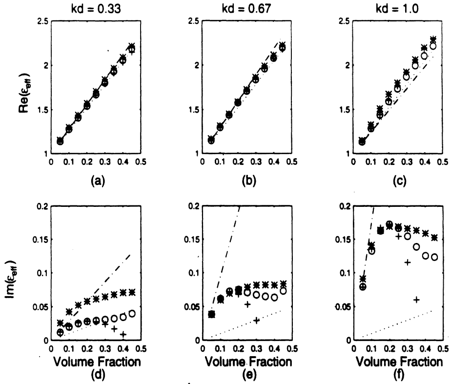
Figure 10: Comparison between five methods of determining effective permittivity for a TM polarized field: EFA (-), PVS (...), QCA-PY (o), QCA-HC (+) and NUM-PY (*). Plots (a) through (c) illustrate \text{Re}(\epsilon_{\text{eff}}) and (d) through (f) illustrate \text{Im}(\epsilon_{\text{eff}}) as a function of volume fraction using a model of particles ( \epsilon_i = 3.6 + i0.1 ) suspended in a classical fluid. Particle diameter ranges from \lambda_i/10 ( kd = 0.33 ) (a and d), 2\lambda_i/10 ( kd = 0.67 ) (b and e), to 3\lambda_i/10 ( kd = 1.0 ) (c and f).
