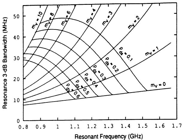
Fig. 11. Nomogram giving snow liquid water content ( m_v ) and equivalent dry snow density ( \rho_{ds} ) in terms of two parameters directly measured by the snow probe: resonant frequency ( f ) and resonance (3-dB) bandwidth ( \Delta f ).
