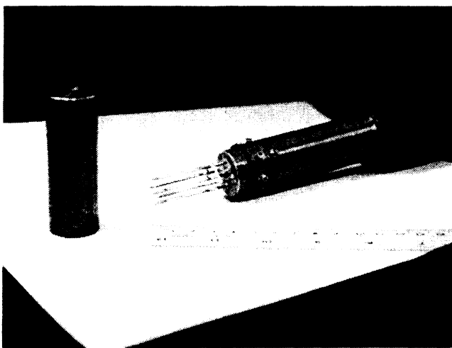
Fig. 4. Photograph of snow probe with cap.
