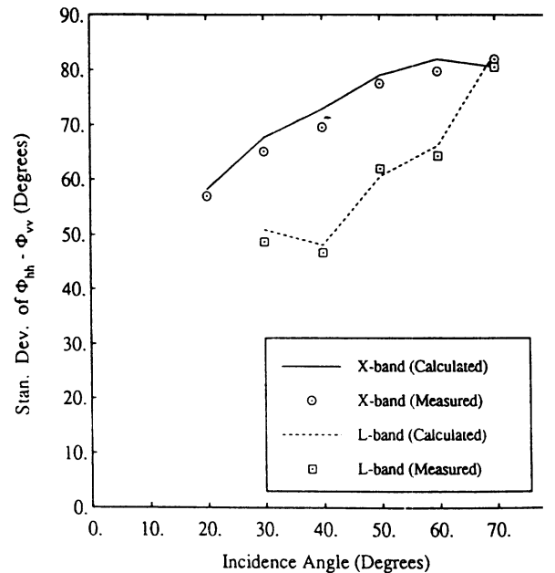
Fig. 9. Angular dependency of the standard deviation of the copolarized phase difference for a dry rough surface with a rms height of 0.4 cm and a correlation length of 8 cm at L- and X-band.
