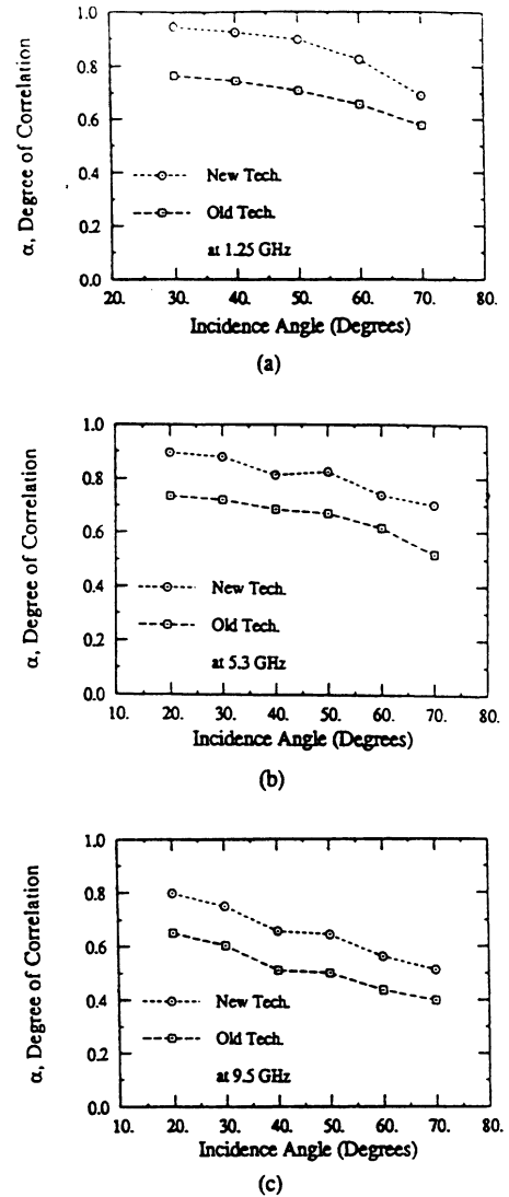
Fig. 7. Degree of correlation for copolarized components of the scattering matrix for the L -band (a), C -band (b), and X -band (c).
