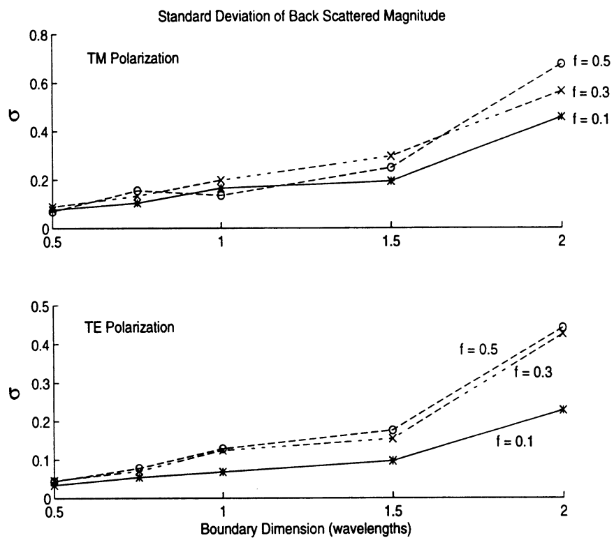
Figure 8: Standard deviation of backscattered field magnitude for three different volume fractions (0.1, 0.3 and 0.5), and both TM and TE polarizations. Similar behavior was observed for the forward scattered field as well.
