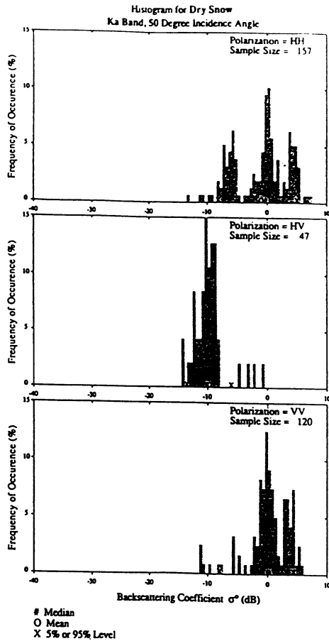
Figure 4. Histograms of \sigma^0 for dry snow at 35 GHz.
