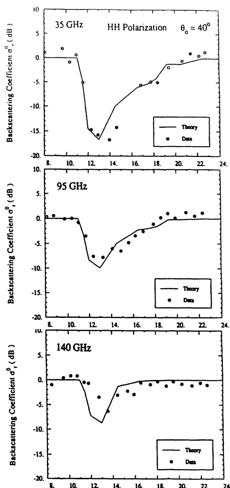
Figure 7. Comparison of measured and calculated diurnal response of \sigma^o for snow at 35, 95, and 140 GHz. The incidence angle is 40^\circ , snow density is 0.32 \text{ g/cm}^3 , and the snow depth is 12 cm.
