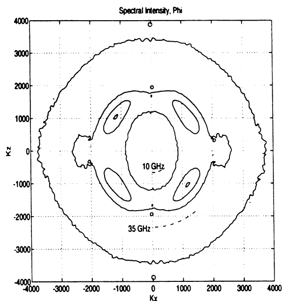
Figure 12: Illustration of the visible region of the Born approximation at two different frequencies shown overlaid on a contour map of the power spectral density (Fig. 9) for the Gaussian particle size distribution. Note that the greatest angular variation due to the packing structure occurs near resonance at f = 21 GHz.
