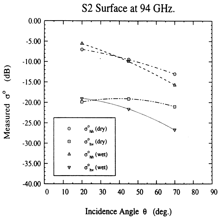
Figure 11: Measured \sigma_{hh}^o and \sigma_{hv}^o for wet and dry surface conditions at 94 GHz ( ks = 5.16 ). Note that at 70^\circ , \sigma^o (dry) is greater than \sigma^o (wet) for both polarizations, evidence of volume scattering contribution.
