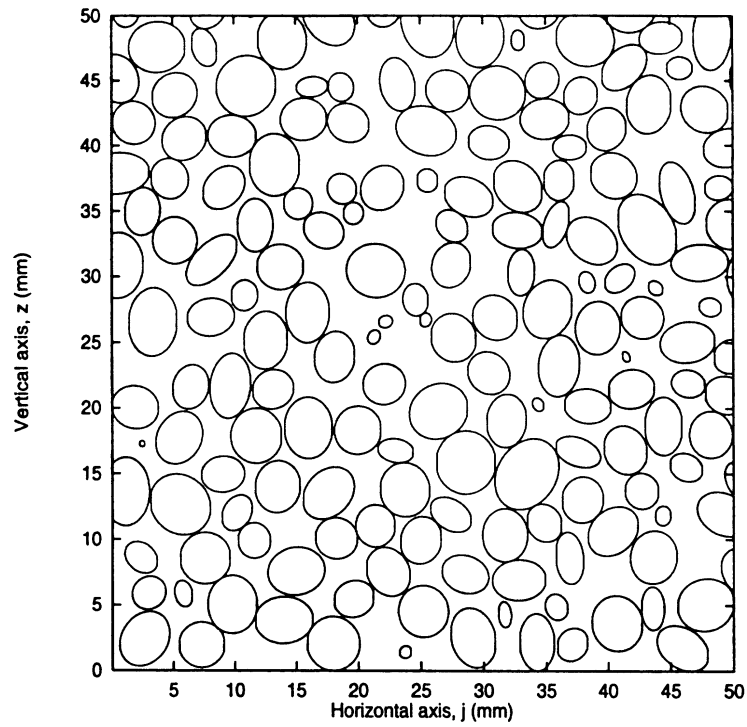
Figure 5: Demonstration of the three-dimensional packing algorithm. Shown is one slice taken out of a 50\text{mm}^3 cube filled with ellipsoidal particles with radii of 2\text{mm} \pm 0.4\text{mm} . This simulation using 3300 particles took approximately 3 hours using 24 processors of an IBM SP Parallel computer.
