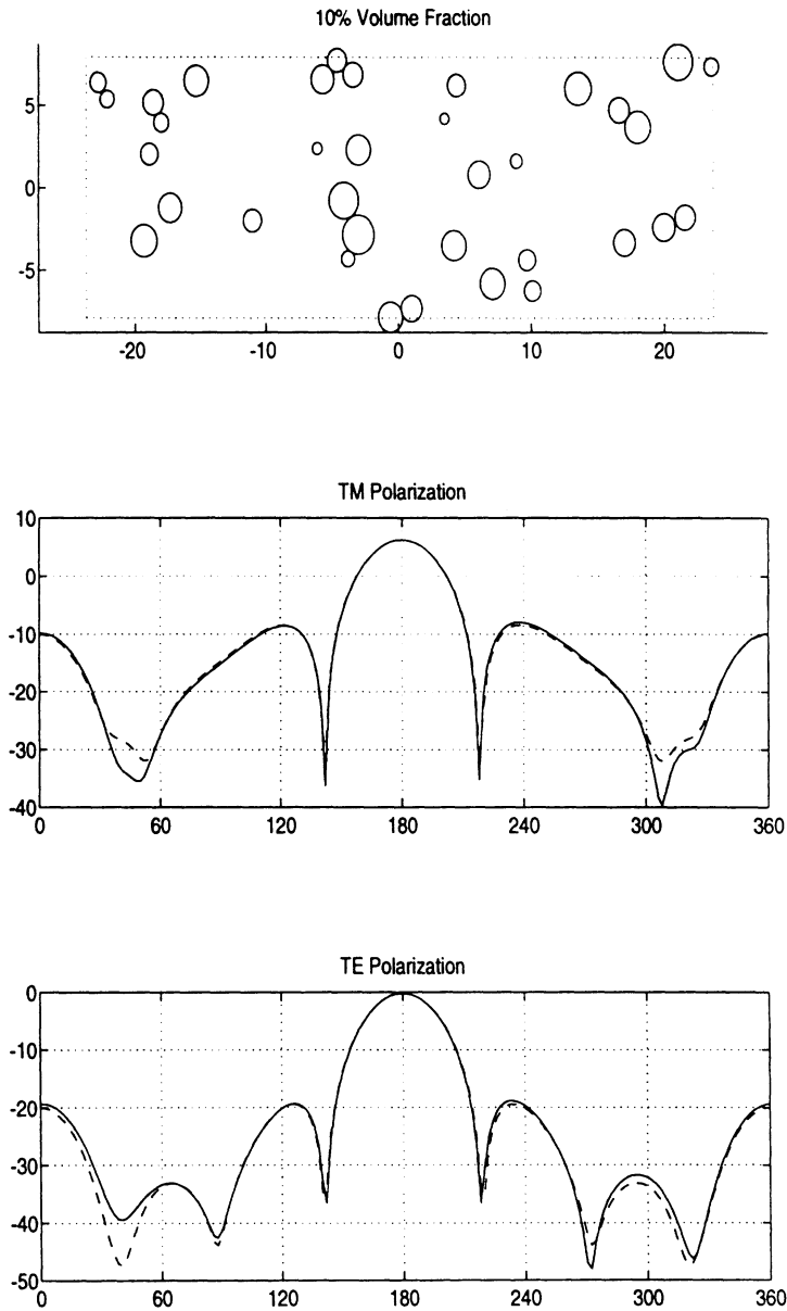
Figure 2: Algorithm results for 10% volume fraction. Shown here is a.) a sample collection of particles confined within an imaginary boundary, b.) average scattered TM field (solid line) and the scattered field from a homogeneous dielectric with permittivity, \epsilon_{\text{eff}} (dashed line), c.) average scattered TE field (solid line) and the scattered field from a homogeneous dielectric with permittivity, \epsilon_{\text{eff}} (dashed line).
