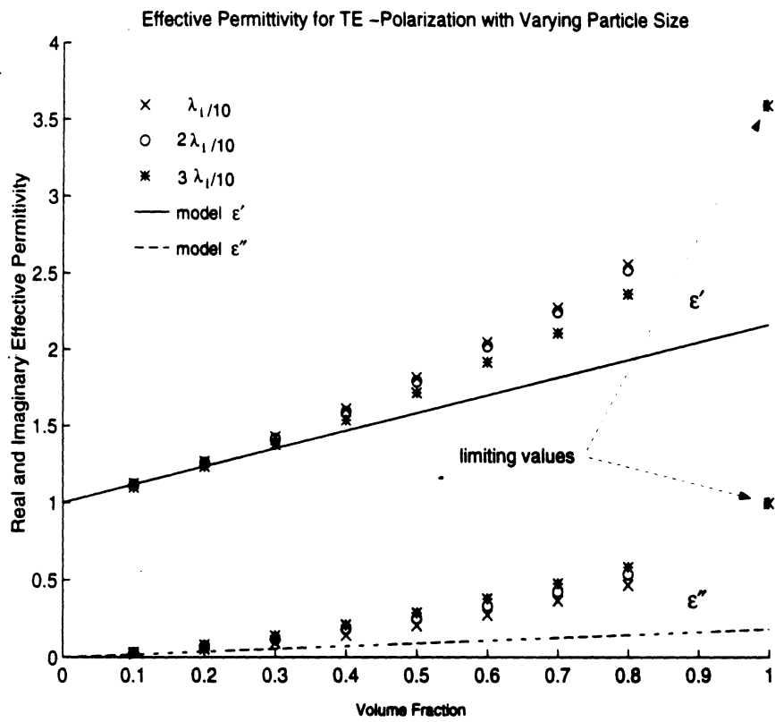
Figure 9: Effective permittivity, \epsilon_{\text{eff}} vs. volume fraction for a TE polarized field. See Fig. 7 for details.
