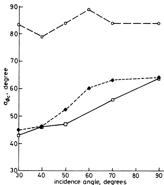
Fig. 12 Measured standard deviation of co-polarised phase difference at 35 GHz for three types of trees
