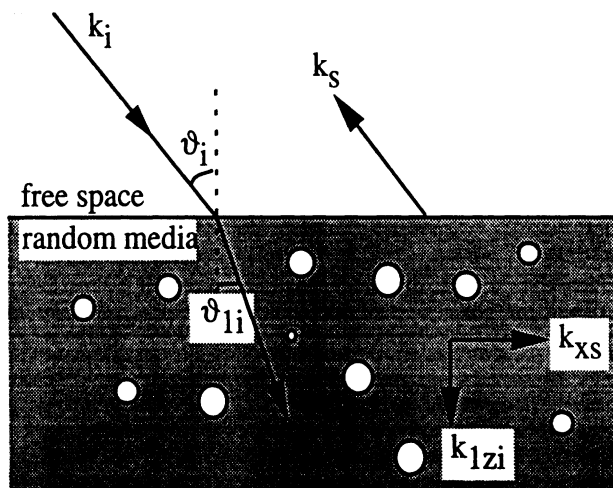
Figure 7: Geometry for a two-dimensional random medium. Medium 0 is considered free space and medium 1 is a random media consisting of particles as described in Fig. 4.
