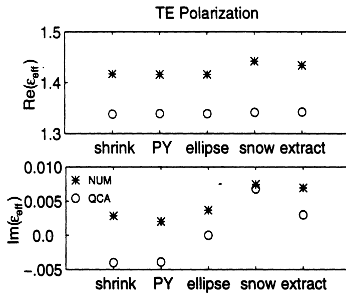
Figure 17: Effective permittivity comparison between particle arrangement methods. Volume fraction = 30%, \epsilon_i = 3.6 + i0.01 , TE Polarization.
