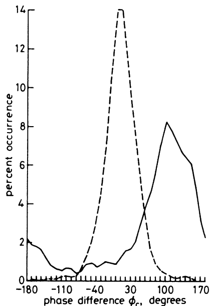
Fig. 8 Measured co-polarised phase angle distributions for two corn fields observed by a 1.2 GHz polarimetric SAR at incidence angles of 19^\circ and 50^\circ
