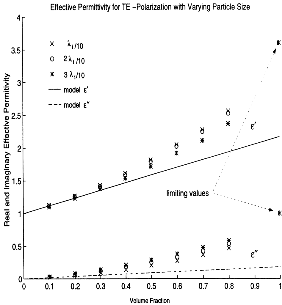
Figure 5: Simulation and mixing formula results for TE polarization.
