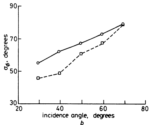
Fig. 7 Standard deviation of the co-polarised phase angle as a function of incidence angle
