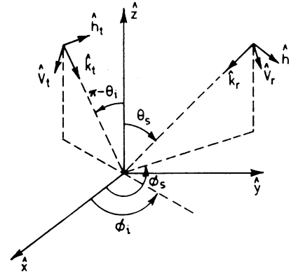
Fig. 1 Co-ordinate systems and scattering geometry for the backscatter alignment (BSA) convention
