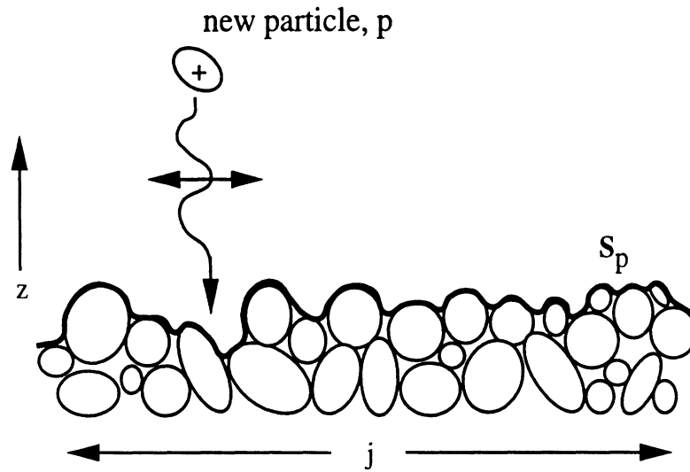
Figure 1: Illustration of the two-dimensional packing algorithm. Particles are fit to the surface S_p to find the minimum height, z . Once a particle has been fit to the surface, it becomes part of the surface for the next iteration of the process.
