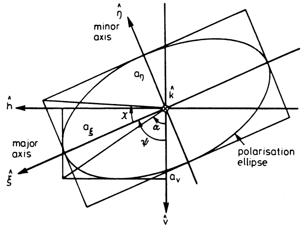
Fig. 2 Polarisation ellipse in the v - h plane for a wave travelling in the k direction
