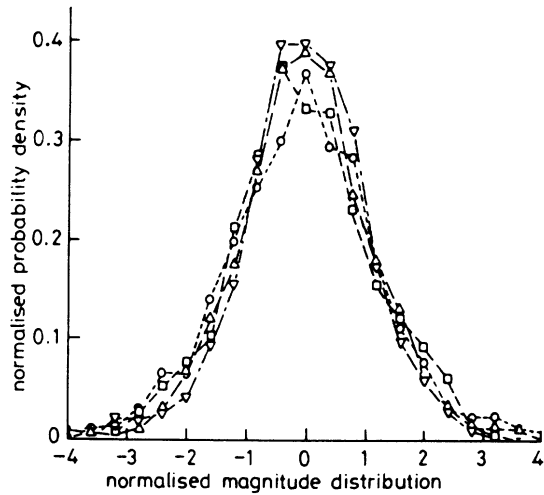
Fig. 3 Histogram of the real and imaginary parts of S_{vv} and S_{hh} for a rough surface with rms height 0.32 cm and correlation length 9.9 cm at C-band and 30° incidence angle
