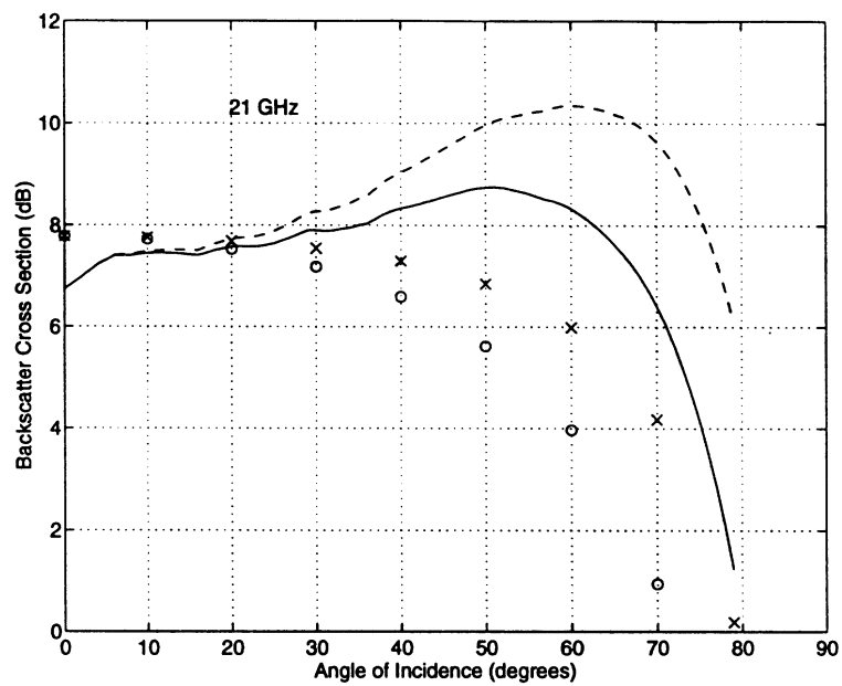
Figure 14: Results of the two-dimensional Born approximation at particle resonance ( f = 21\text{GHz} ) for both numerically derived (Gaussian particle size distribution) and exponential correlation functions. Solid lines (-) and circles (o) indicate vertical and dashed lines (- -) and crosses (x) indicate horizontal polarizations. The symbols represent the theoretical exponential curves in both cases.
