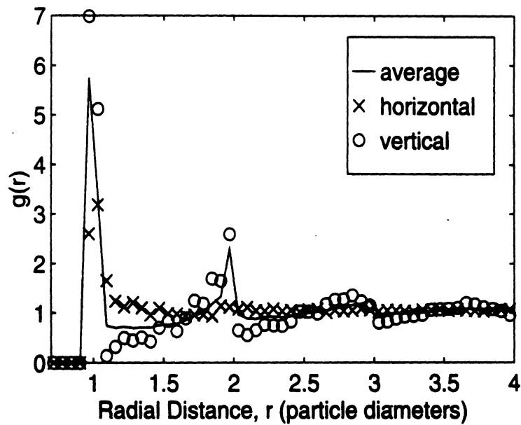
Figure 4: Simulation of a two-dimensional snow-type medium for a volume fraction of 30%. Shown is the average pair distribution function over all angles and the pair distribution function from the vertical and horizontal directions which accentuate the azimuthal asymmetry.
