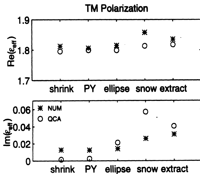
Figure 16: Effective permittivity comparison between particle arrangement methods. Volume fraction = 30%, \epsilon_i = 3.6 + i0.01 , TM Polarization.
