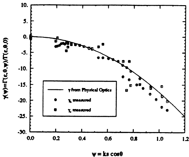
Fig. 7. The reduction of coherent scattering from a surface due to roughness. Shown is the measured coherent reflectivity of several surfaces (all with with \epsilon' = 3 ) but differing roughness parameters \psi , normalized to the reflection coefficient of a smooth surface. The angles of incidence range from 20^\circ to 70^\circ and the roughness ks ranges from 0 to 2. The continuous curve is the Physical Optics prediction for surfaces with Gaussian-height probability densities.
