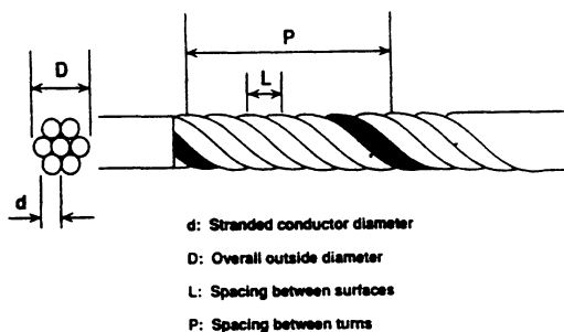
Fig. 3. Geometry of powerline cable.
