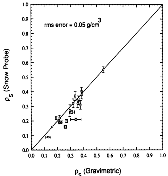
Fig. 10. Comparison of snow density results obtained via snow probe (with associated empirical algorithm) and gravimetric measurements.
