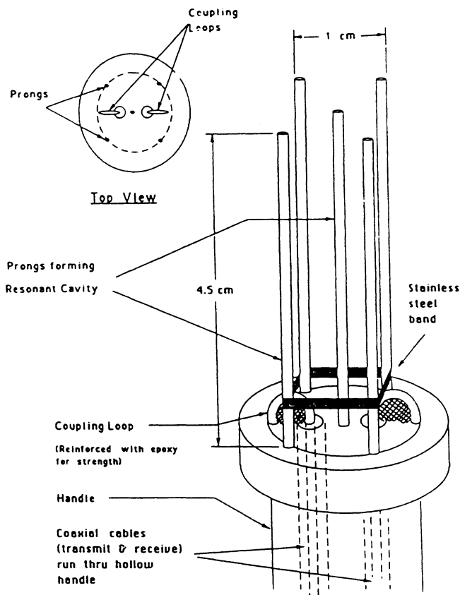
Fig. 3. Illustration of snow probe. Coaxial transmission lines extend through handle. At the face of the snow probe, the center conductors of the coaxial lines extend beyond and curl over to form coupling loops.
