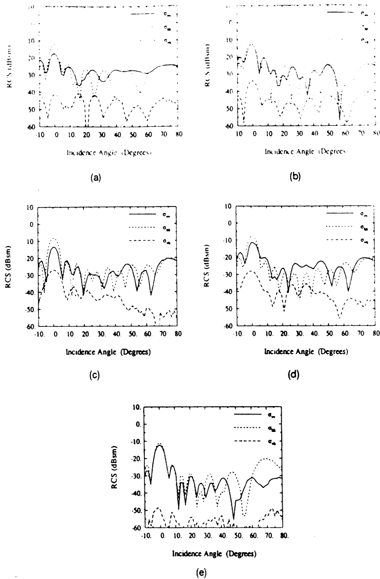
Fig. 5. Radar backscatter cross section for 30 cm long cable. (a) Cable 1. (b) Cable 2. (c) Cable 3. (d) Cable 4. (e) Smooth cylinder of diameter 1.27 cm, at 4.75 GHz.
