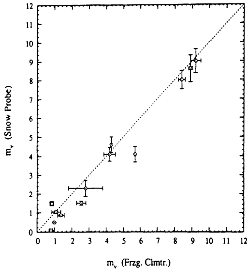
Fig. 6. Comparison of snow wetness results obtained via snow probe and freezing calorimetry, respectively. Snow probe data points are based on an average of twelve separate measurements.
