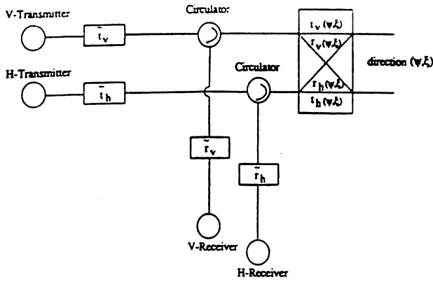
Fig. 2. Simplified block diagram of a polarimetric radar system.
