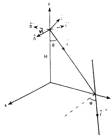
Fig. 4. Geometry of radar system above powerline cable.
