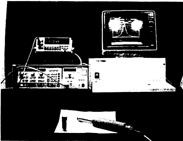
Fig. 1. Photograph of snow probe system.
