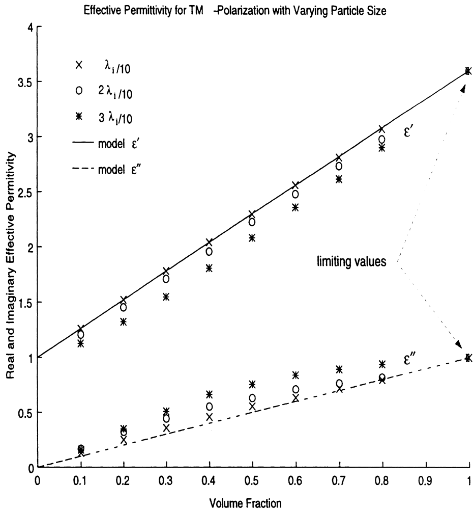
Figure 4: Simulation and mixing formula results for TM polarization. Real (solid line) and imaginary (dashed line) components of the effective permittivity derived from the Polder-Van Santen mixing formula compared with effective permittivity obtained by numerical simulation. Symbols indicate different particle diameters of \lambda_i/10 - x, 2\lambda_i/10 - o, and 3\lambda_i/10 - *. Inclusion permittivity is \epsilon_i = 3.6 + i1.0
