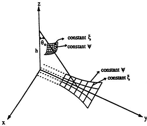
Fig. 4. Geometry of a radar above x - y plane and transformation of azimuth-over-elevation coordinate to Cartesian coordinate.
