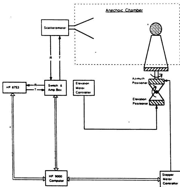
Fig. 1. Automatic radar cross section measurement setup.
