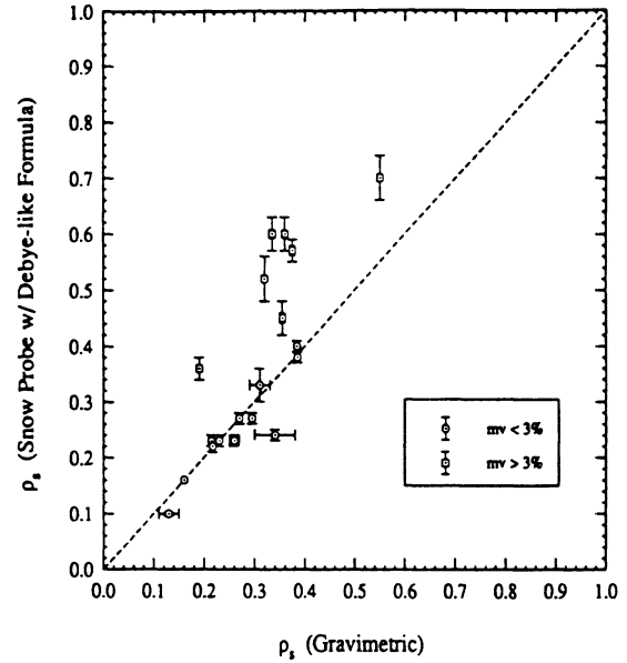
Fig. 7. Comparison of snow density results obtained via snow probe (in conjunction with Debye-like relation) and gravimetric measurements. Data points represented with squares were from snowpacks having volumetric wetness levels of >3\% ; with circles, <3\% .
