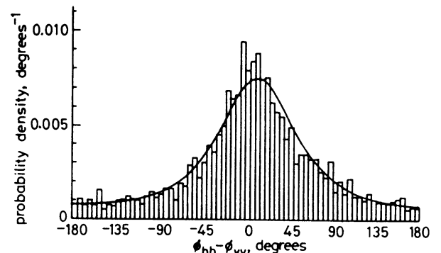
Fig. 5 Measured and calculated f(\phi_c) for a grassy area in Northern Michigan observed by a 1.2 GHz SAR in April 1990
