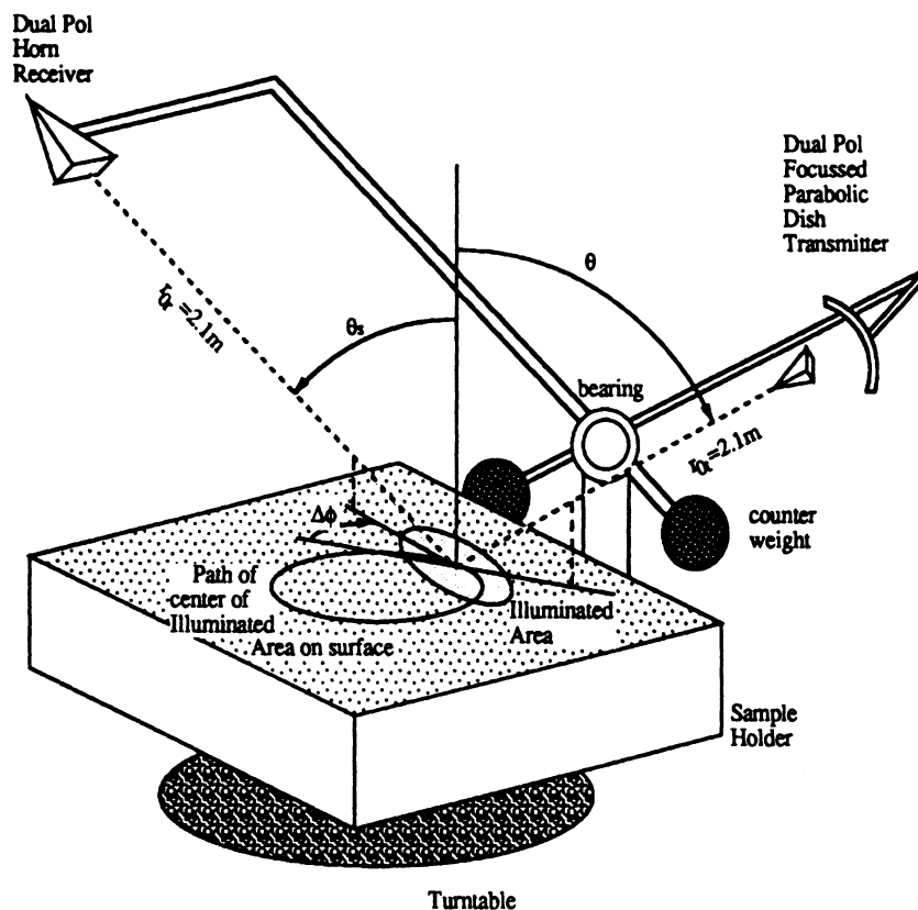
Fig. 4. Diagram of the Bistatic Facility.
