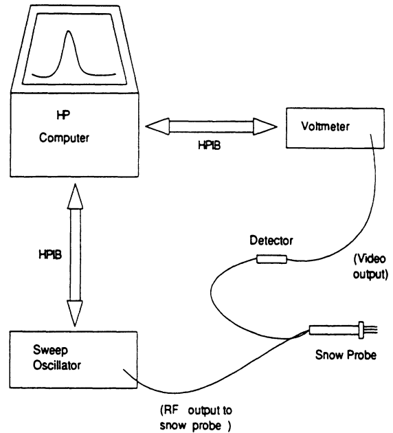
Fig. 2. Schematic diagram of snow probe system.
