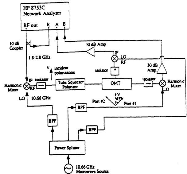
Fig. 3. Experimental setup for tuning and characterizing the prototype K -band squeezed waveguide polarizer.
