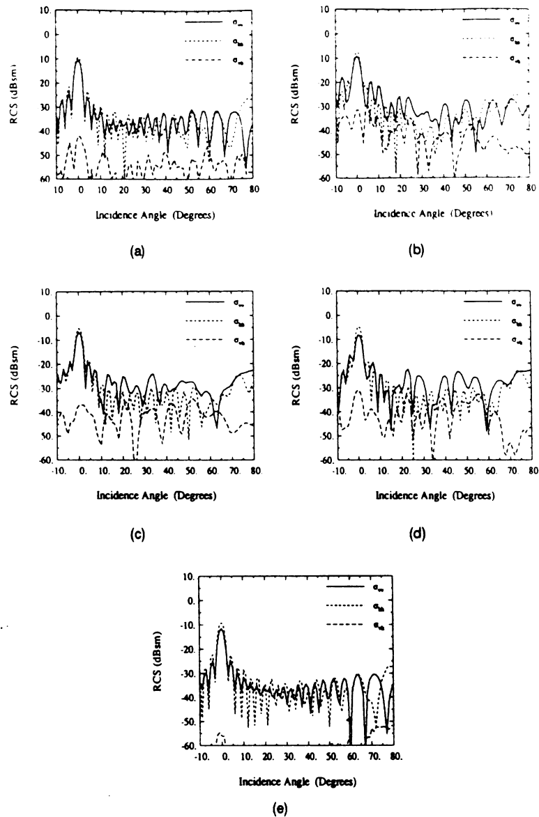
Fig. 7. Radar backscatter cross section for 30 cm long cable. (a) Cable 1. (b) Cable 2. (c) Cable 3. (d) Cable 4. (e) Smooth cylinder of diameter 1.27 cm, at 9.5 GHz.
