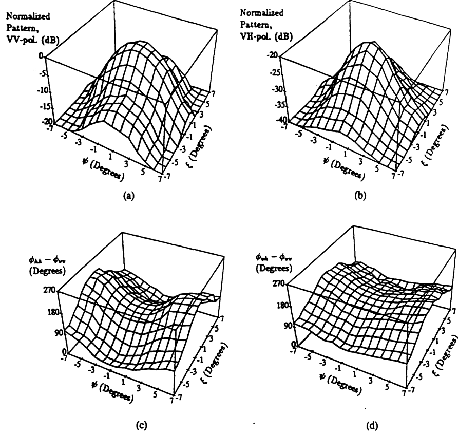
Fig. 5. Polarimetric response of a metallic sphere over the entire mainlobe of X -band scatterometer; normalized \sigma_{vv} (a) corresponds to G_v^2 and normalized \sigma_{vh} (b) corresponds to G_v G_h ; phase difference between copolarized (c) and cross-polarized (d) components of the sphere response correspond to phase variation of the co- and cross-polarized patterns of the antenna.
