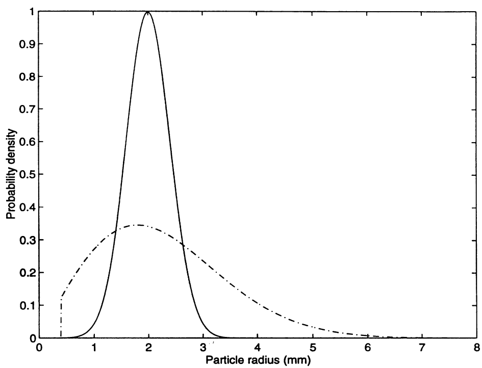
Figure 10: Gaussian (solid line, -) and truncated Rayleigh (dot dashed line, .-) Probability distribution functions of particle radii used in the packing algorithm. Both distributions have the same mean.
