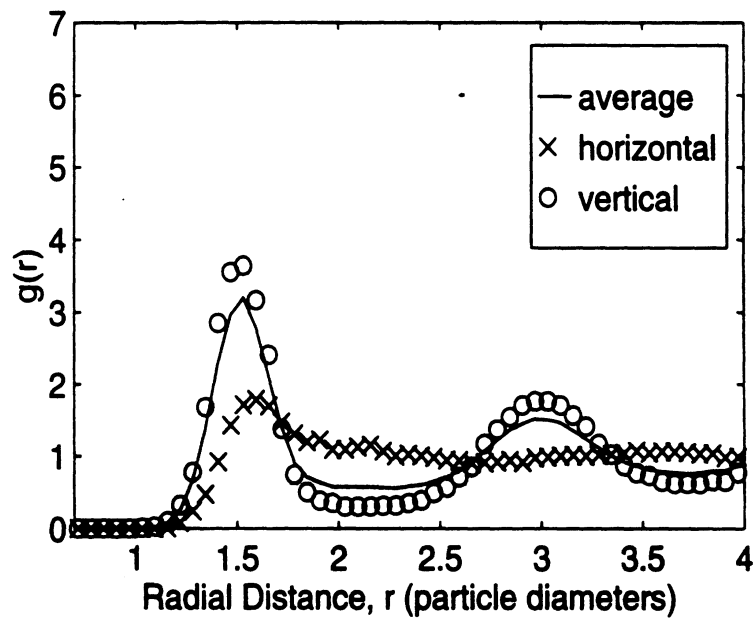
Figure 5: Particle arrangement simulation using a distribution of disks shrunk down to a uniform size for a volume fraction of 30%. Shown is the average pair distribution function over all angles and the pair distribution function from the vertical and horizontal directions which accentuate the azimuthal asymmetry. This example is given to demonstrate one method of obtaining different particle arrangements and different pair distribution functions.
