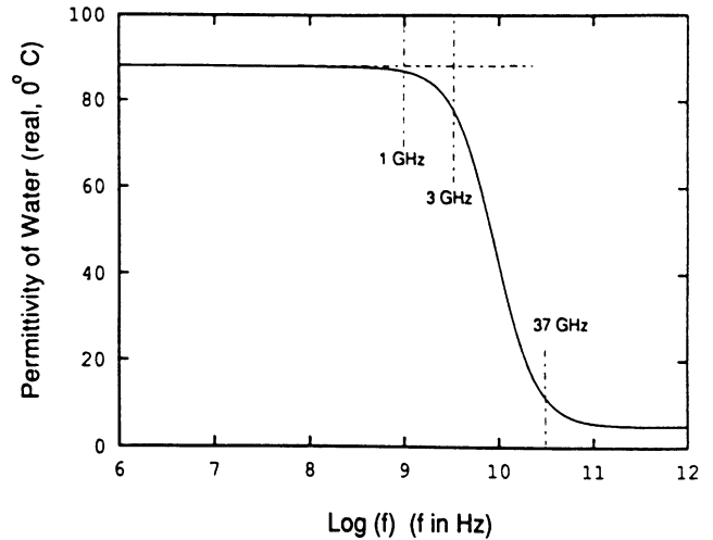
Fig. 9. Real part of permittivity of water at 0°C.
