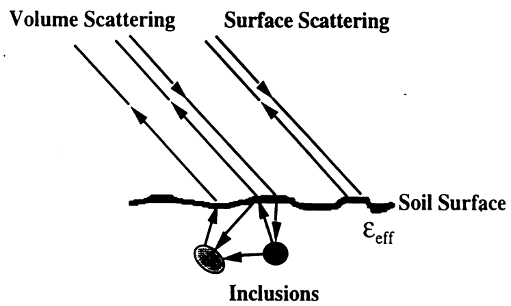
Figure 5: Surface and volume-scattering mechanisms contributing to the total backscatter.
