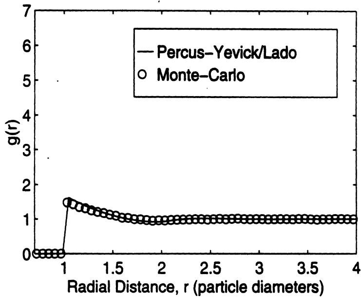
Figure 2: Simulation of a classical fluid for a volume fraction of 30%. Shown are results from Monte-Carlo numerical simulations and the PY equation in two dimensions solved by Lado.
