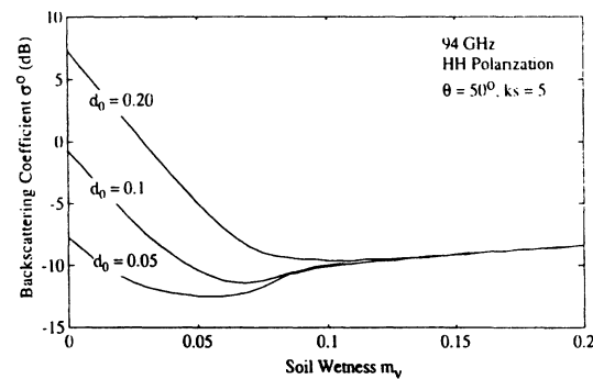
Figure 12. Variation of \sigma^0 at 94 GHz with m_v for moderately rough surface with ks = 5 .
