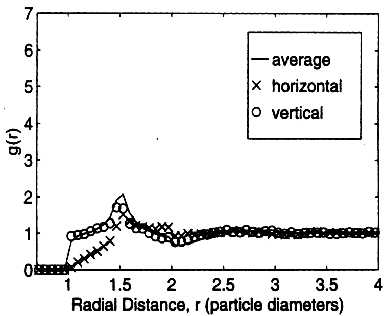
Figure 6: Particle arrangement simulation using ellipses for a volume fraction of 30%. Shown is the average pair distribution function over all angles and the pair distribution function from the vertical and horizontal directions which accentuate the azimuthal asymmetry. This example is given to demonstrate one method of obtaining different particle arrangements and different pair distribution functions.
