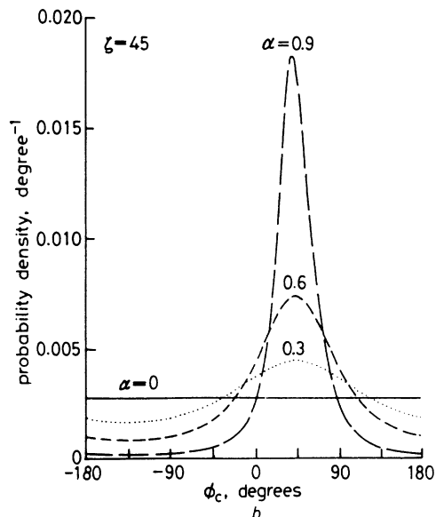
Fig. 6 Plots of f(\phi_c)
