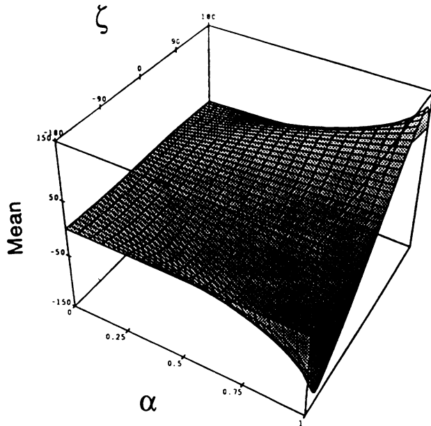
Fig. 3. The mean value of the copolarized phase difference as a function of \alpha (degree of correlation) and \zeta (coherent phase difference).
