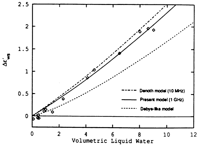
Fig. 8. \Delta\epsilon'_{ws} versus m_v . Shown is data and best fit curve, plus a model obtained from a comparable study at 10 MHz, and Debye-like model.
