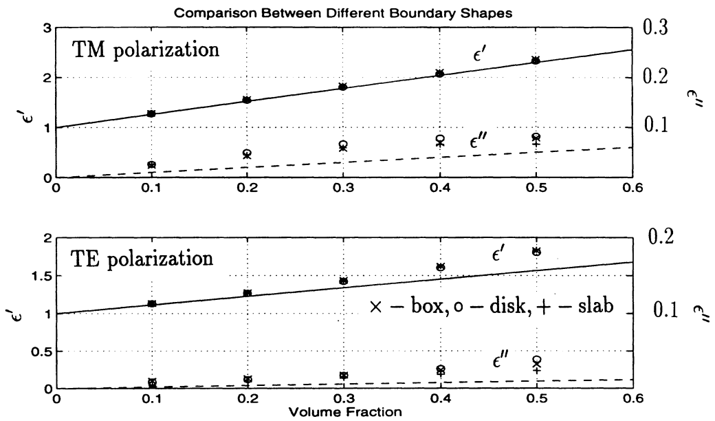
Figure 9: Effective permittivity comparison for differing boundary shapes. Shown are the real and imaginary permittivities for three different boundary shapes: o - circular disk (diameter = 2\lambda_i ), + - rectangular slab ( 3\lambda_i \times \lambda_i ) and \times - square box ( 1.5\lambda_i \times 1.5\lambda_i ). The imaginary part of the effective permittivity is multiplied by ten so that both parts of the effective permittivity may be displayed on the same graph. Lines indicate results from the two-dimensional Polder-Van Santen mixing formula.
