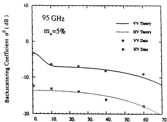
Figure 6. Measured and calculated angular variation of \sigma^o for wet snow with 5% wetness at 95 GHz.
