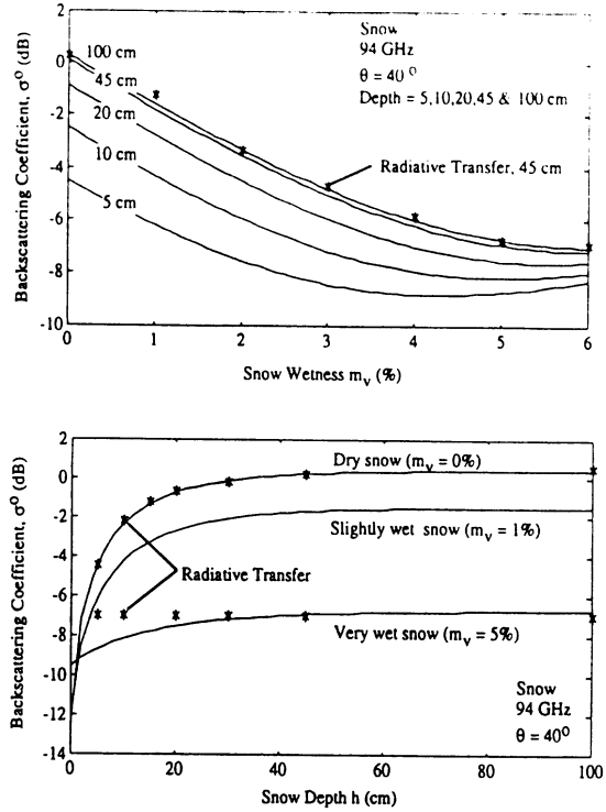
Figure 9. Variations of co-polarized \sigma^o with snow depth h and snow liquid water content m_v at 94 GHz.
