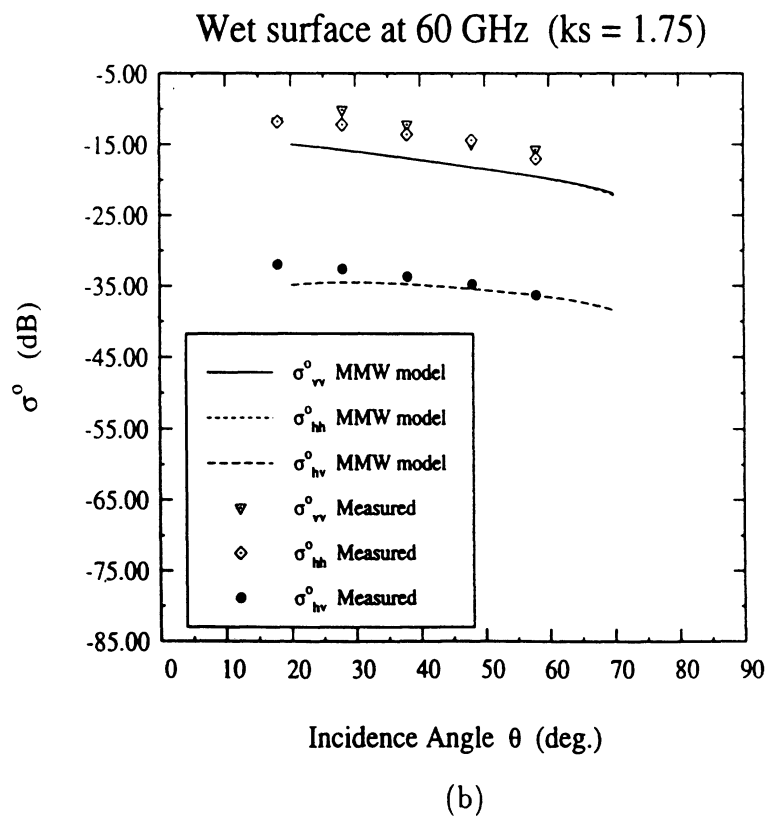
Figure 10: Comparison between measured data for wet soil surfaces ( \epsilon_r = 1.9 + j 0.4 ) at 60 GHz and the MMW semi-empirical surface scattering model for (a) ks = 0.16 , and (b) ks = 1.75 . (Data from Yamasaki et al. [3]).
