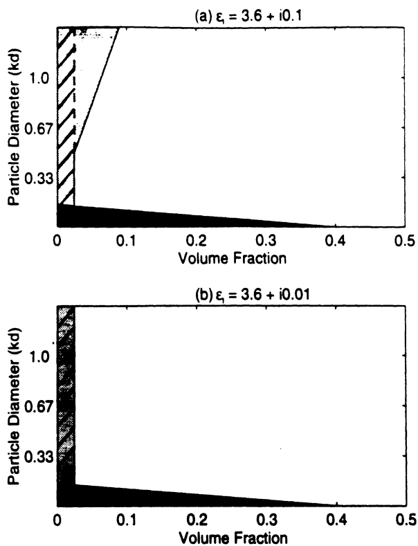
Figure 15: TE polarization validity regions based on 20% differences between imaginary \epsilon_{\text{eff}} for the numerical method of determining \epsilon_{\text{eff}} (NUM-PY) and the theoretical methods of QCA-PY (light gray), EFA (hatched) and PVS (dark gray) for (a) \epsilon_i = 3.6 + i0.1 and (b) \epsilon_i = 3.6 + i0.01 .
