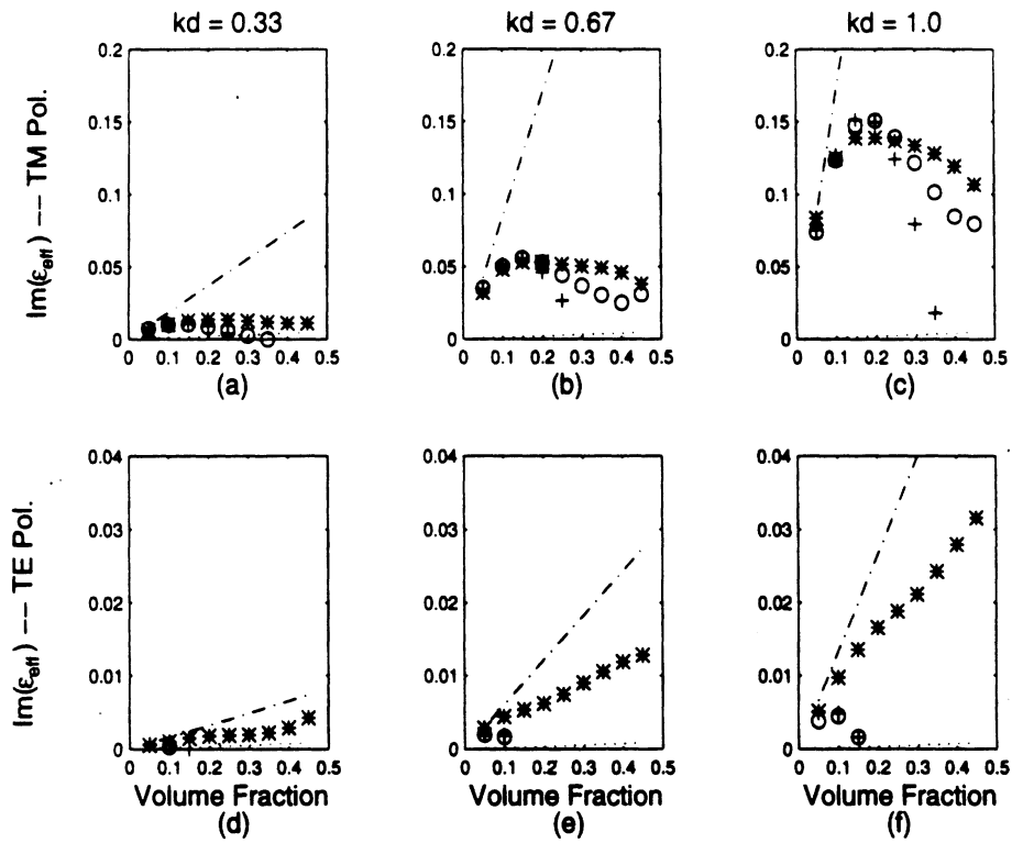
Figure 12: Comparison between five methods (QCA-PY, QCA-HC, EFA, PVS and NUM-PY) of determining the effective permittivity for TM and TE polarized fields. The permittivity of the included particles is \epsilon_i = 3.6 + i0.01 . The real component (not shown) is essentially unchanged from the previous example when \epsilon_i = 3.6 + i0.1 . See the caption in Fig. 10 for details.
