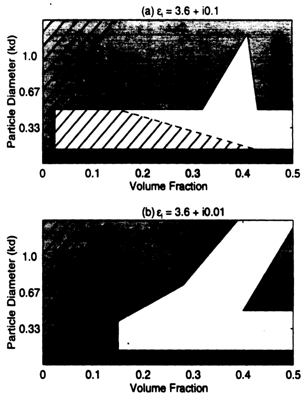
Figure 14: TM polarization validity regions based on 20% differences between imaginary \epsilon_{\text{eff}} for the numerical method of determining \epsilon_{\text{eff}} (NUM-PY) and the theoretical methods of QCA-PY (light gray), EFA (hatched) and PVS (dark gray) for (a) \epsilon_i = 3.6 + i0.1 and (b) \epsilon_i = 3.6 + i0.01 .
