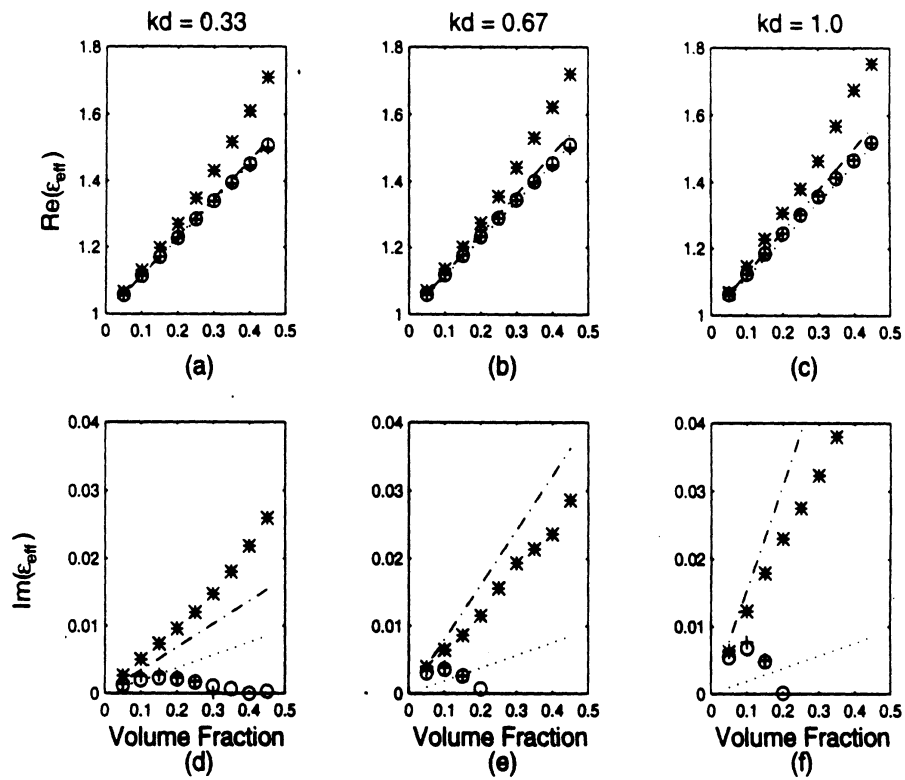
Figure 11: Comparison between five methods (QCA-PY, QCA-HC, EFA, PVS and NUM-PY) of determining effective permittivity for a TE polarized field. See the caption of Fig. 10 for details.
