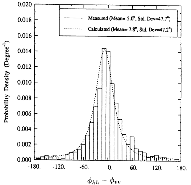
Fig. 6. The histogram and pdf of the copolarized phase difference for a rough surface with a rms height of 0.32 cm and a correlation length of 9.9 cm at C-band and at a 30^\circ incidence angle.
