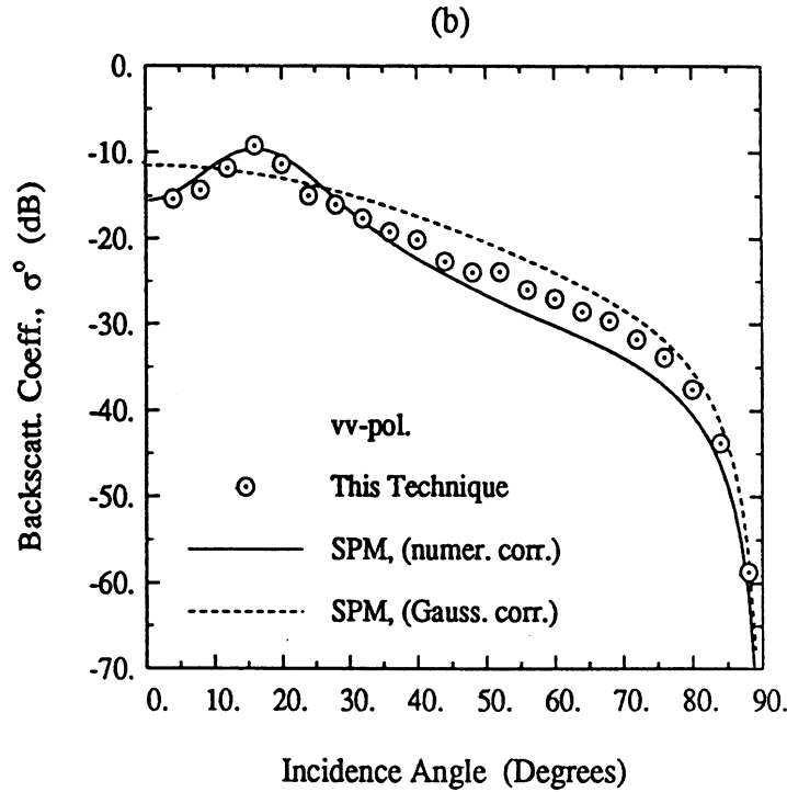
Figure 5: Backscattering coefficient \sigma^\circ of the random surface with ks = 0.12 , kl = 2.13 , and \epsilon_1 = \epsilon_2 = 15 + i3 as computed by the SPM and the numerical technique; (a) hh -polarization and (b) vv -polarization.
