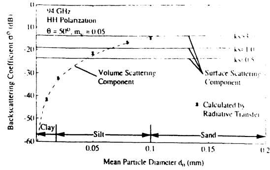
Figure 11. Variation of volume scattering component \sigma^v at 94 GHz with mean particle diameter d_0 . The level of the surface scattering component is indicated for comparison for three roughnesses.
