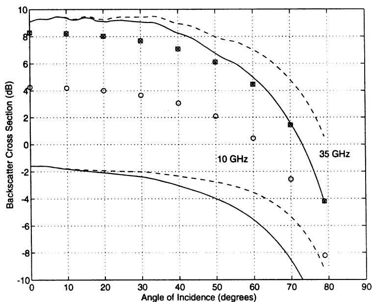
Figure 13: Results of the two-dimensional Born approximation for both 10 and 35 GHz for the Gaussian particle size distribution. Solid lines (—) are for vertical polarization, dashed (---) are for horizontal polarization and the symbols ( \circ and \boxtimes ) indicate vertically polarized results of the Born approximation using the best fit exponential (Fig. 10).
