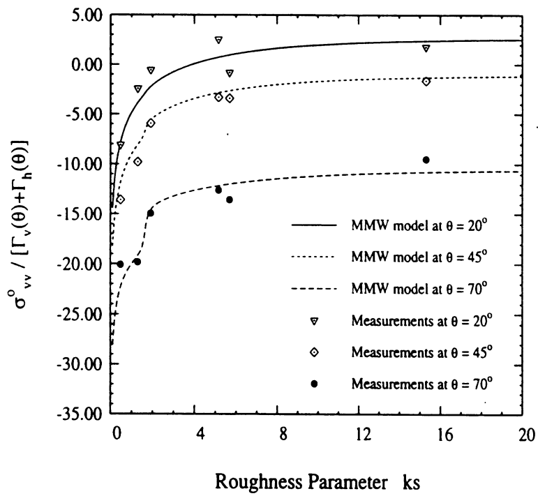
Figure 8: The sensitivity of \sigma_{vv}^o to surface roughness for wet soils at various incidence angles.
