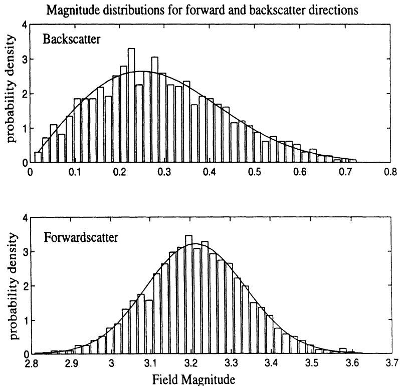
Figure 7: Forward and backscatter field magnitude distributions. Numerical simulations (bar graph) follow the Rice-Nakagami distribution (solid line). This example is for a square box of dimension 1.5\lambda \times 1.5\lambda , 40% volume fraction, TE polarization.
