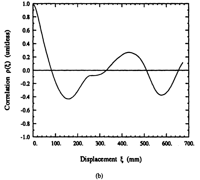
Fig. 3. Typical results of surface characterization of one of the surfaces measured in this study: (a) Histogram of measured heights for a slightly rough surface and the Gaussian probability distribution used to model it; a total of 4353 height measurements were made, from which the rms height was calculated to be s = 6.9 mm. (b) Measured autocorrelation function of the same surface.
