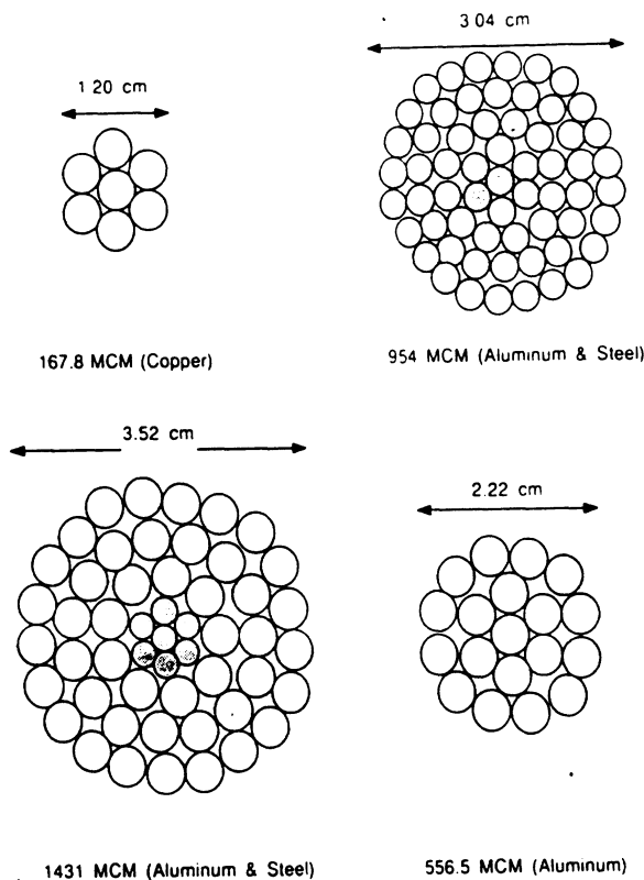
Fig. 2. Cross section of powerline samples.
