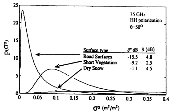
Figure 5. Probability density functions for short vegetation, road surfaces and dry snow cover at 35 GHz; \bar{\sigma}^0 (dB) and S (dB) are the mean value and associated standard deviation, both in dB, of the measured \sigma^0 (dB) distribution.
