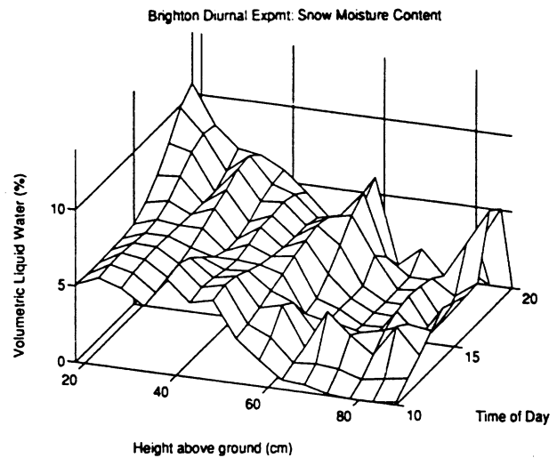
Fig. 12. Snow moisture measured via the snow probe in a 0.88-m snowpack over a diurnal cycle, shown as a function of time and height above the ground.
