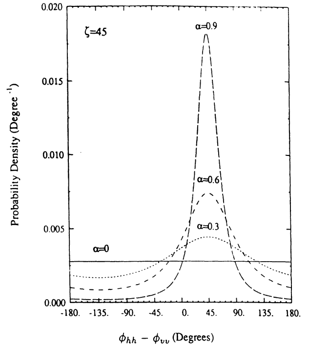
Fig. 2. The probability density function of the copolarized phase difference for a fixed value of \zeta (coherent phase difference) and four values of \alpha (degree of correlation).
