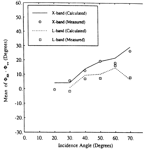
Fig. 8. Angular dependency of the mean of the copolarized phase difference for a dry rough surface with a rms height of 0.4 cm and a correlation length of 8.4 cm at L and X-band.
