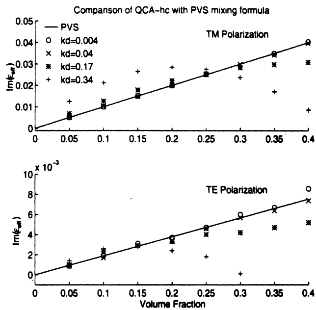
Figure 13: Performance of QCA-HC at very low frequencies. Shown is \text{Im}(\epsilon_{\text{eff}}) for particles with diameter \lambda_i/800 , \lambda_i/80 , \lambda_i/20 , and \lambda_i/10 for both TM and TE polarizations ( \epsilon_i = 3.6 + i0.1 ).
