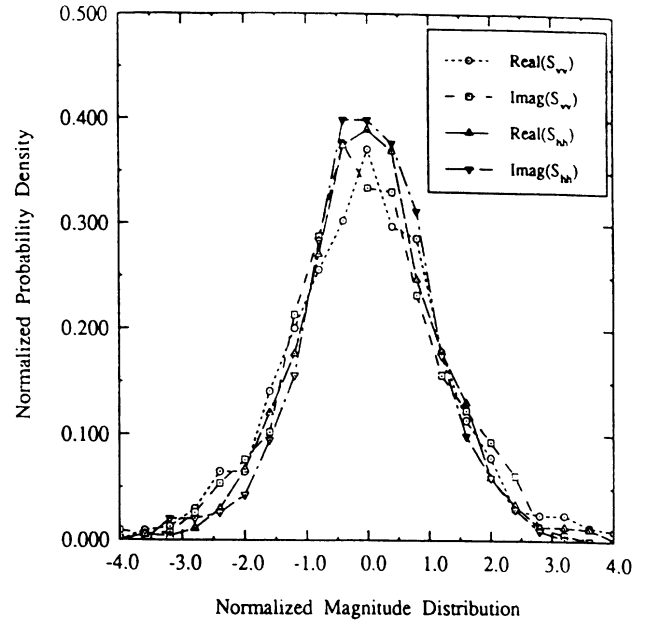
Fig. 5. The histogram of the real and imaginary parts of S_{vv} and S_{hh} for a rough surface with a rms height of 0.32 cm and a correlation length of 9.9 cm at C-band and at a 30^\circ incidence angle.
