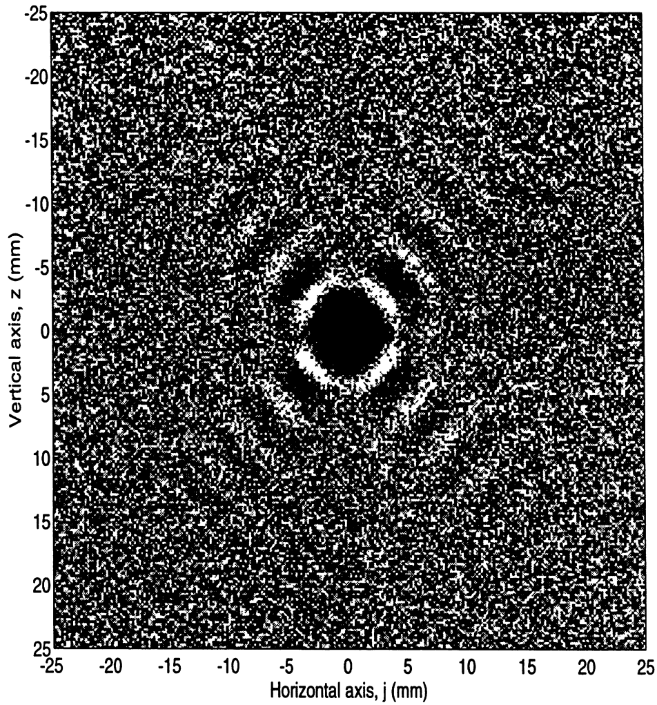
Figure 15: The pair distribution function, p(\bar{r}_j|\bar{r}_i) for the packed array shown in Fig. 4 (Gaussian size distribution). Dark areas indicate low probability and bright areas indicate high probability of finding another particle at \bar{r}_j given a particle at \bar{r}_i .
