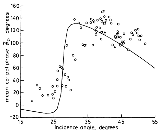
Fig. 9 Measured and calculated mean co-polarised phase angle for corn fields observed by a 1.2 GHz SAR system
