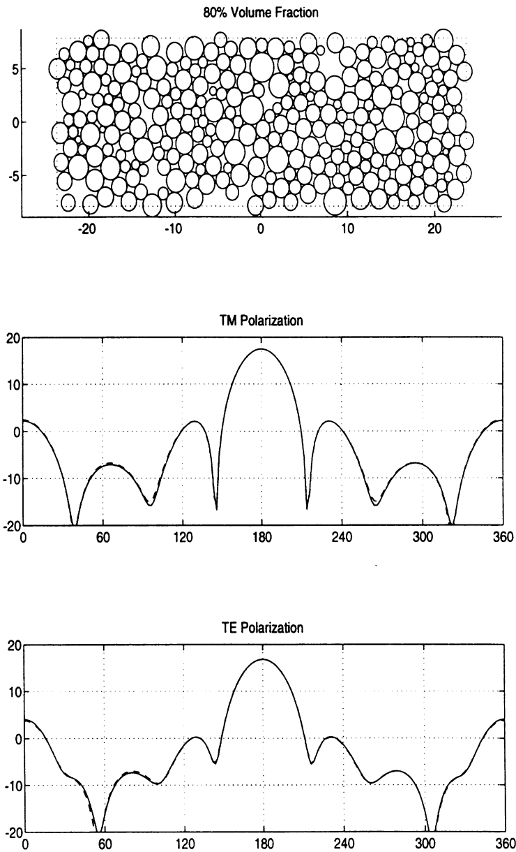
Figure 3: Algorithm results for 80% volume fraction. See Fig. 2 for description of individual sub-figures.
