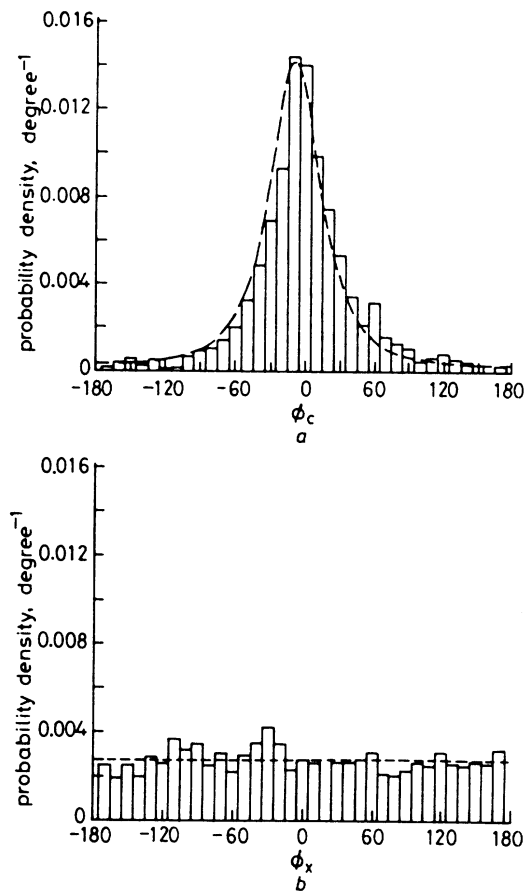
Fig. 4 Measured and calculated probability density functions
