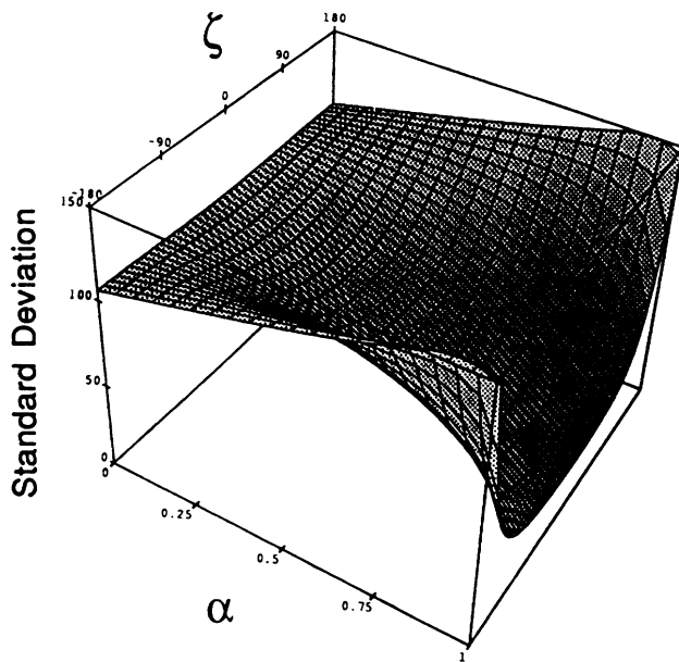
Fig. 4. The standard deviation of the copolarized phase difference as a function of \alpha (degree of correlation) and \zeta (coherent phase difference).
