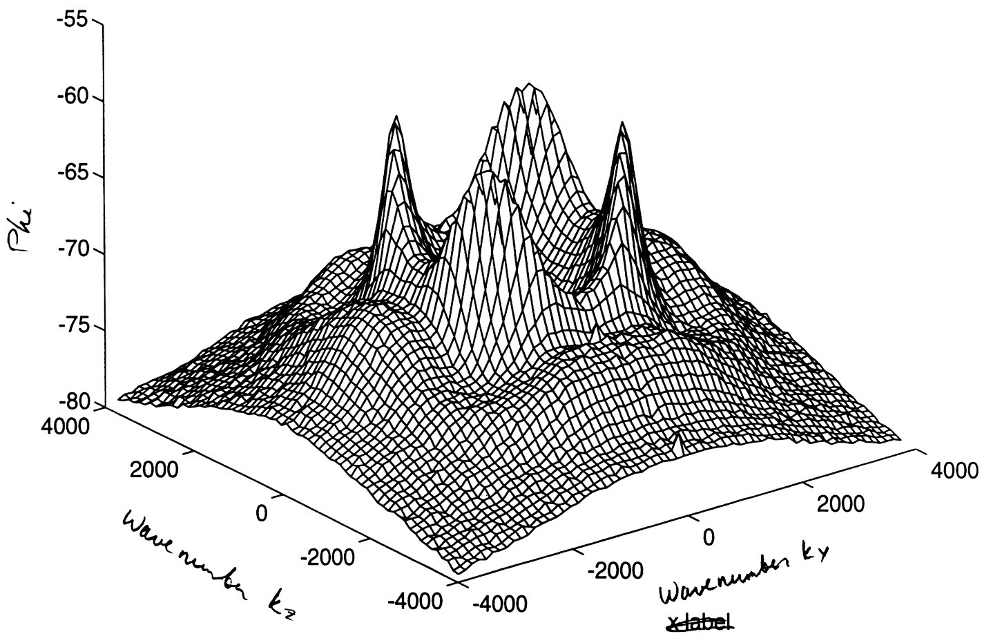
Figure 9: The power spectral density derived from data shown in Fig. 4. Strong peaks along the diagonal highlight the periodicity in the correlation function seen along this axis. Arcs drawn along a constant radius are proportional to the backscatter intensity as a function of incidence angle.
