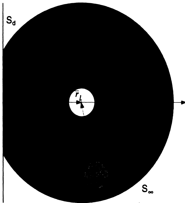
Figure 1: Domain of integration. Shown are the three surfaces ( S_d , S_e , and S_\infty ) and their inward pointing surface normals for the integral in (18).
