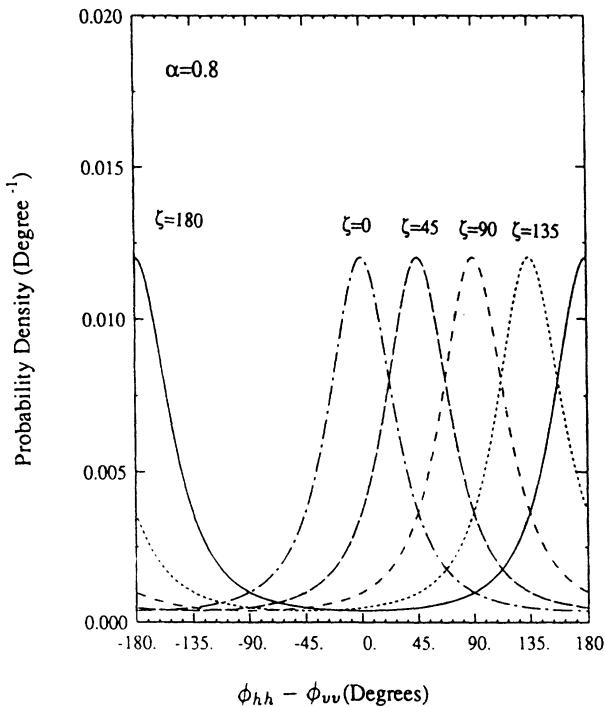
Fig. 1. The probability density function of the copolarized phase difference for a fixed value of \alpha (degree of correlation) and five values of \zeta (coherent phase difference).
