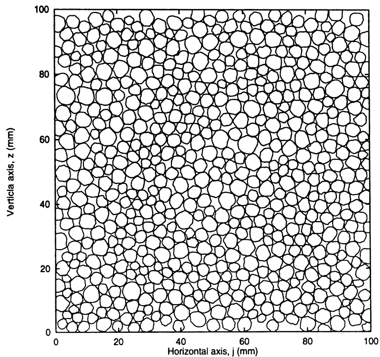
Figure 6: Demonstration of the packing algorithm for two-dimensional rocks. Rock surfaces are generated by a random walk about a uniform radius 2\text{mm} \pm 0.4\text{mm} . This particular simulation took approximately 30 seconds on a Sun 10 Workstation.
