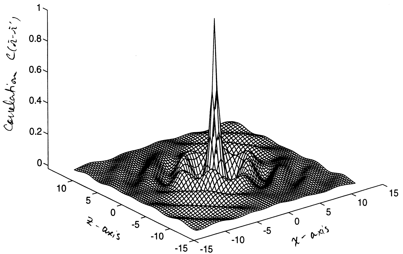
Figure 8: Two-dimensional correlation function for the particles in Fig 4. The correlation function is not axially symmetric.
