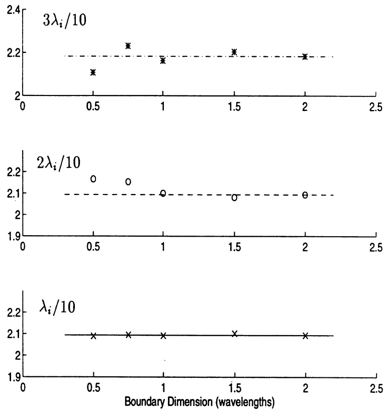
Figure 10: Real part of effective permittivity versus boundary dimension for three different particle sizes: \lambda_i/10 - \times , 2\lambda_i/10 - o , 3\lambda_i/10 - * and a volume fraction of 40%, TM polarization.
