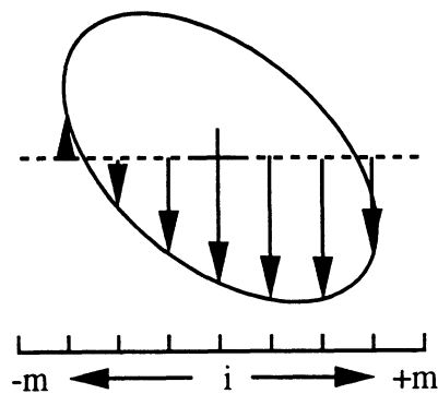
Figure 2: Illustration of the lower surface of a particle, M_p^{\text{lower}} . The particle is discretized into a horizontal grid and the maximum and minimum heights of the particle at points on the grid define the upper and lower surfaces.
