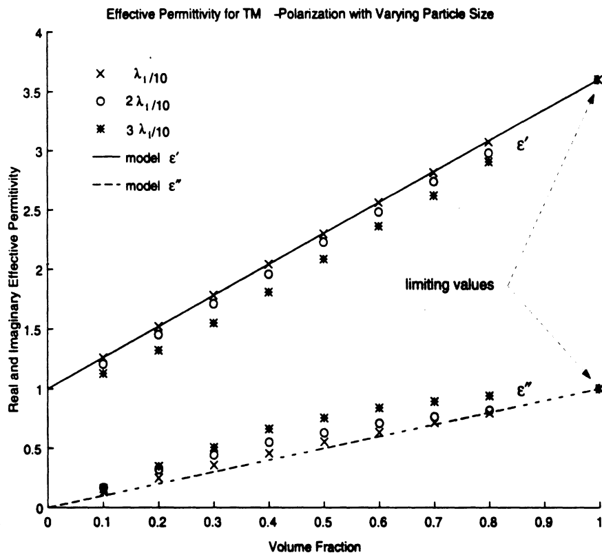
Figure 8: Effective permittivity, \epsilon_{\text{eff}} , vs. volume fraction for a TM polarized field incident upon a random medium. Shown are results from the numerical method for different particle sizes along with those obtained by the Polder-Van Santen mixing formula. The volume fraction was adjusted by particle extraction.
