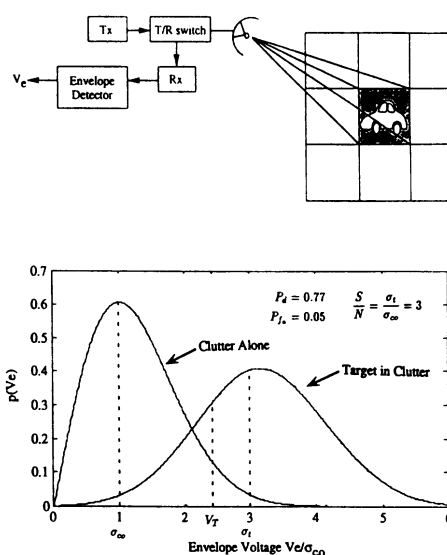
Figure 1. Probability density functions for clutter alone and clutter with a target with RCS = 5 dB above the average clutter cross section, \sigma_{co} .
