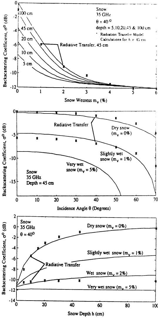
Figure 8. Variation of \sigma^o with incidence angle \theta , snow depth h and liquid water content m_v at 35 GHz.
