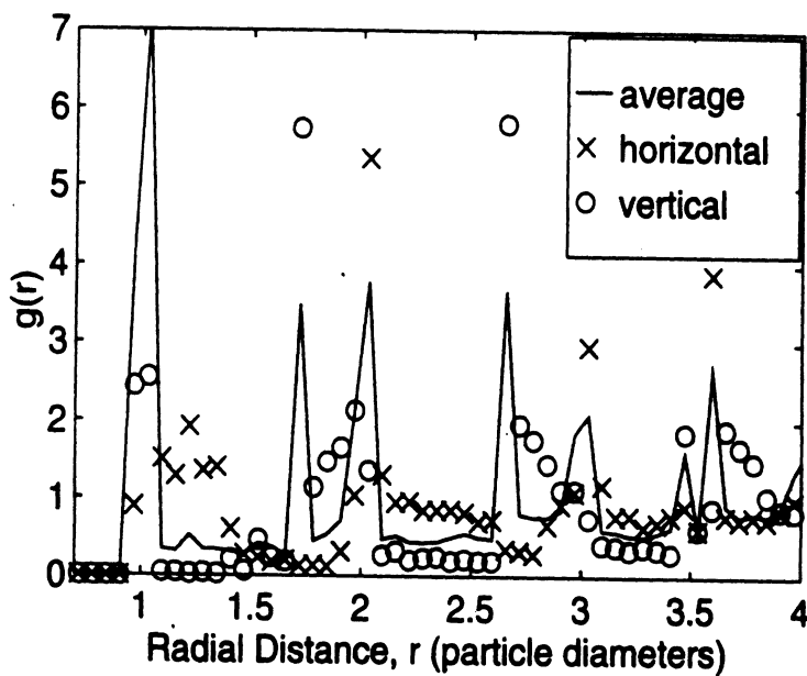
Figure 3: Particle arrangement simulation using particle extraction from a near perfect lattice for a volume fraction of 30%. Shown is the average pair distribution function over all angles and the pair distribution function from the vertical and horizontal directions which accentuate the azimuthal asymmetry. Because the basic structure of the lattice remains unchanged for different volume fractions, the pair distribution function does not change with particle number density.
