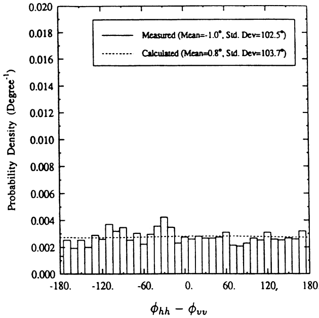
Fig. 7. The histogram and pdf of the cross-polarized phase difference for a rough surface with rms height of 0.32 cm and correlation length of 9.9 cm at C-band and at a 30° incidence angle.
