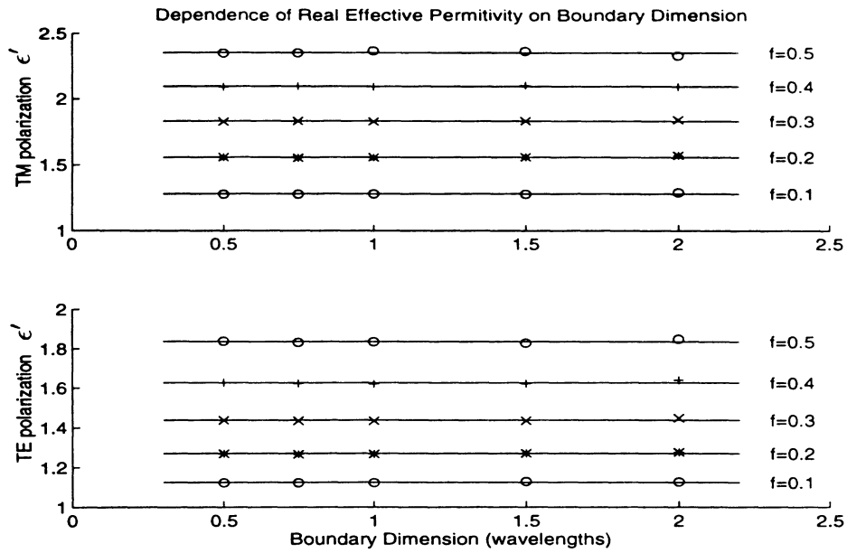
Figure 6: Solution dependence on boundary dimension for TM and TE polarizations. Different lines on the graph represent the average permittivity for a given volume fraction of f = 0.1, 0.2, 0.3, 0.4 or 0.5 .
