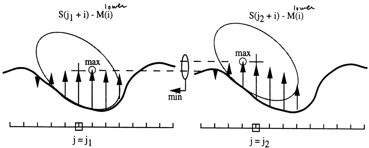
Figure 3: Illustration of equation (4) for two different points ( j_1, j_2 ) on the surface S(j) . The dilation of the surface is shown for each point on the surface where the maximum is highlighted by a circle. This is the height of where the center of the ellipse would lie for a given horizontal location, j . The minimum of these heights defines the point of minimum potential energy.
