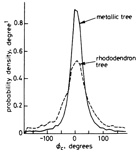
Fig. 11 Measured f(\phi_c) for a rhododendron tree and an artificial metallic tree at 35 GHz
