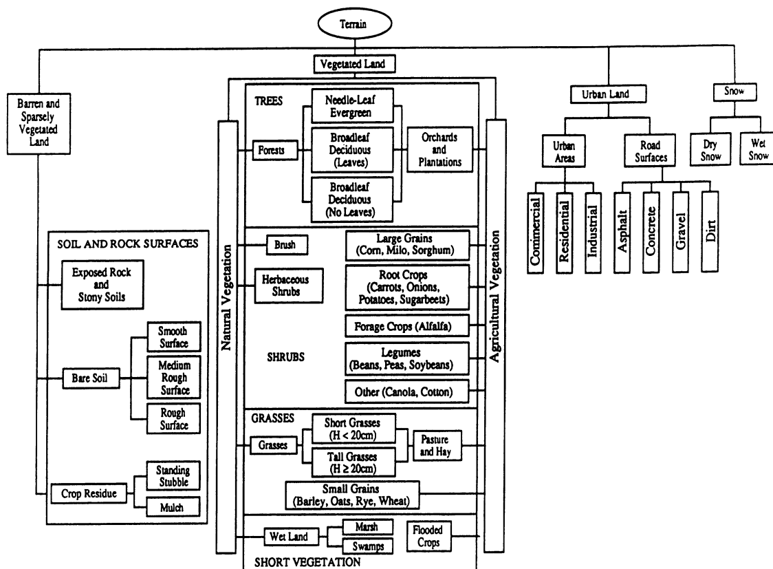
Figure 3. Radar terrain classification system.
