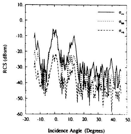
Fig. 11. Radar backscatter cross section of curved 30 cm long cable 2 at 34.5 GHz versus incidence angle (radius of curvature \approx 10 cm).
