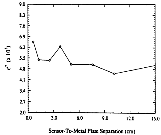
Fig. 5. Variation in measurement of \epsilon'' of sugar as a function of sensor proximity to metal plate. (Real part \epsilon' stayed in the range 2.00–2.01.)
