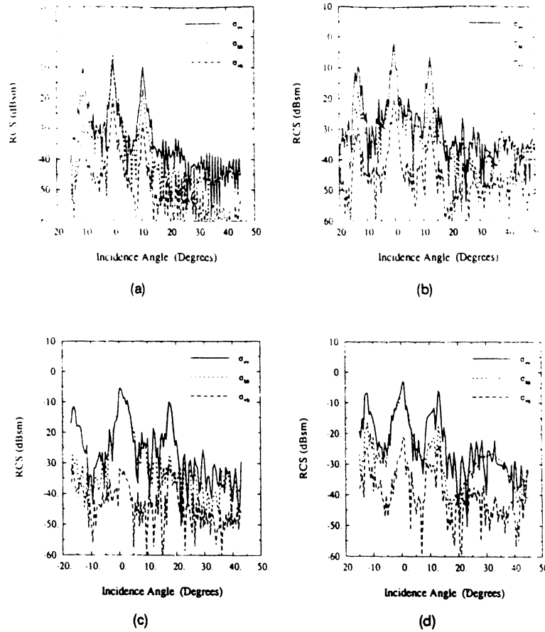
Fig. 9. Radar backscatter cross section for 30 cm long cable. (a) Cable 1. (b) Cable 2. (c) Cable 3. (d) Cable 4 at 34.5 GHz.
