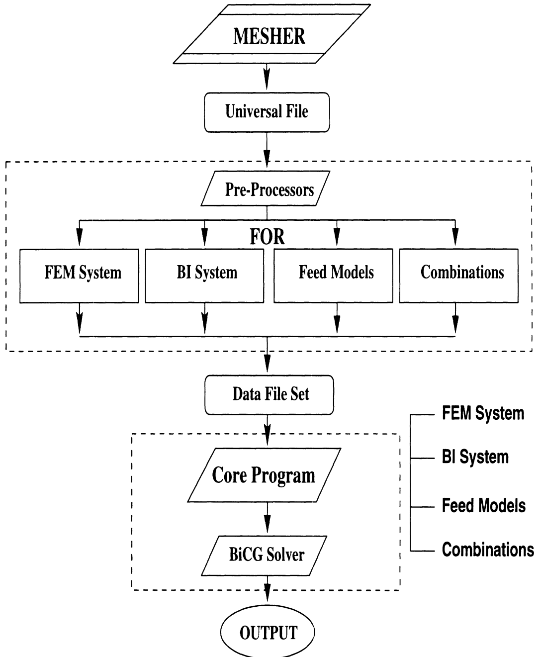
Figure 3.5: A flow chart describes the major implementation procedures from the mesh generation, a few data preprocessors, the FE–BI kernel, to the BiCG solution and finally the data output.
