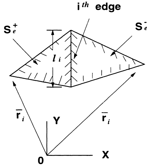
Figure 3.3: Pair of triangles sharing the i th edge
