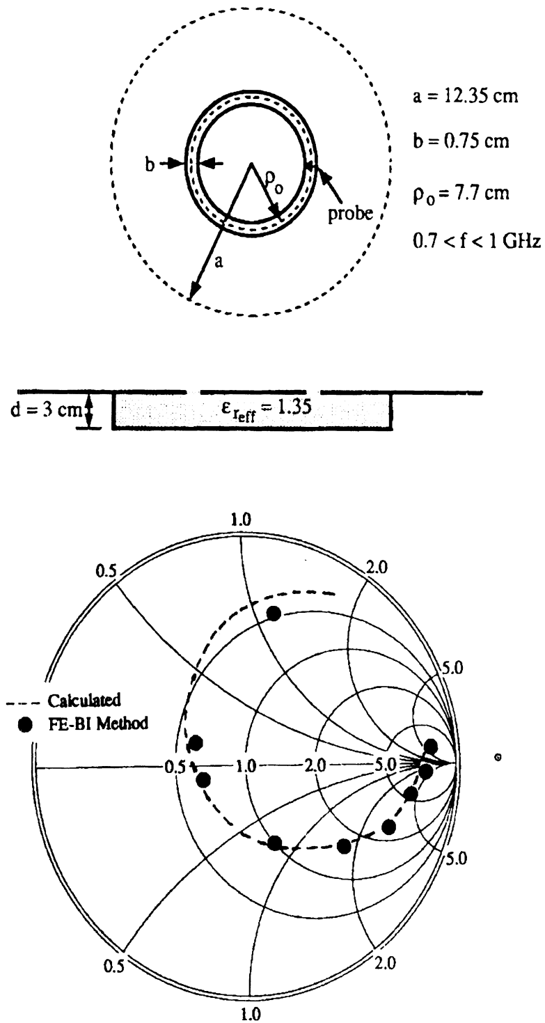
Figure 3.10: Comparison of input impedance calculations for the illustrated cavity-backed slot.
