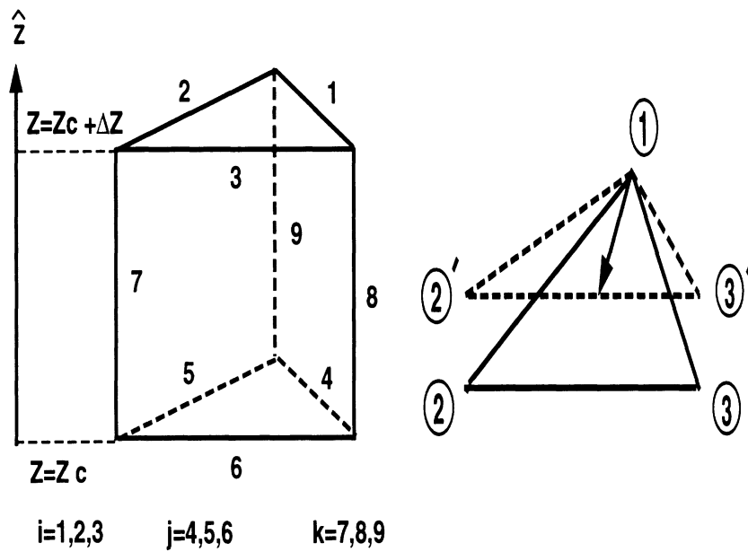
Figure 5.3: Right angled prism
