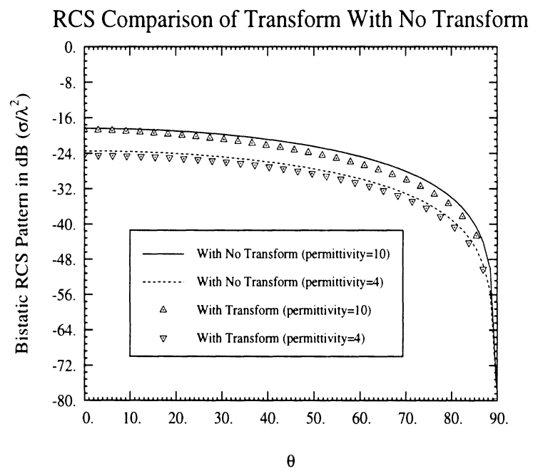
Figure 4.9: Bistatic RCS scattering by a circular patch antenna modeled using the regular BiCG FE-BI and the BiCG-FFT algorithm with overlaying transform.
