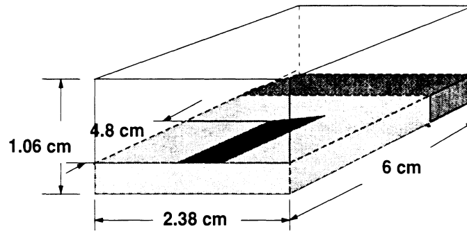
Figure 8.1: Illustration of the shielded microstrip stub excited with a current probe.
