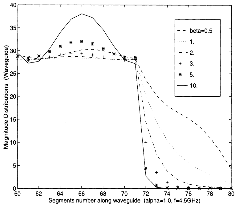
Figure 7.6: Field values of the TE 10 mode inside a waveguide terminated by a perfectly matched uniaxial layer. The absorber is 10 elements thick and each element was 0.5 cm which translates to about 13 samples per wavelength at 4.5 GHz.
