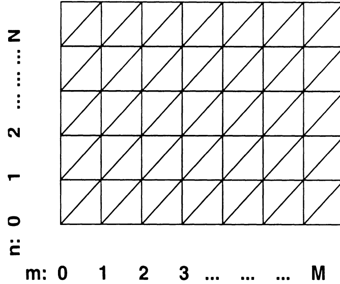
Figure 4.1: Structured mesh consists of equal right triangles
