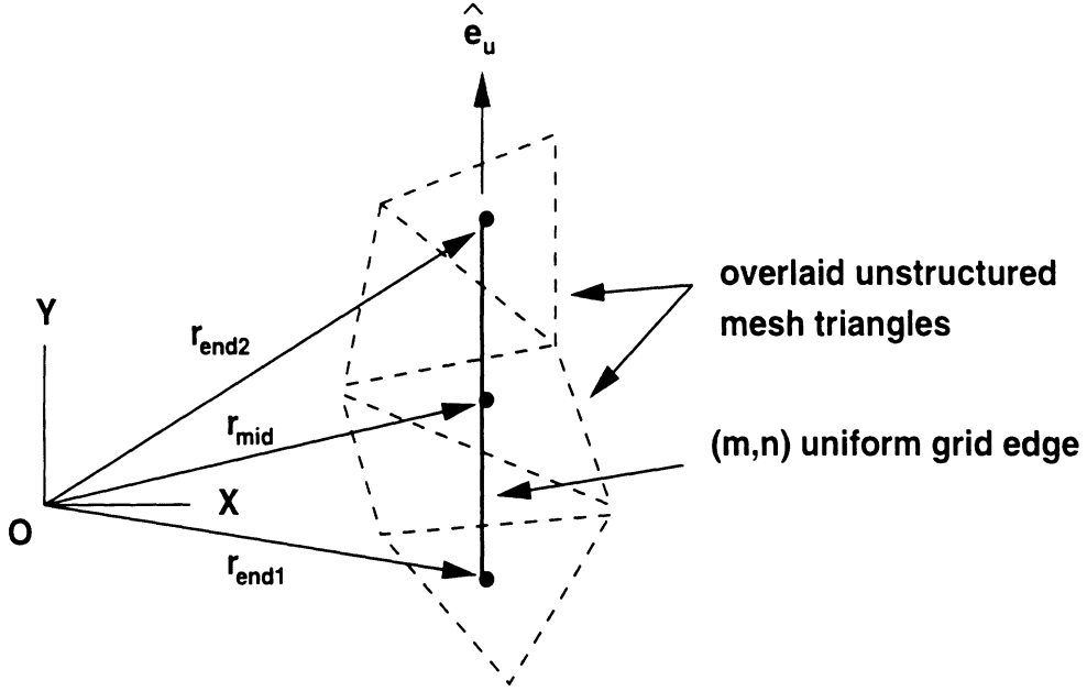
Figure 4.5: Illustration of the parameters and geometry used in constructing the transformation matrix elements between the structured and unstructured mesh.
