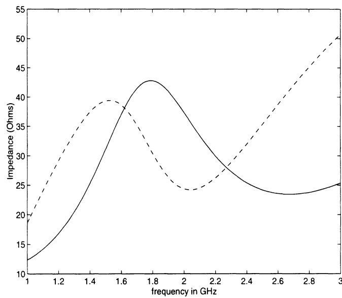
Figure 8.2: Impedance calculations using traditional FEM frequency analysis for a shielded microstrip stub shown in figure 8.1. Solid line is the real part and the dashed line denotes the imaginary part of the solutions. These computations are used as reference for comparisons.
