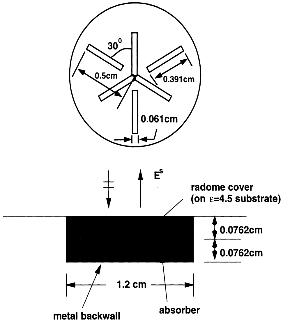
Figure 5.6: Illustration of the setup for computing the FSS transmission coefficient Upper figure: periodic element (top view); Lower figure: periodic element in cavity (cross-sectional view)
