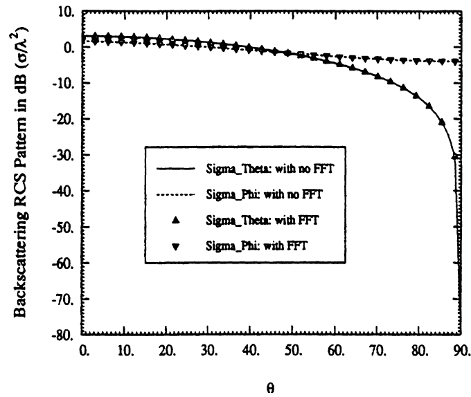
Figure 4.7: Comparisons of the monostatic radar cross section scattering by a 2 \times 2 triangular patch array shown in fig. 4.6. The results were computed using the regular BiCG FE-BI technique described in chapter 3 and using the BiCG-FFT proposed in this chapter.
