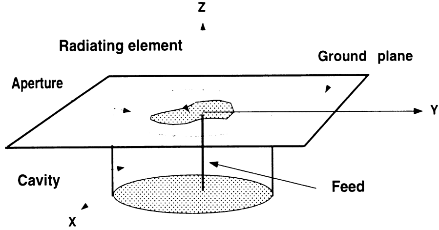
Figure 2.1: Illustration of a typical conformal antenna configuration.
