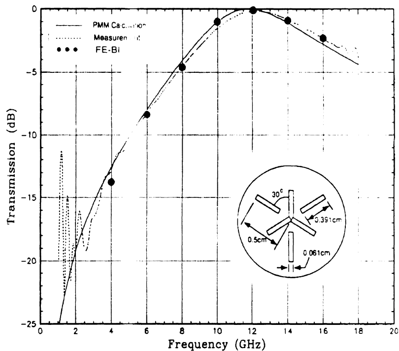
Figure 5.7: Calculations and comparisons of transmission through the FSS structure shown in fig. 5.6
