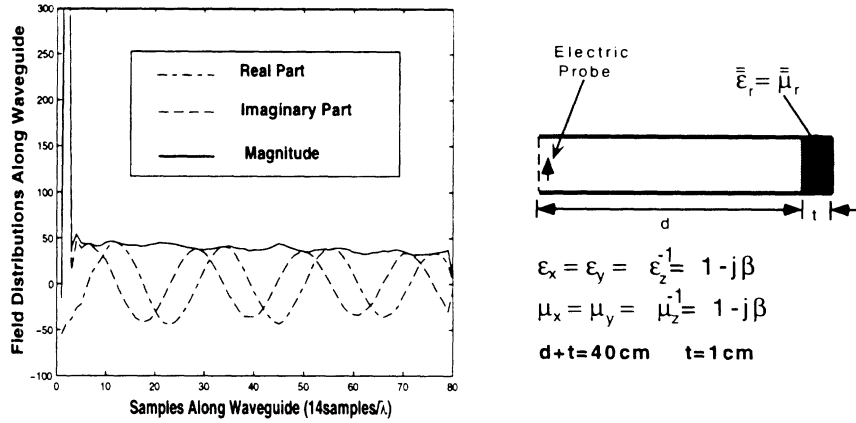
Figure 7.5: Typical field values of TE 10 mode inside a rectangular waveguide terminated by a perfectly matched uniaxial layer.
