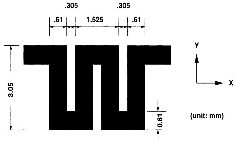
Figure 7.12: Illustration of a meander line geometry used for comparison with measurement.
