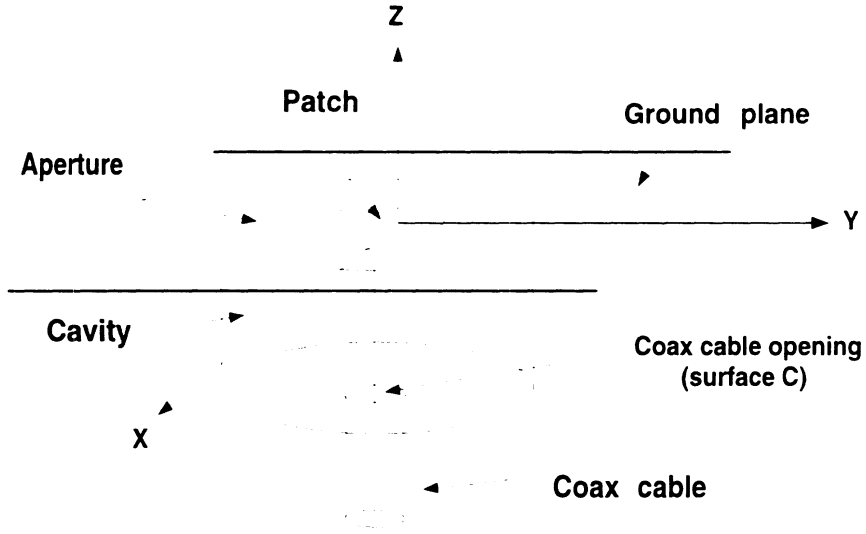
Figure 3.1: Illustration of a typical radiation and scattering problem.
