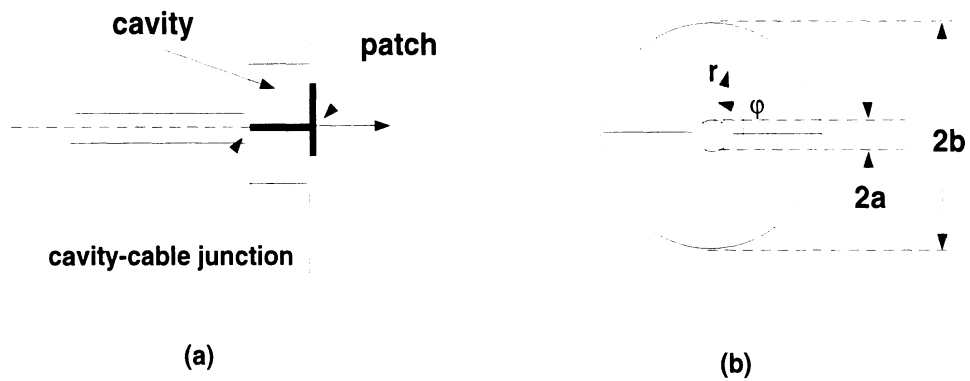
Figure 6.4: (a) Side view of a cavity-backed antenna with a coax cable feed; (b) Illustration of the FEM mesh at the cavity-cable junction (the field is set to zero at the center conductor surface).
