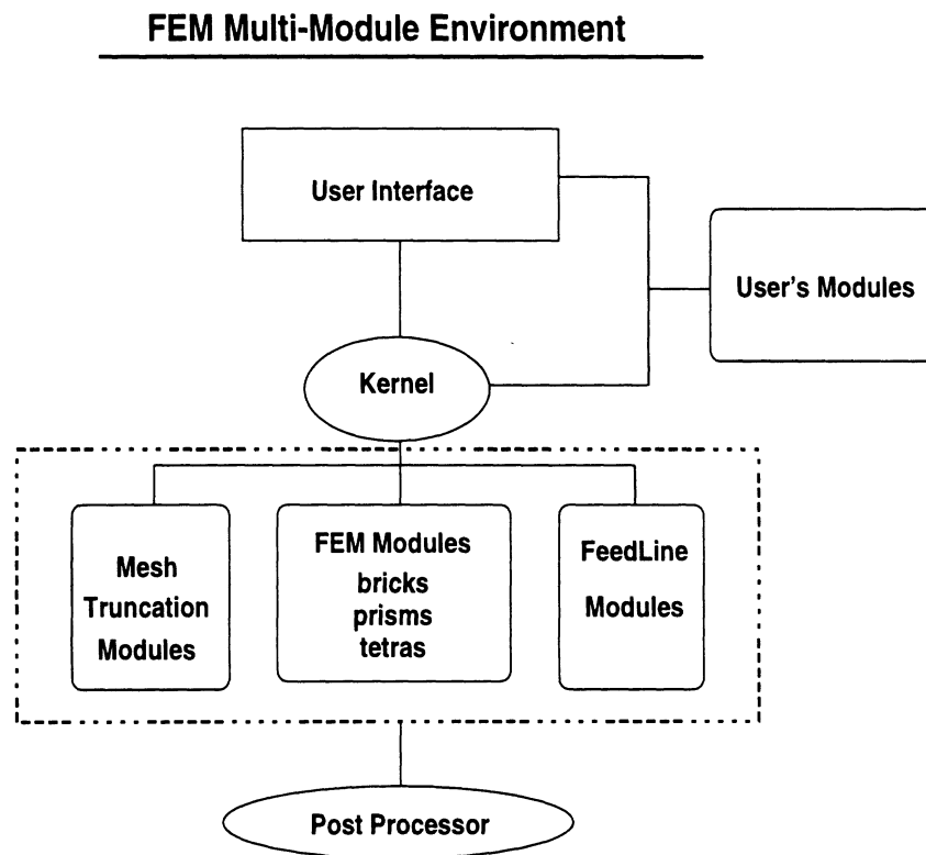
Figure 9.1: Multi-modular FEM environment
