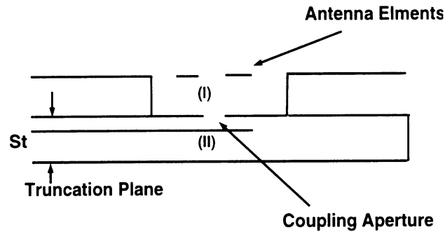
Figure 6.1: Cross-section of an aperture coupled patch antenna, showing the cavity region I and the microstrip line region II for two different FEM computation domains.
