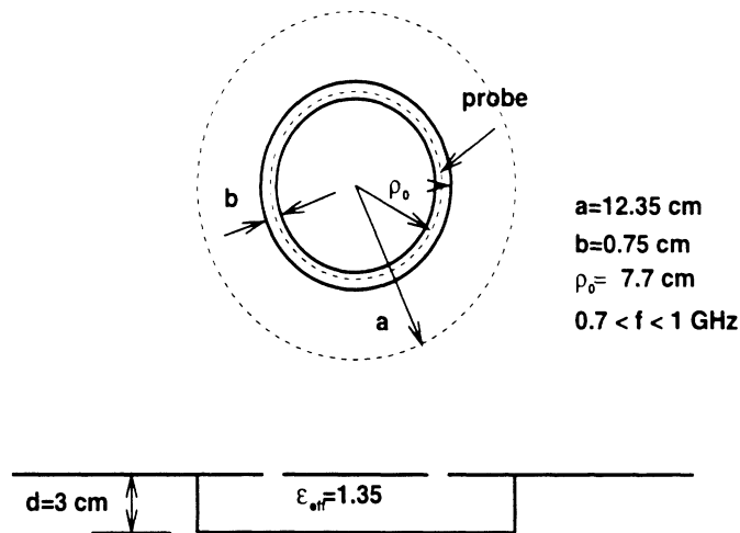
Figure 5.4: Geometry of the annular slot antenna backed by a cavity 23.7 cm in diameter and 3 cm deep
