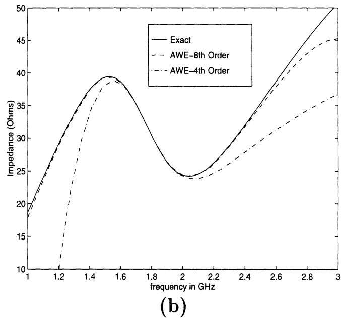
Figure 8.3: 4th order and 8th order AWE implementations using one point expansion at 1.78 GHz are shown to compare with the reference data. With the 4th order AWE solutions, 56% and 33% bandwidth agreement can be achieved for the real (a) and imaginary (b) parts of impedance computations, respectively. It is also shown that the 8th order solutions agree excellently with the reference data over the entire band. (a) Real Part (b) Imaginary Part computations
