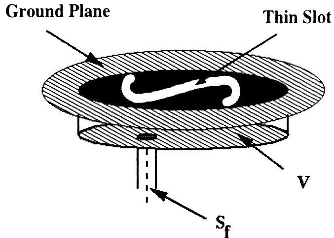
Figure 5.1: Geometry of cavity-backed microstrip antennas
