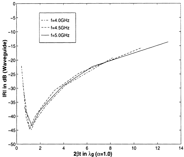
Figure 7.7: Reflection coefficient vs 2\beta t/\lambda_g ( \alpha = 1 ) for the perfectly matched uniaxial layer used to terminate the waveguide shown in fig. 7.6.
