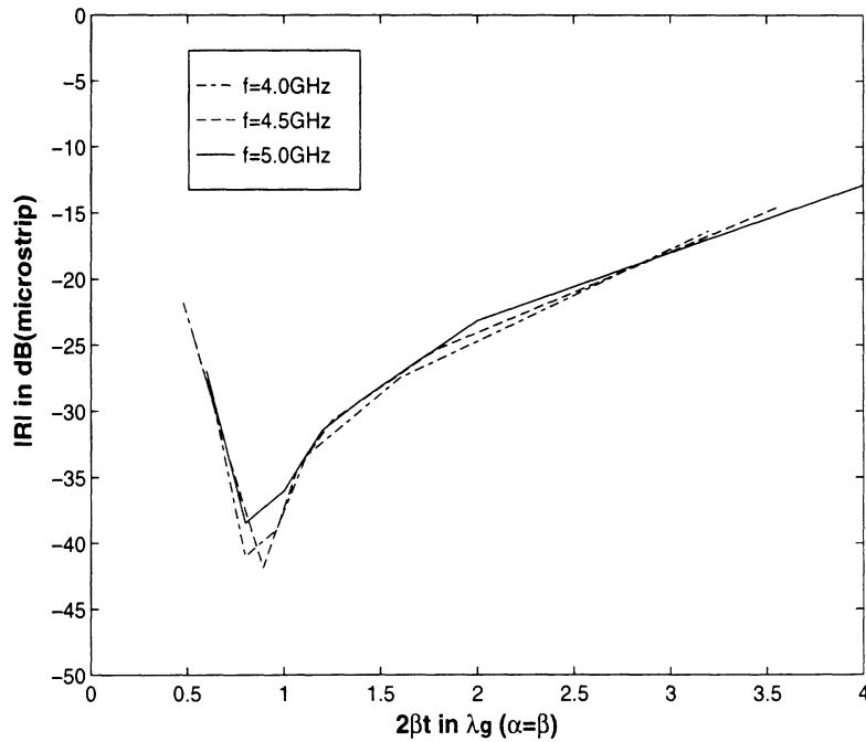
Figure 7.10: Reflection coefficient vs 2\beta t/\lambda_g with \alpha = \beta , for the shielded microstrip line terminated by the perfectly matched uniaxial layer.
