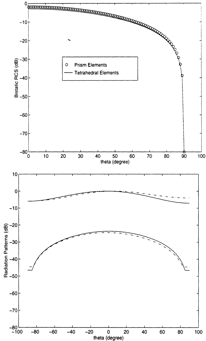
Figure 5.5: Scattering: Bistatic (co-pol) RCS patterns computed using the tetrahedral FE-BI code and the prismatic FE-BI code. The normally incident plane wave is polarized along the \phi = 0 plane and the observation cut is perpendicular to that plane. Radiation: X-pol and Co-pol radiation patterns in the \phi = 0 plane from the annular slot antenna shown in fig. 5.4. The solid lines are computed using the tetrahedral FE-BI code whereas the dotted lines are computed using the prismatic FE-BI code. The excitation probe is placed at the point ( y=0 ) marked in fig. 5.4.
