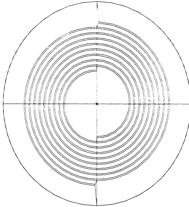
Figure 5.9: Illustration of a typical 2-arm slot-spiral design
