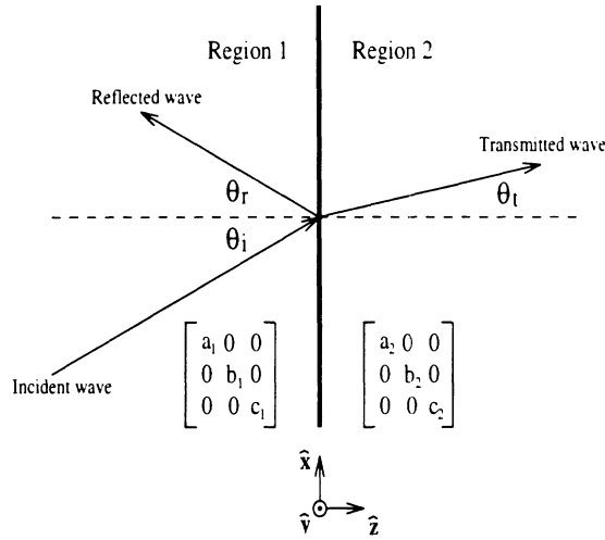
Figure 7.4: Plane wave incidence on an interface between two diagonally anisotropic half-spaces.
