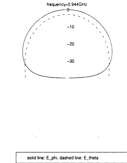
Figure 5.11: Radiation Pattern at f=0.944\text{GHz} (lower end of frequency range). It can be seen that the axial ratio of the pattern becomes larger compared to that at the center frequency, but still remains within 3dB for a wide angle range. This indicates that the number of the outer turns in the spiral contour design is most likely sufficient.
