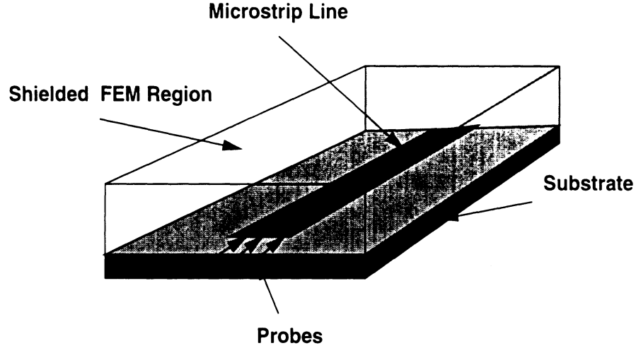
Figure 7.1: Illustration of a shielded microstrip line.
