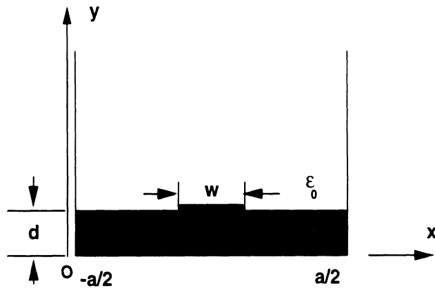
Figure 7.2: Illustration of the cross section of a shielded microstrip line.
