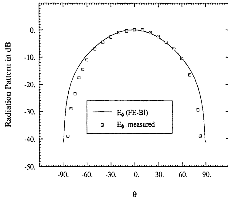
Figure 3.9: Comparison of the calculated radiation pattern ( E_\phi ), taken in the \phi = 90^\circ -plane, with data in reference [35] for the one-arm conical spiral shown in fig. 3.8
