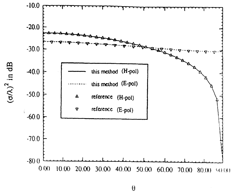
Figure 4.8: Comparisons of the monostatic radar cross section scattering by an empty aperture with the same cavity size and dielectric filling ( \epsilon_r=1 ) as the structure shown in fig. 4.6. Again, the results were calculated using the regular BiCG FE-BI technique described in chapter 3 and using the BiCG-FFT proposed in this chapter.
