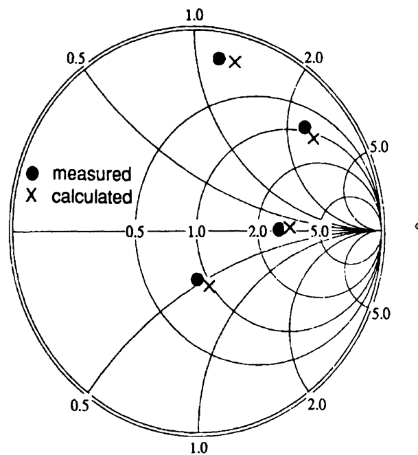
Figure 3.7: Comparison of the computed and measured input impedance for the circular patch shown in fig. 3.6. The feed was placed 0.8 cm from the center of the patch and the frequency was swept from 3 to 3.8 GHz.
