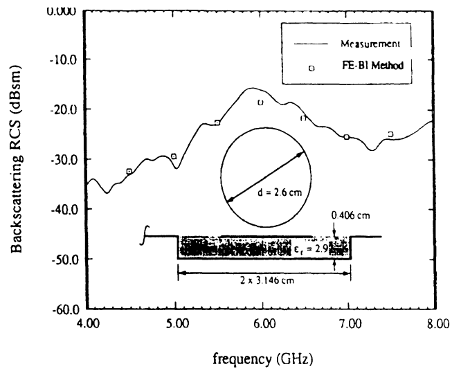
Figure 3.6: Comparison of the computed and measured \sigma_{\theta\theta} backscatter RCS as a function of frequency for the shown circular patch. The incidence angle was 30^\circ off the ground plane.
