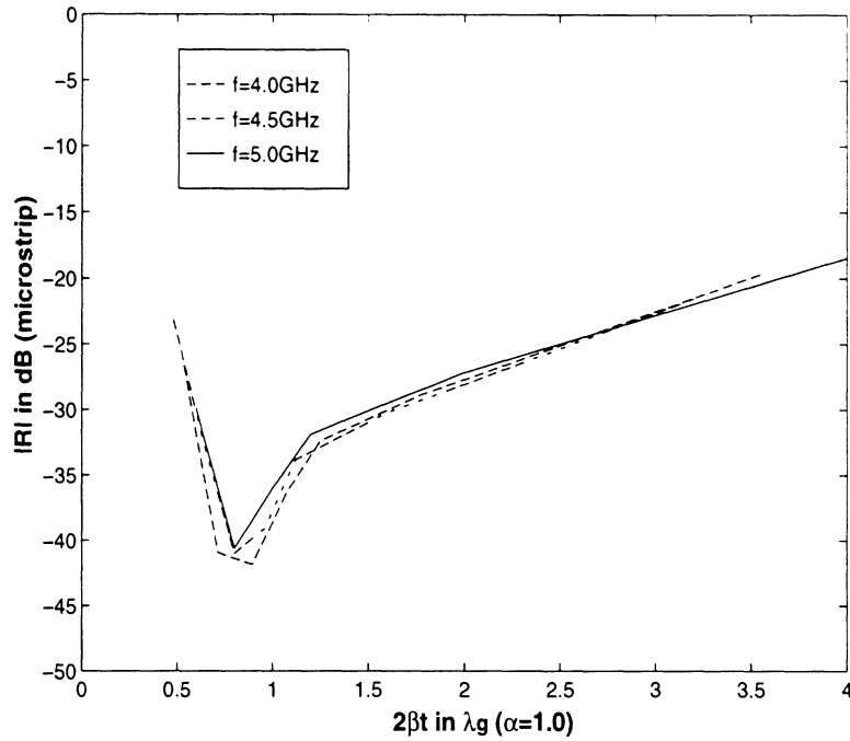
Figure 7.9: Reflection coefficient vs 2\beta t/\lambda_g with \alpha=1 , for the shielded microstrip line terminated by the perfectly matched uniaxial layer.
