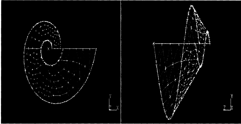
Figure 3.8: Illustration of the configuration and mesh of the one-arm conical spiral used for the computation of fig. 3.9.
