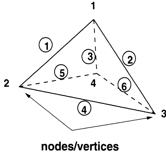
Figure 3.2: A tetrahedron and its local node/edge numbering scheme
