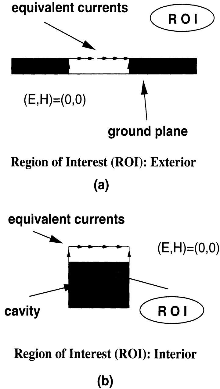
Figure 1.3: Illustrations of equivalence principle when applied to the structure shown in fig. 1.1b.
