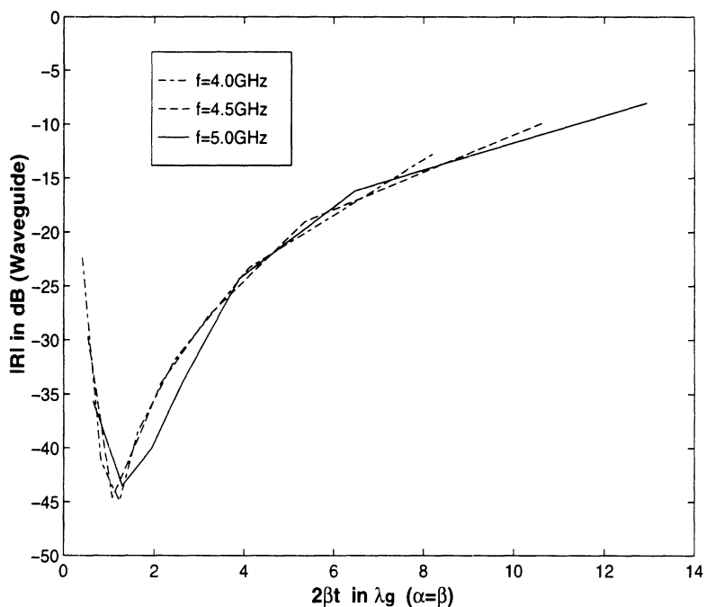
Figure 7.8: Reflection coefficient vs 2\beta t/\lambda_g , with \alpha = \beta , for the perfectly matched uniaxial layer used to terminate the waveguide shown in fig. 7.6.
