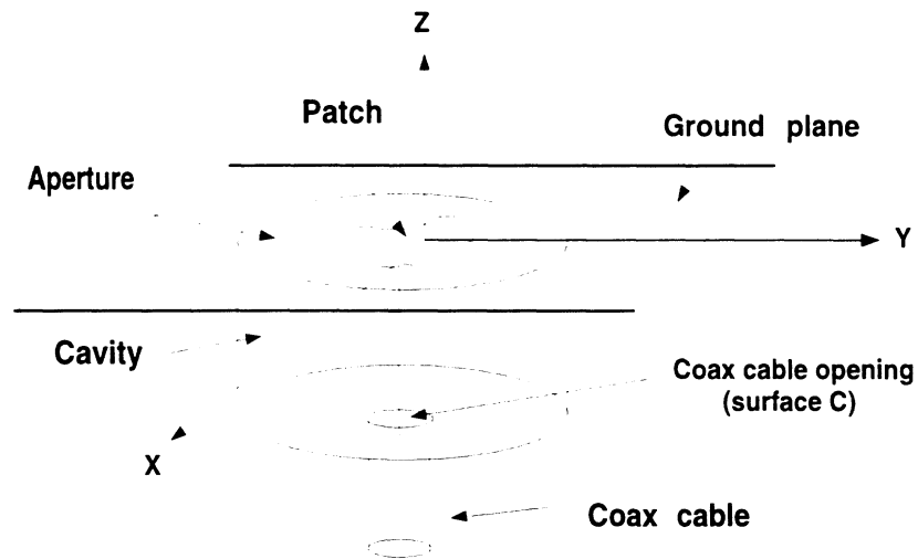
Figure 6.3: Illustration of a cavity-backed patch antenna with a coax cable feed.
