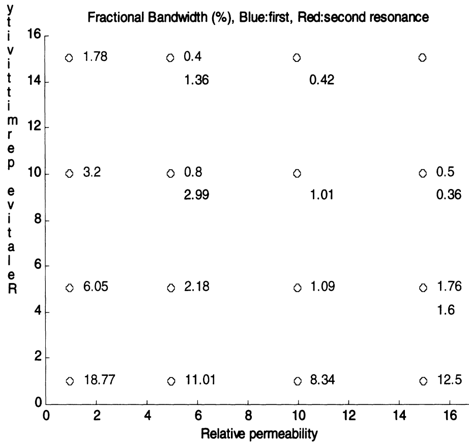
Figure 4: Variation of the fractional bandwidth for the primary (blue) and secondary (red) resonances in the \mu - \epsilon (permeability-permittivity) plane.
