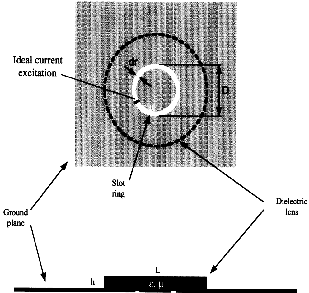
Figure 1: Geometry of the slot-ring radiator loaded with a finite magnetic dielectric lens. h=1.5\text{cm} , L = 6\text{cm} , D=3\text{cm} , r_d=0.2\text{cm} .
