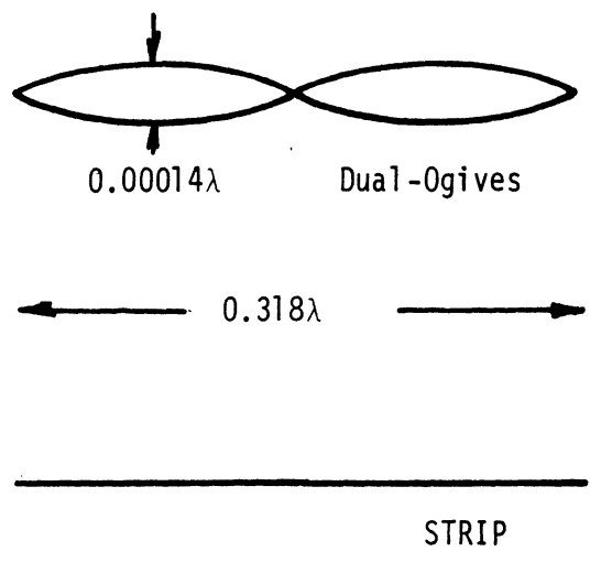
Fig. C1. Models used for testing RESTE and RESTH.
