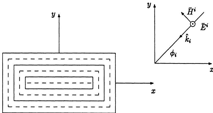
Fig. 1. Dielectric cylinder with strips placed at the geometric center of each layer
