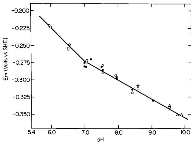
Fig. 2. Potential vs. pH diagram for 3 \cdot 10^{-5} M deazariboflavin in 0.1 M buffers at 25^{\circ}\text{C} . \circ indicates equilibrium measurements made with riboflavin, \bullet indicates values obtained from potentiometric measurements with lumiflavin 3-acetate, \triangle indicates redox potentials determined by equilibration with flavodoxin, \triangle indicates value at pH 8.6 determined by Fisher, Spencer and Walsh [4]. SHE, standard hydrogen electrode.
