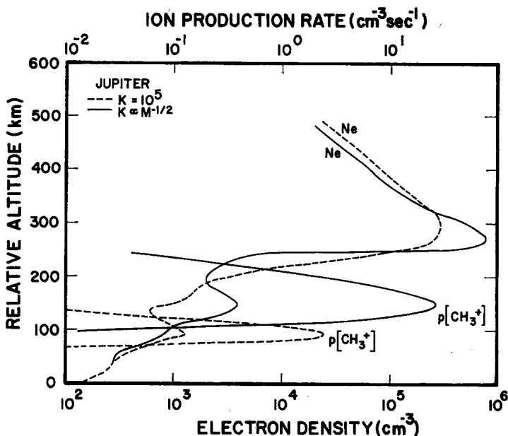
FIG. 2. Jupiter's model ionosphere with K = 10^5 \text{ cm}^2 \text{ sec}^{-1} and K \propto M^{-1/2} . \text{CH}_3^+ ion production rates, p[\text{CH}_3^+] , for the two models are given by the upper scale. Height scale is the same as in Fig. 1.
