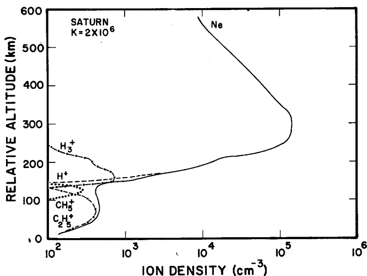
FIG. 1. A model for Saturn's ionosphere with eddy diffusion coefficient, K = 2 \times 10^6 \text{ cm}^2 \text{ sec}^{-1} . The vertical scale gives the height above a reference level where the hydrogen density is 10^{16} \text{ molecules cm}^{-3} .
