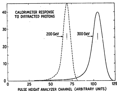
Fig. 4. The pulse-height spectra from 200 and 300 GeV protons incident on the calorimeter.
