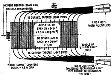
MICHIGAN NEUTRON CALORIMETER
