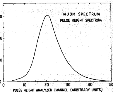
Fig. 2. A muon pulse-height spectrum taken with the calorimeter. The numbers on the abscissa scale differ by a factor of 25.3 from those of figs. 3 and 4.
