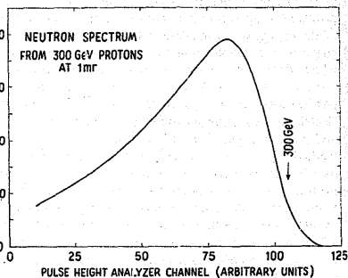
Fig. 3. A typical pulse-height spectrum of neutrons produced by 300 GeV protons on a ^{12}\text{C} beryllium target at 1 mr.
