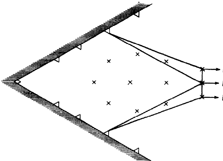
Fig. 10. Optimal truss, with twelve interior nodes and nine support nodes.
