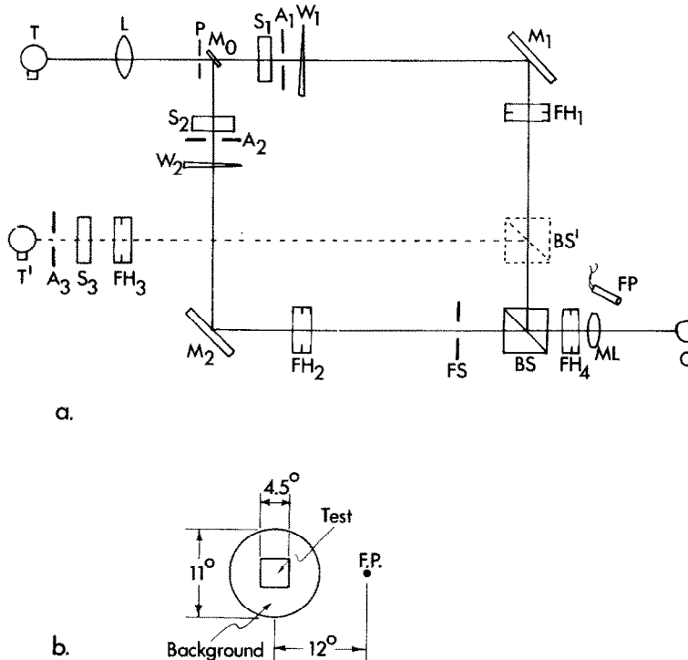
Fig. 1. (a) The Maxwellian view system. See text for details. (b) The observer's view in the apparatus. The test patch was 4.5^\circ square, and was centered on the 11^\circ background field. The fixation point (F.P.) was 12^\circ to the right of the field.
