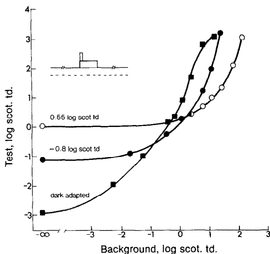
Fig. 9. Transient rod saturation, measured against steady preadapting fields. Pre-adapting field and flashed background were red (Wratten No. 26); 30 msec test was blue (480 nm). Pre-adapting field intensities were 0.55 log scot. td (open circles) or -0.8 log scot. td (solid circles) also shown is the case of no pre-adapting field (solid squares). Subject E.A.
