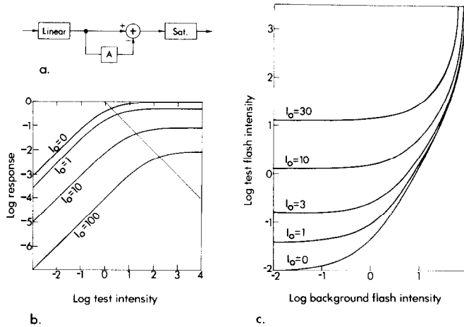
Fig. 7. (a) Subtractive adaptation model. In response to a steady input, an adapting signal is generated by the box marked "A", and this signal is subtracted from the original signal at the summing junction marked "+". (b) The effect of a steady background signal, I_0 , on the incremental response function of a system displaying I/(I + \sigma) saturation, with no adaptation. Curves (on a log-log plot) shift down and to the right at 45^\circ , due to response compression. A subtractive process can reverse the effect by reducing the size of I_0 . (c) Changes in the corresponding increment threshold curves for the same situation, assuming k = 1 , \sigma = 1 and \delta = 0.01 (see text).
