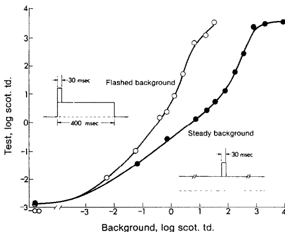
Fig. 2. Increment thresholds, using rod isolation conditions, for the flashed and steady backgrounds of Experiment 1. Open circles: 30 msec 480 nm test against red (Wratten No. 26) background flash. Solid circles: 30 msec green (Ilford No. 624) test against red (Wratten No. 26) background. With flashed backgrounds, rod saturation occurred with much less intense backgrounds than were required with the steady backgrounds. Subject E.A.
