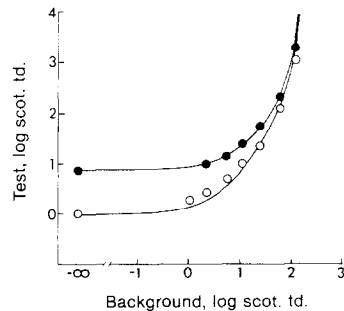
Fig. 13. The data of Fig. 10, on the time-course of pre-adaptation, fit with the subtractive model (equation 9). At t = 200 msec, I_0 = 13.1 ; at t = \infty , I_0 = 1.6 . All other parameters are the same for both curves: k = 0.284 , \sigma = 5 and \delta = 0.03 .
