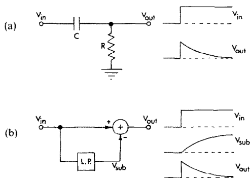
Fig. 16. (a) Simple “RC” high-pass filter, along with its step response (right). (b) The equivalent system constructed with a lowpass filter and feed-forward subtraction.
