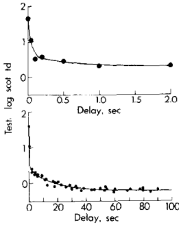
Fig. 11. Threshold for a 30 msec 480 nm test flash, presented at various times after the onset of a 0.5 log scot. td red (Wratten No. 26) field. Top and bottom show the same data, at different time scales.
