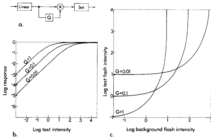
Fig. 8. (a) Multiplicative adaptation model. The adapting signal, generated at "G", multiplies the original signal by some gain between 0 and 1, at the point marked "X". (b) The effect of a gain change on the response function of a system displaying I/(I + \sigma) saturation. Curves shift to the right. (c) Changes in corresponding increment threshold functions for the same system. Curves shift up and to the right at 45^\circ , without changing shape.
