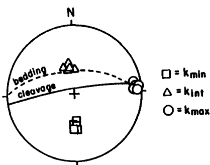
Fig. 4. Typical orientations of the principal susceptibility axes. The minimum axis is expected to be perpendicular to a planar rock fabric, such a bedding in this example. The maximum axis is commonly found at the bedding–cleavage intersection (from Borradaile, 1988).
