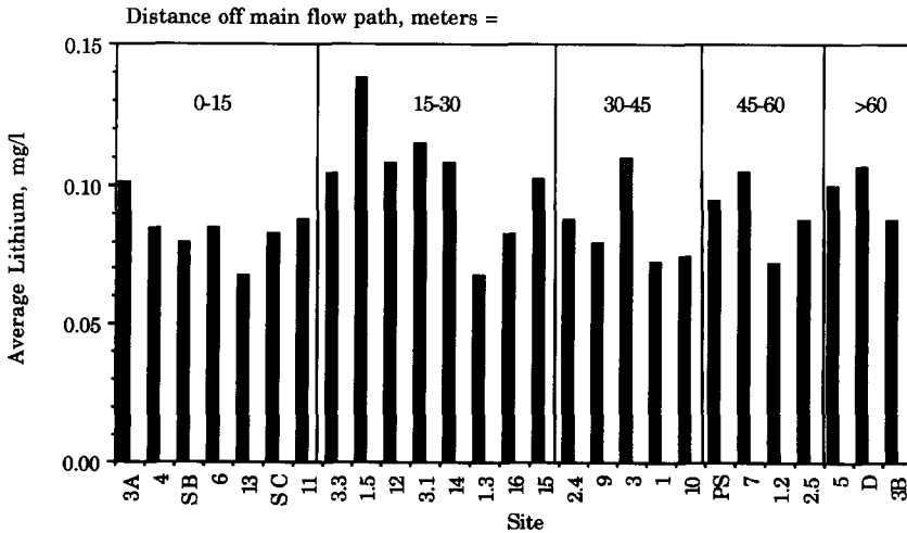
Fig. 17. Average tracer concentration at various interior wetland stations during the August, 1990 test, grouped by distance from presumed main flow path. Various distances are not different ( \alpha = 0.05 ).
