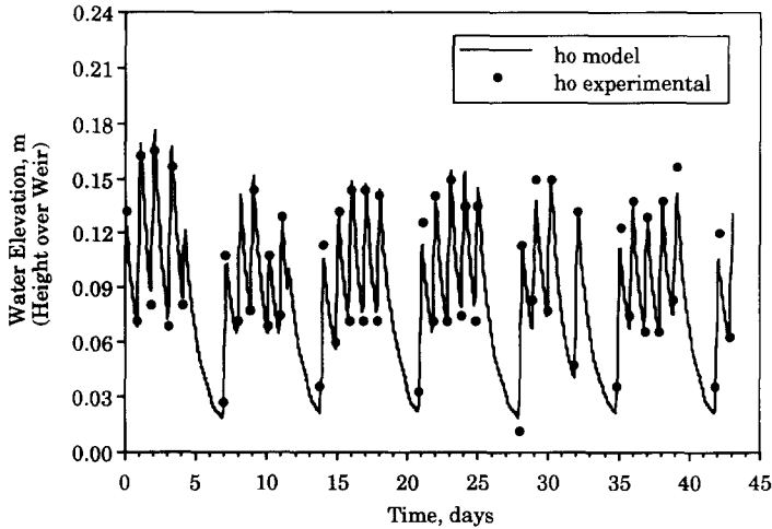
Fig. 4. Dynamic water elevations in wetland EW3 for the period June 3–July 16, 1991.
