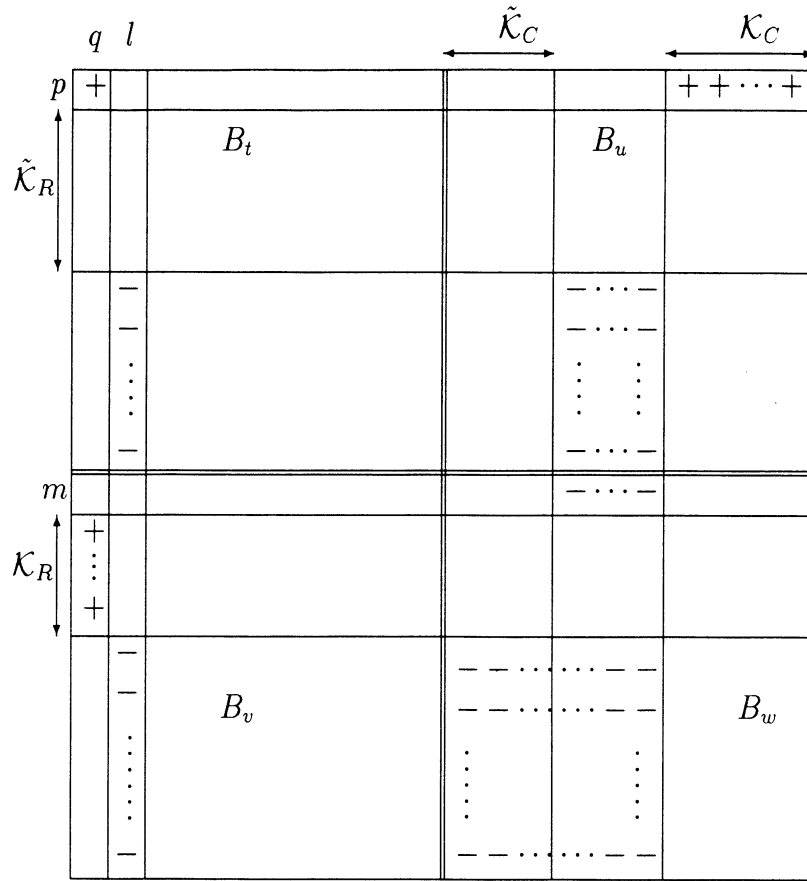
Figure 4: Pictorial representation of signs of nonzero coefficients in (15)
