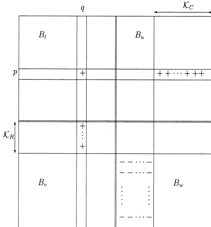
Figure 3: Pictorial representation of signs of nonzero coefficients in (12). The double lines indicate the row and column partitions.
