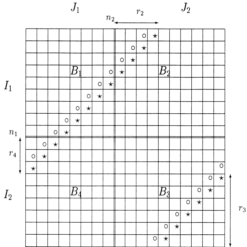
Figure 2: The double lines indicate the row and column partitions, and the four blocks B_1 , B_2 , B_3 , and B_4 are shown. The 2n basic cells corresponding to basic vector x_B are marked with (o) or (*).
