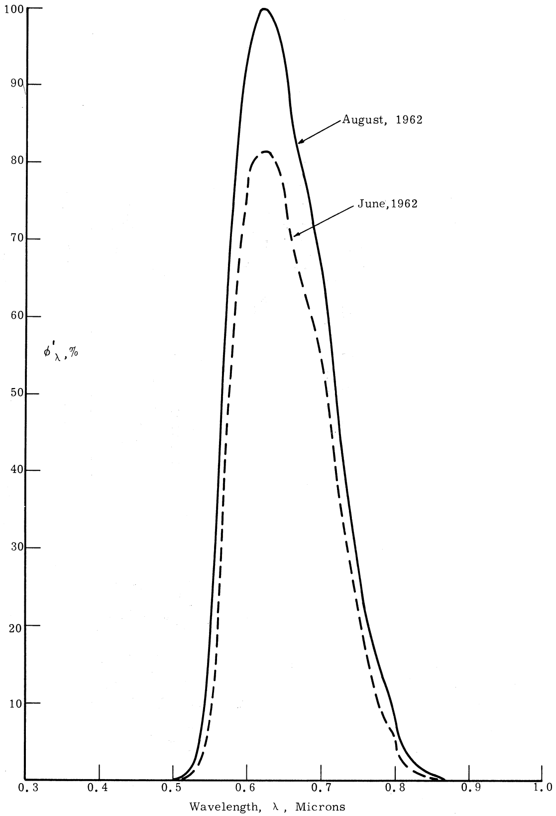
Figure 2. Relative characteristic response, \phi'_\lambda , of 0.55-0.85 micron channel of F-1 MRIR.
