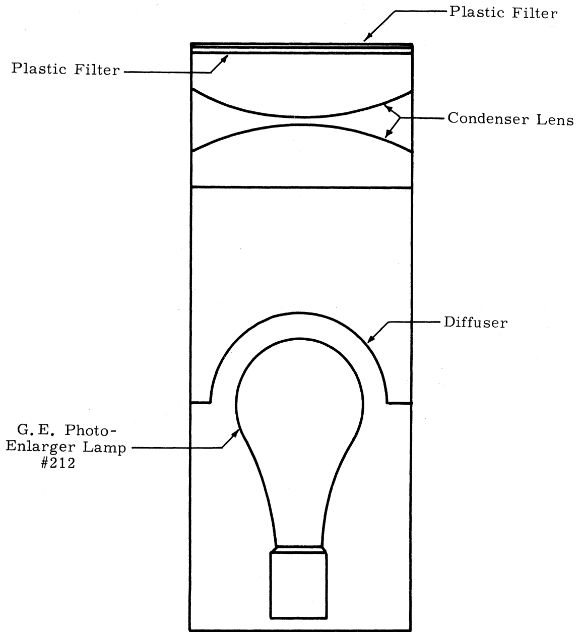
Figure 14. SBRC calibration source.
