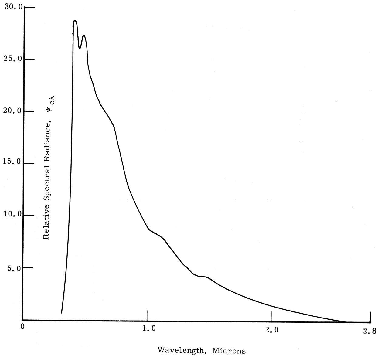
Figure 9. Relative spectral radiance of carbon arc—MgO reflector calibration source.
