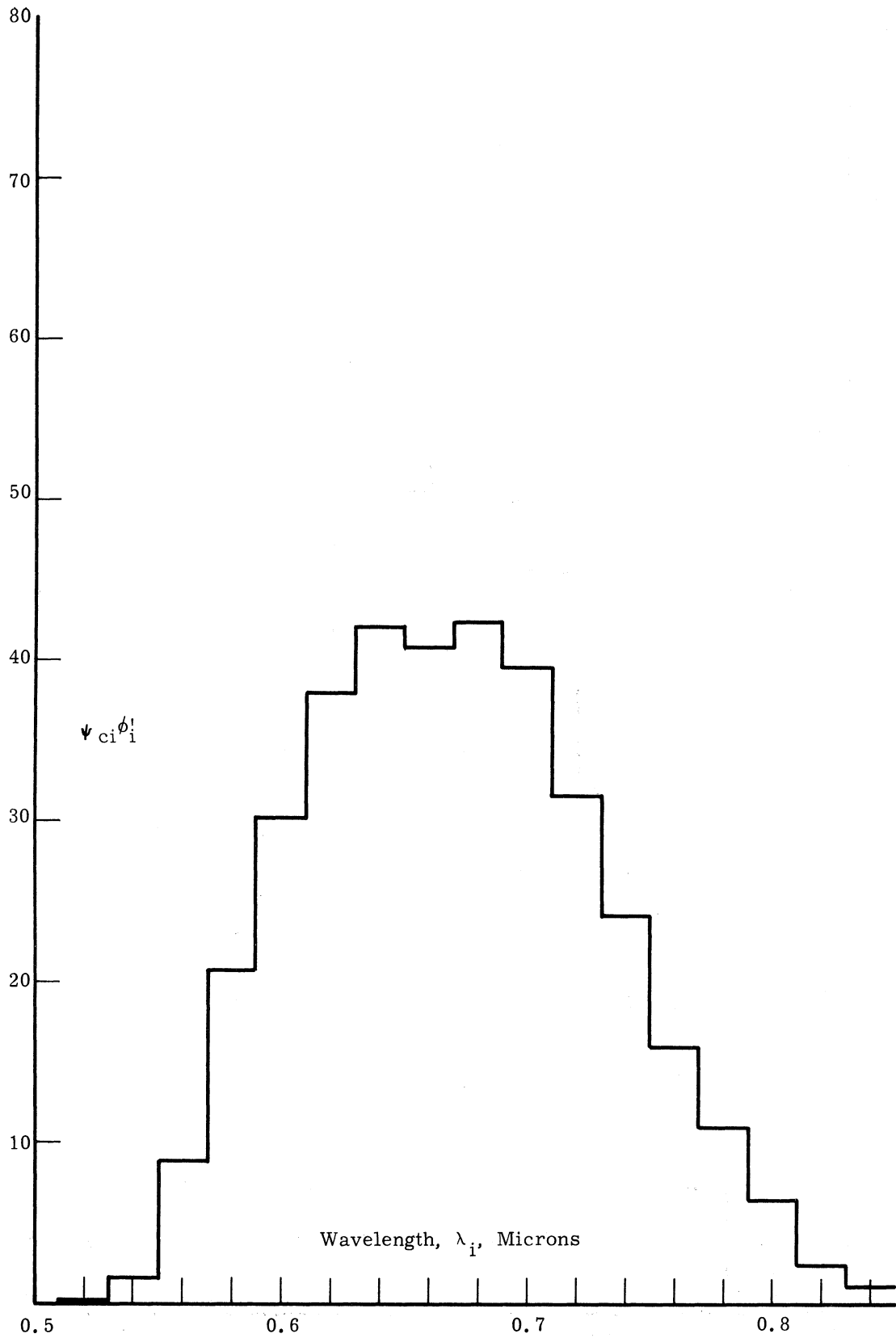
Figure 26. k_n \phi_i \psi_{ci} for lamp—MgO reflector and 0.55-0.85 micron channel of F-1 MRIR.
