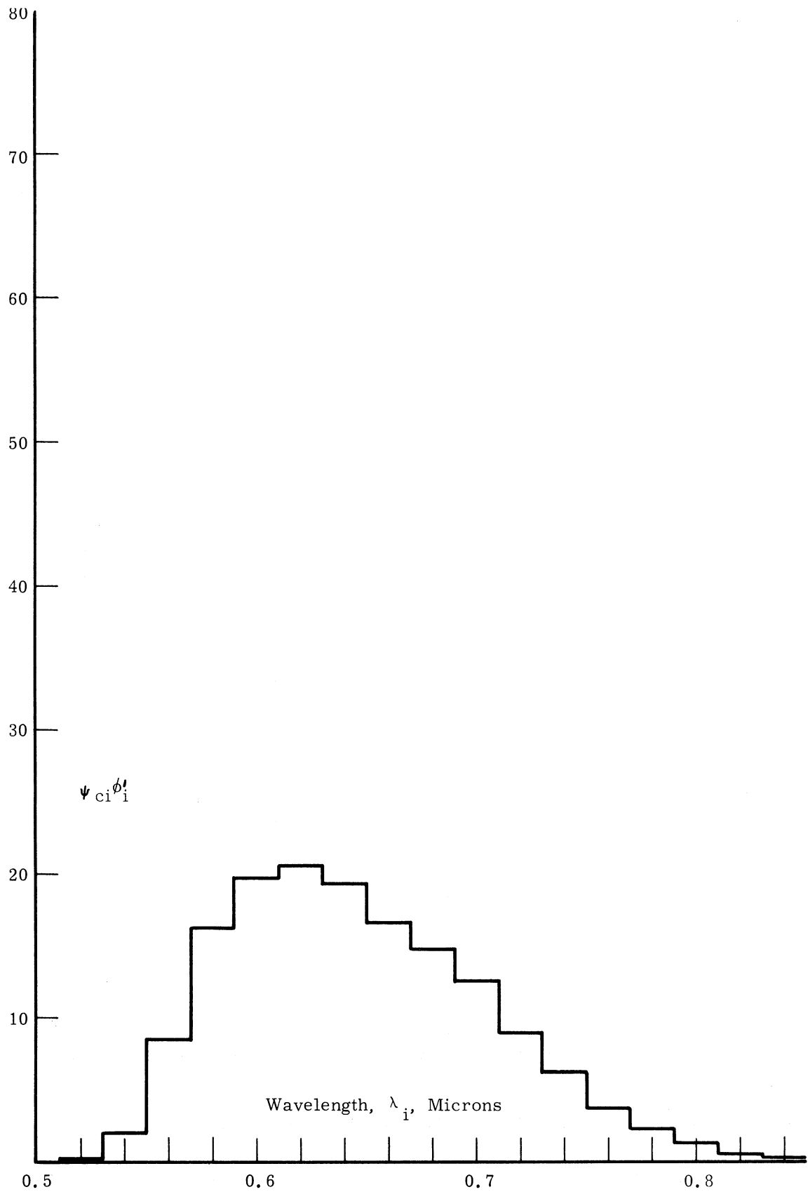
Figure 25. \phi_i \psi_{ci} for carbon arc—MgO reflector and 0.55-0.85 micron channel of F-1 MRIR.
