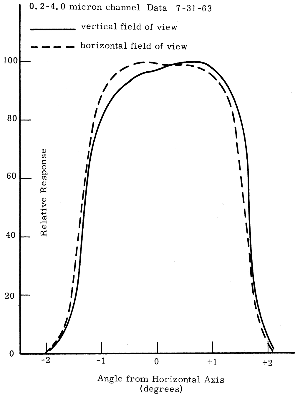
Figure 4. Field of view contours of the 0.2-4.0 micron channel of the F-4 MRIR.
