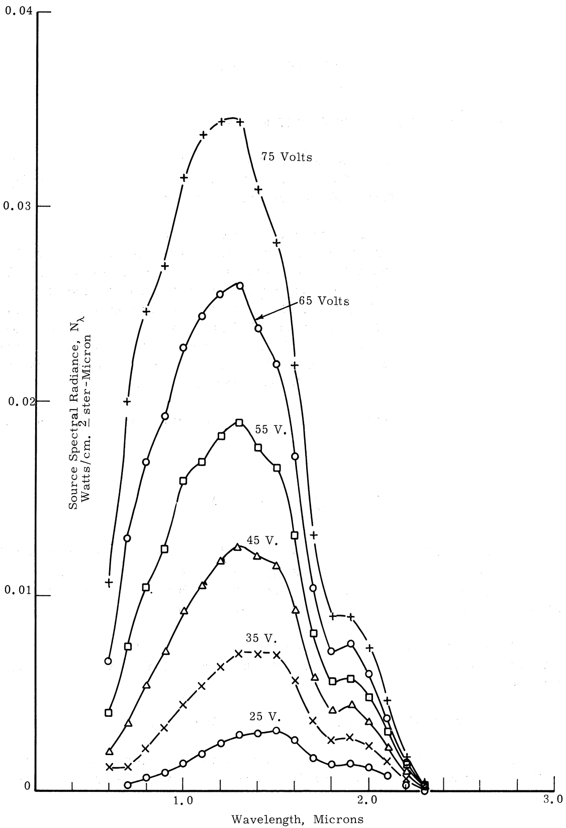
Figure 15. Spectral radiance of SBRC calibration source.
