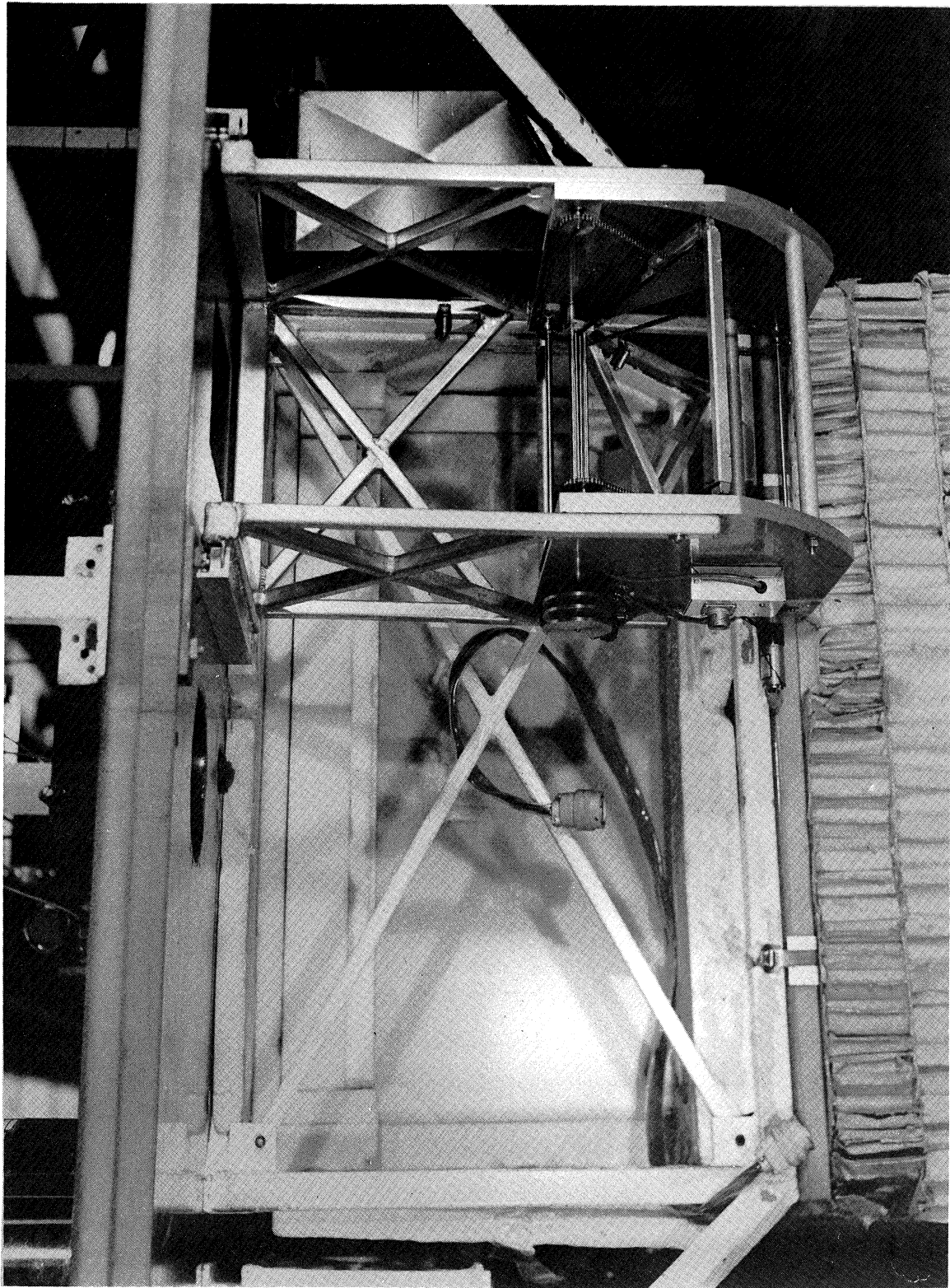
Figure 1. View Mirror for U M IRIS Interferometer
