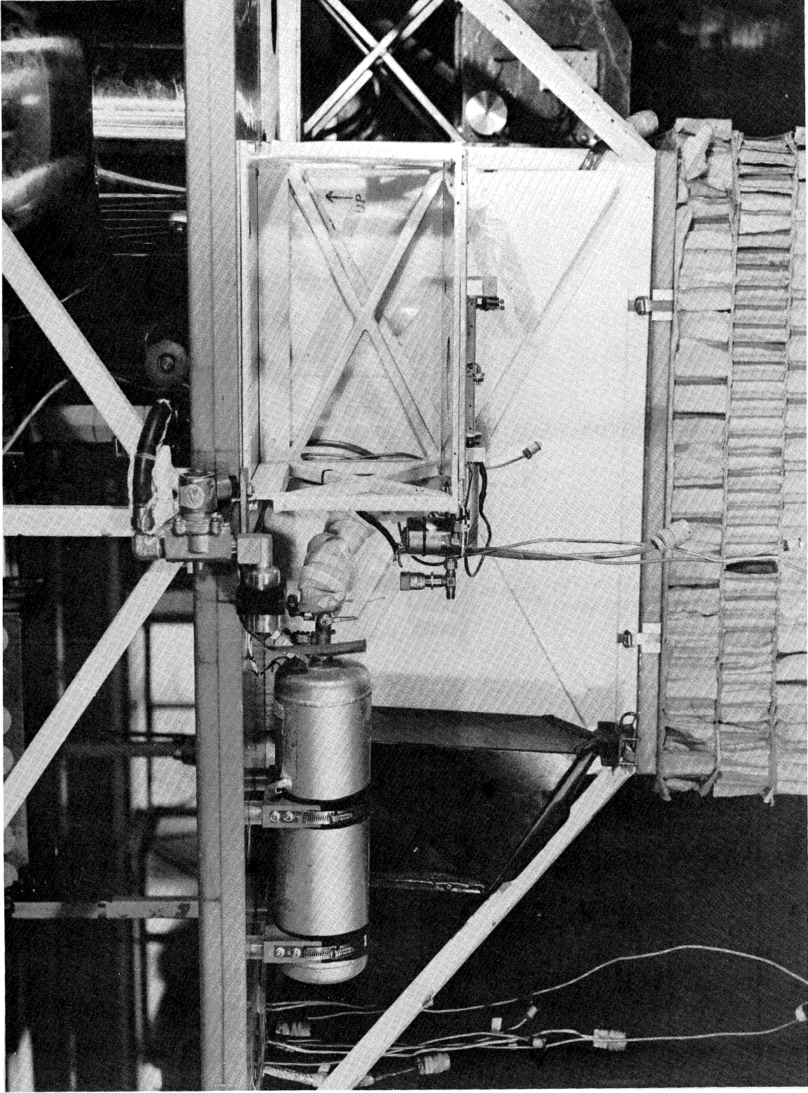
Figure 3. Filter-wedge Cooling System
