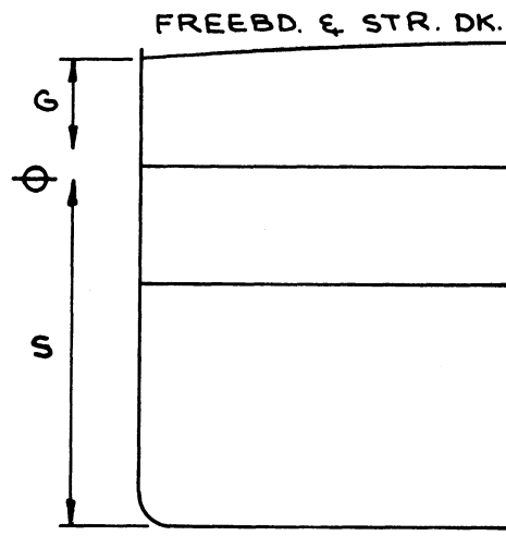
B. SCANTLING DRAFT SHIP
