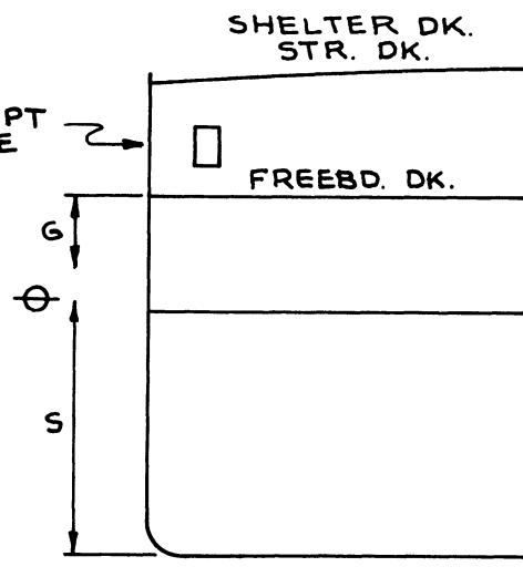
D. SHELTER DECK SHIP WITH SCANTLING DRAFT
