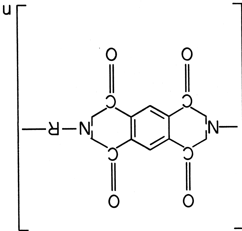
Figure 23. Polyimide
