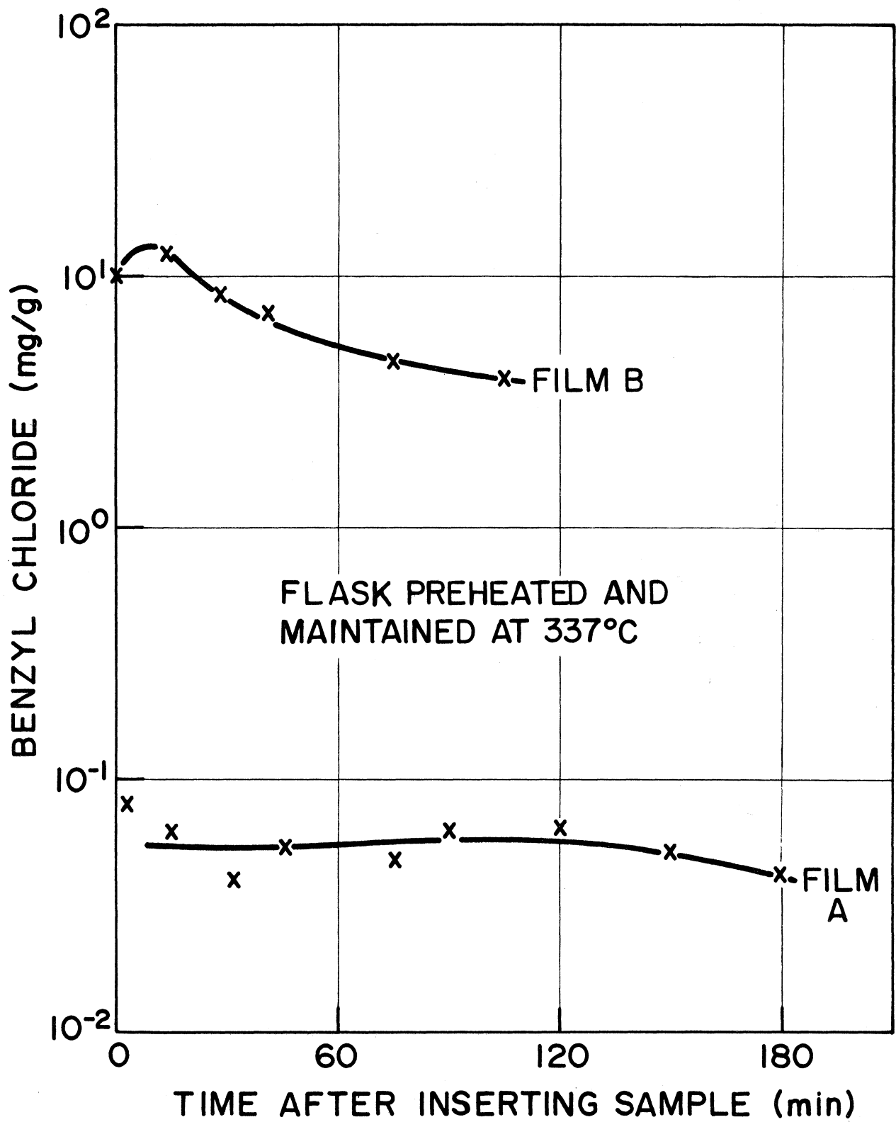
Figure 14. Benzyl chloride production by two meat-wrap films (A and B) heated at 337 C
