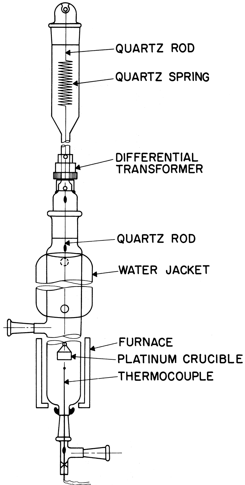
Figure 2. Schematic diagram of a thermogravimetric analysis (TGA) apparatus
