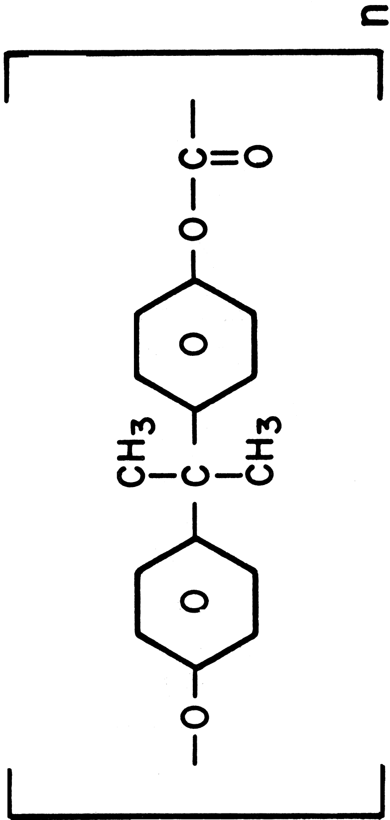
Figure 42. Bisphenol A-polycarbonate
