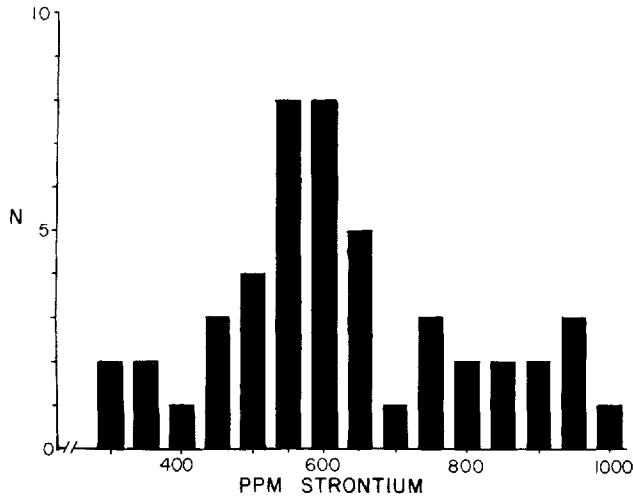
Fig. 2 Distribution of bone strontium levels in adults from Phase C Middle Formative period at Chalcatzingo. The samples were analyzed as dissolved bone ash by atomic absorption spectrometry (N=47, \bar{X} =627, SD=175, V=28).
