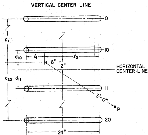
Fig. 4. Dimensions for Example Calculation of Radiation Field
