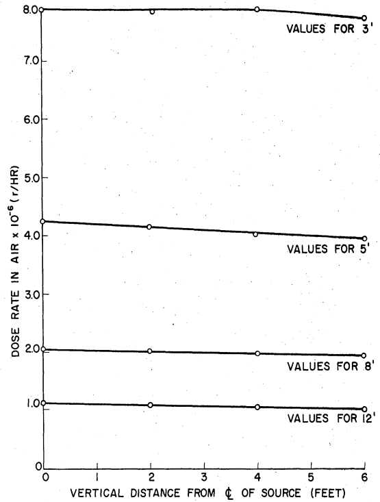
Fig. 5. Radiation Flux Versus Vertical Distance for Selectively Spaced Fuel Elements
