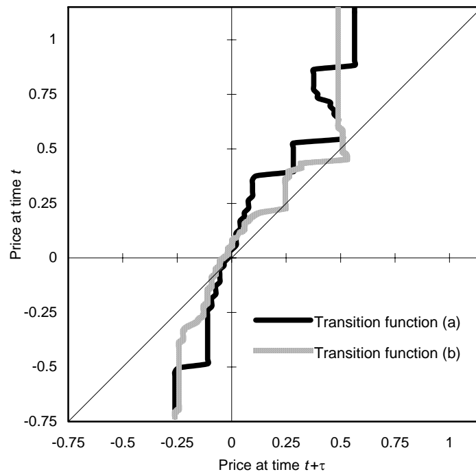
Figure 5. Mode lines of the transition probability functions
