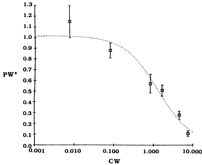
Fig. 2. Transport kinetics of N -benzoylproline. PW* is the dimensionless membrane permeability, and CW the membrane surface concentration (mM). The values of PW* shown are mean \pm SE. (Adapted from Ref. 24.)
