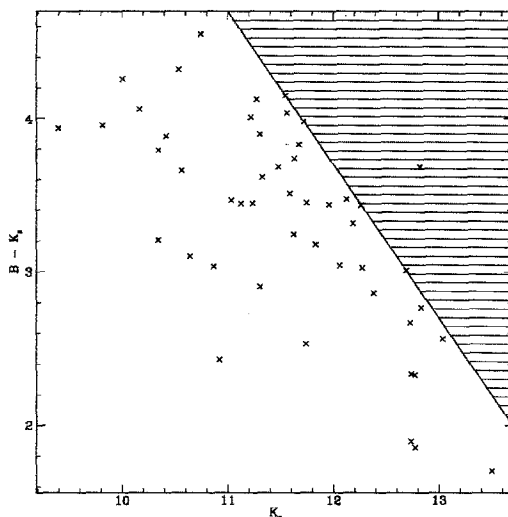
Fig. 4. The color-magnitude diagram ( B - K_s vs. K_s ) for galaxies in an 11 sq. deg. field near l=135^\circ , b=-25^\circ . The shaded region corresponds to the limit of the Zwicky catalog, B \sim 15.7 mag. Only the bluest of the faint galaxies are found in both the Zwicky and 2MASS samples.
