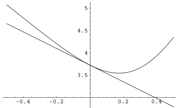
Fig. 5. The graph of y = L(P_X) and its tangent line y = -\varepsilon(6, 1, X) .
