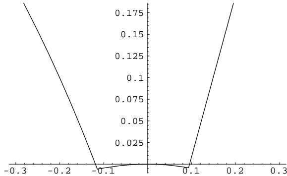
Fig. 8. The graph of \tilde{L}(6, 1, X) + \varepsilon(6, 1, X) .
