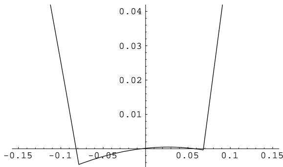
Fig. 9. The graph of \tilde{L}(7, 1, X) + \varepsilon(7, 1, X) .
