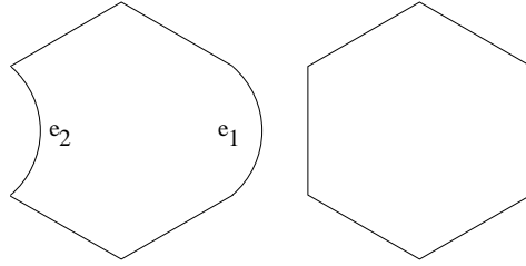
Fig. 6. A deformation reducing the perimeter at fixed area.
