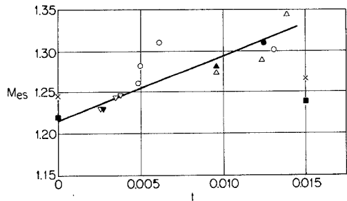
Figure 4 Effect of curvature parameter, t , on Mach number for incipient separation, M_{es} , from Reference [20]. Triangles and circles correspond to different airfoils. Present calculations shown as follows: at t = 0 , (■) Re = 10^6 , \Pi = 0.5 , K = 0 ; (×) Re = 10^7 , \Pi = 0.5 , K = 0 . At t = 0.015 , (■) Re = 10^6 , \Pi = 0 , K = 0.21 ; (×) Re = 10^7 , \Pi = 0 , K = 0.28 .
