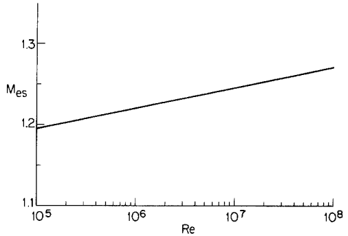
Figure 3 M_{es} (Mach number at incipient separation) vs. Re for flow over a flat plate, calculated using Eqn. (27a) with (\tau_w)_{min} = 0 , \Pi = 0.5 , K = 0 .
