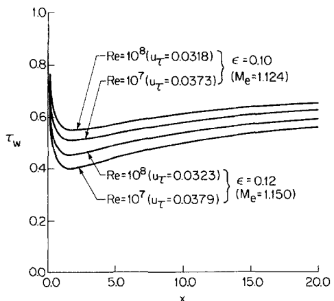
Figure 1 \tau_w vs. x for various values of M_e and Re , for flow over a flat plate. (Eqn. (27a) with \Pi = 0.5 , K = 0 ).
