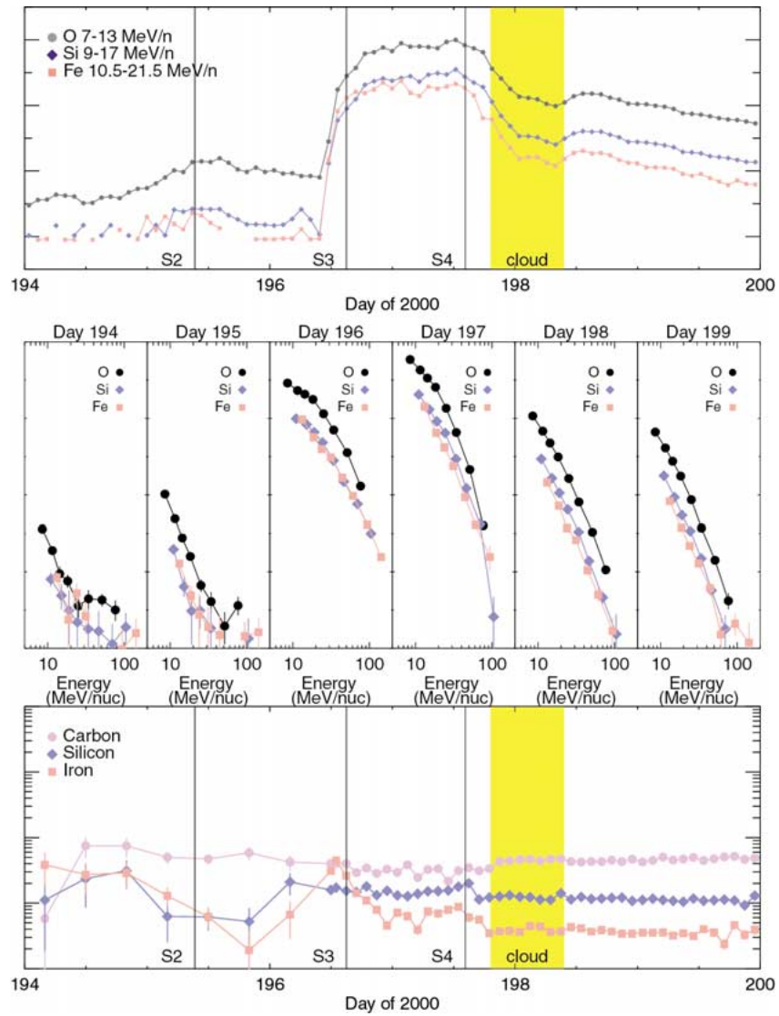
Figure 7. SIS intensity time profiles for O, Si, and Fe ( top panel ); daily averaged elemental spectra for O, Si and Fe ( middle panel ); and abundances relative to O over 12 to 60 MeV \text{nuc}^{-1} for C, Si, and Fe using 8-h and 2-h averages ( bottom panel ). Typical gradual SEP abundances for these elements are given along the right-hand side of the plot. In the top and bottom panels, vertical lines denote identified shocks and a yellow shaded region indicates the passage of Cloud4.
